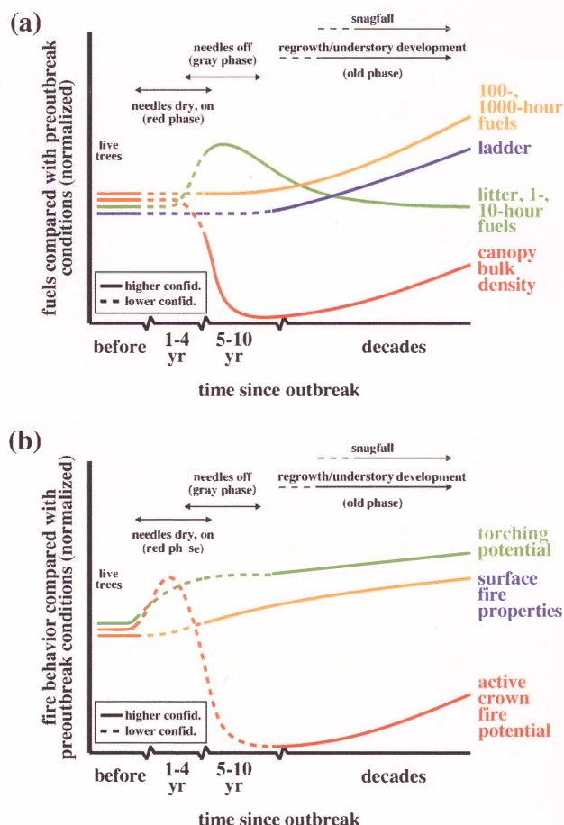
Fig. 2. Conceptual framework of (a) fuels characteristics and (b) fire behavior relative to preoutbreak conditions for red, gray, and old (snagfall and regrowth) phases. Surface fire properties include reaction intensity, rate of spread, and flame length. For postoutbreak phases, solid lines indicate higher confidence in responses based on Fig. 3, and dashed lines indicate lower confidence (more disagreement, fewer studies, or knowledge gaps).
