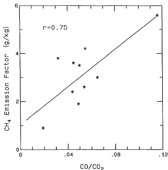
Figure 28.12 \text{CH}_4 emission factor versus the ratio of CO to \text{CO}_2 emission factors for ten of the seventeen fires studied. r is the correlation coefficient, and the line shown is a linear regression. Data is taken from Table 28.4.
