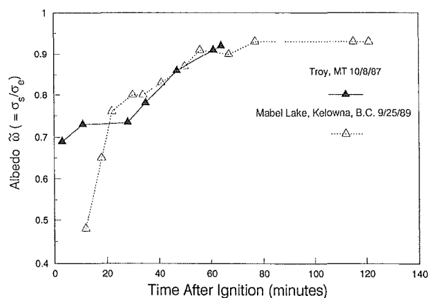
Figure 28.8 The time evolution of the single-scattering albedo \bar{\omega} for smoke from the Troy (solid triangles) and Mabel Lake (hollow triangles) prescribed burns.
