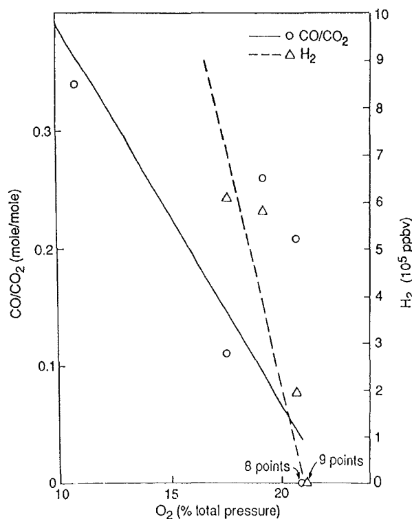
Figure 28.11 Concentration ratio of CO/CO 2 (circles) and H 2 concentration (triangles) versus O 2 in the plume from the Battersby fire. The data were obtained at or within 100 m of the ground. The lines shown are linear regressions (from Hegg et al., 1990).
