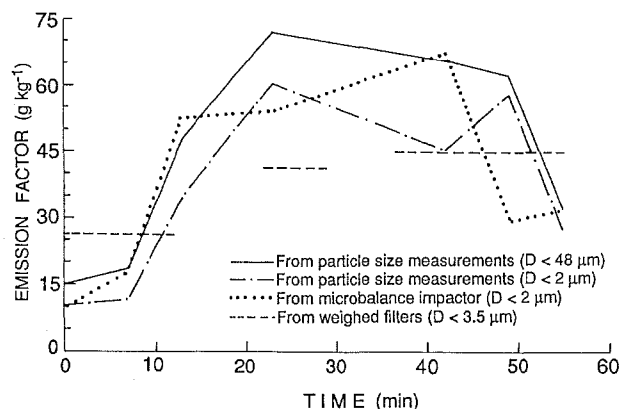
Figure 28.2 Emission factors for particle mass as a function of time from the beginning of observations on the Abec fire. A vigorous cumulus cloud capped the smoke column for the first 10 to 15 min. The measurements were made downwind of this capping cumulus in the stabilized plume of smoke (from Radke et al., 1988).
