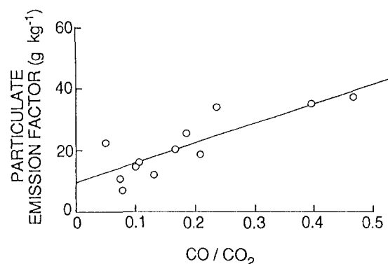
Figure 28.4 Emission factors for particles as a function of the \text{CO}/\text{CO}_2 concentration ratio in the plume from the Battersby fire. The \text{CO}/\text{CO}_2 ratio is a measure of the extent of oxidation in the plume, with higher values indicating less oxidation (from Hegg et al., 1990).
