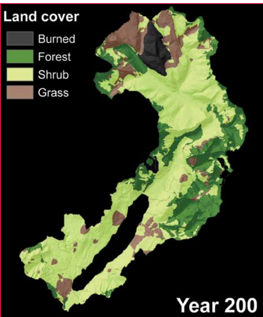
Figure 5—In a watershed dominated by forest in 2009, FIREBGCv2 predicts shrubs will dominate after 200 years of influence from changed climate and wildfire. Source: Rachel Loehman, Missoula Fire Sciences Laboratory.
