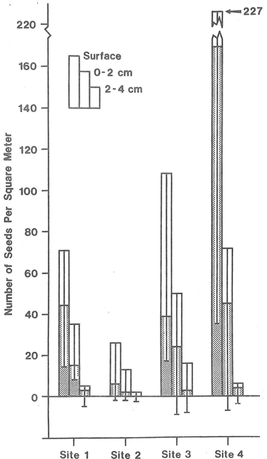
Figure 2 —The average number of mamane seeds per m 2 was greater on the soil surface than within the soil at depths of 0- to 2-cm and 2- to 4-cm at four sites on Mauna Kea. Vertical bars represent one-half of one standard deviation. Shaded portions denote the number of seeds that germinated in the laboratory.
