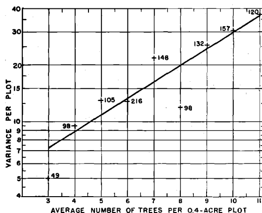
Fig. 3.—Relationship of variance per plot to average number of trees per plot.
