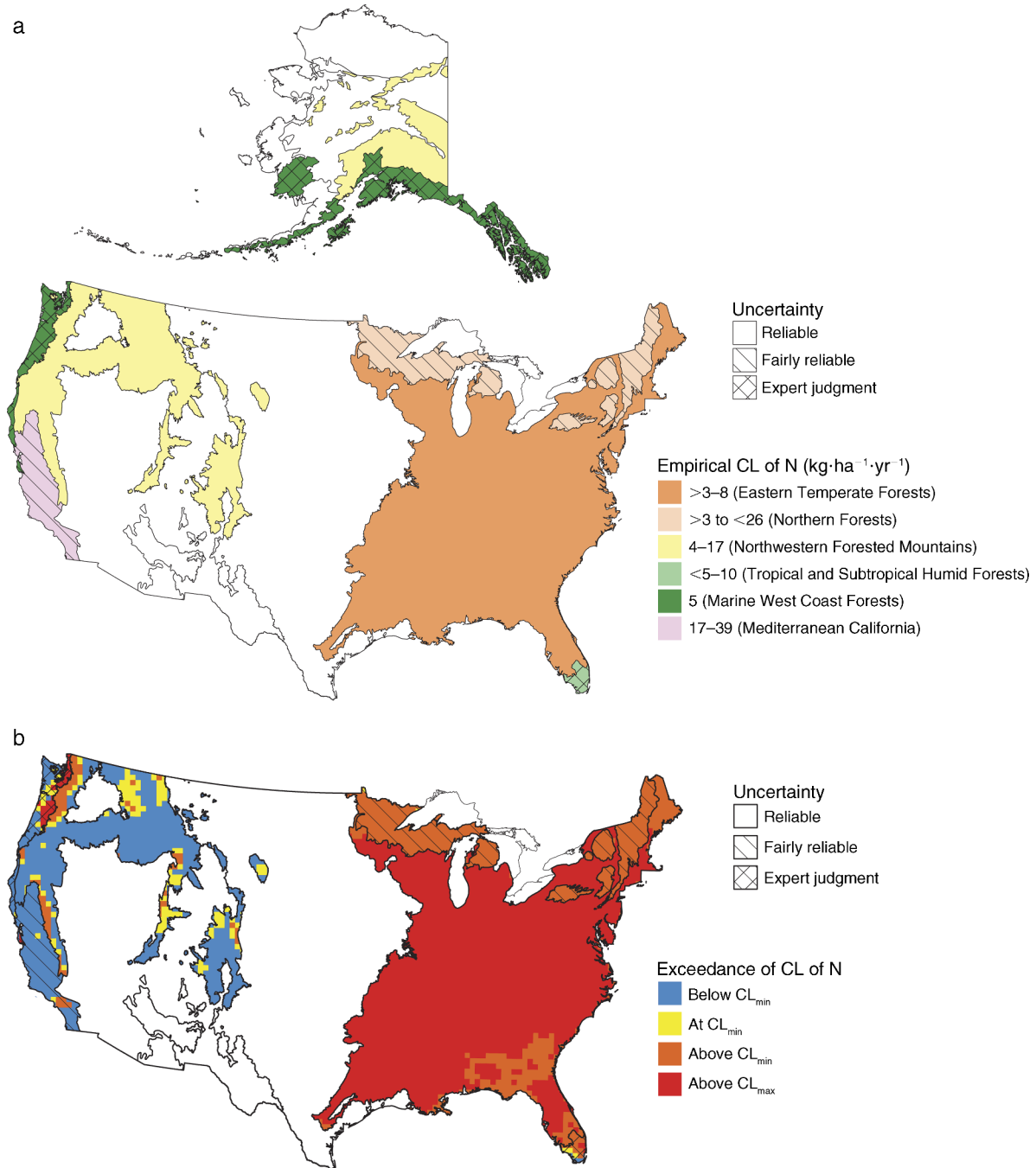
FIG. 6. Map of (a) critical loads and (b) exceedances of N for forest ecosystems by ecoregion in the United States. (a) The range of critical loads reported for forest ecosystems is shown for each ecoregion; this map does not include the responses of mycorrhizal fungi, lichens, or understory herbaceous plants already represented. The hatch marks indicate increasing level of uncertainty: no hatch marks for the most certain “reliable” category, single hatching for the “fairly reliable” category, and cross-hatching for the “expert judgment” category. The color sequence moves from red toward blue and violet as the critical load increases. As the range of the critical load gets broader, the saturation of the color decreases. (b) Exceedance (critical load – deposition) is shown for several categories: (1) no exceedance (below \text{CL}_{\min} ), when deposition is lower than the CL range, (2) at \text{CL}_{\min} , when deposition is within \pm 1 of the CL range, (3) above \text{CL}_{\min} , when deposition is above the lower end of the CL range, but lower than the upper end of the range, (4) above \text{CL}_{\max} , when deposition is above the upper end of the CL range. CMAQ deposition data were not available for Alaska, so we were not able to calculate exceedance for Alaska.
