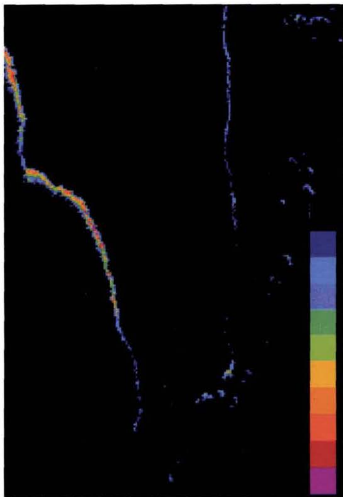
Plate 3. An active prescribed fire in the campo limpo (clean grassland) phase of the Cerrado at the Reserva Ecológica of the Instituto Brasileiro de Geographia e Estatística, Distrito Federal, Brazil, as measured by the Fire Imaging Spectrometer. This density-sliced image depicts the wavelength-integrated fire radiance computed as (A\sigma/\pi)T^4 (see text). The color bar depicts increasing radiance from dark blue to magenta in increments of 625 \text{ (J m}^{-2} \text{ s}^{-1} \text{ sr}^{-1}) . The fire was ignited along a gallery forest at the far right and a roadway to the left of the combustion. Apparent fire-line widths are in scale and show variations in burning conditions. More intense portions of the fire line on the left are propagating with the wind; the line on the right (in blue) is nearly stationary and parallel to the ambient wind field. Detached areas of fire at the far right are largely residual combustion in woody material or ground fuels along the margin of the gallery forest.
