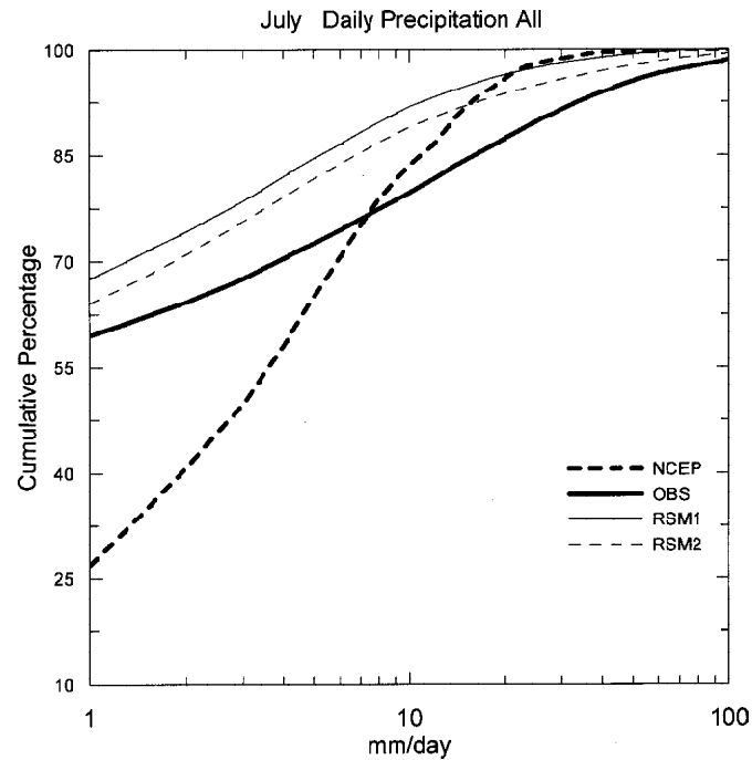
Fig. 12. Same as Fig. 10, except for July.
