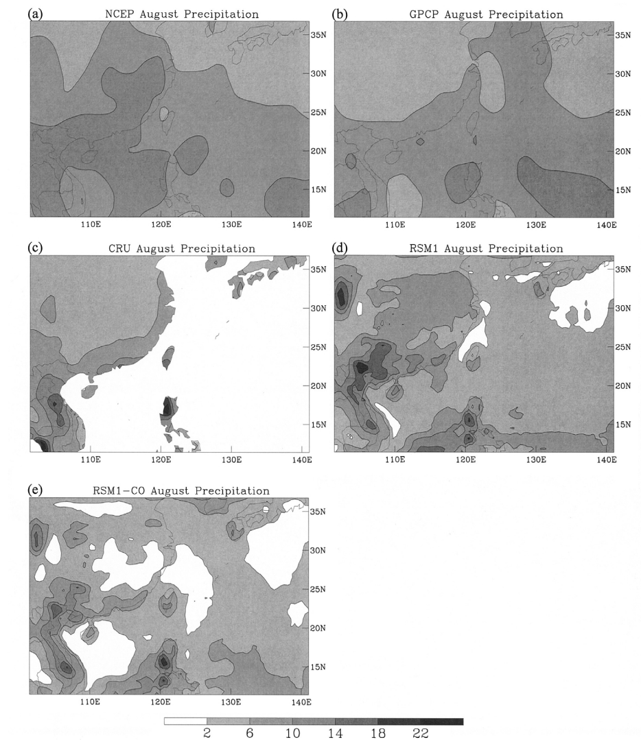
Fig. 7. Same as Fig. 5, except for August.
