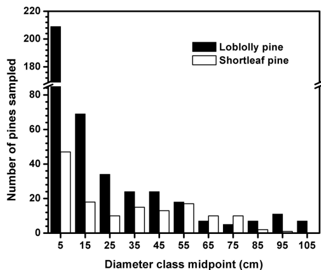
Figure 1. Diameter class distribution of loblolly and shortleaf pines selected for height-diameter model fitting.
