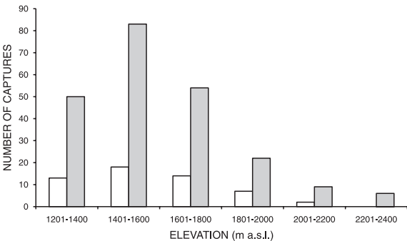
Figure 2. Elevations of fisher captures in live (□) and camera traps (■) in the Sierra National Forest, Fresno County, California, USA. Data are combined for surveys conducted from 2002 to 2004.
