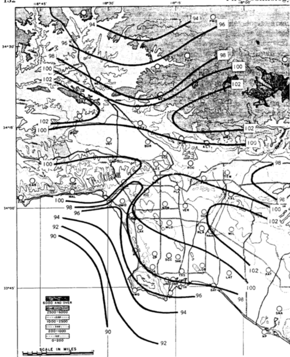
Figure 2. Thermal structure during late afternoon on November 1.
