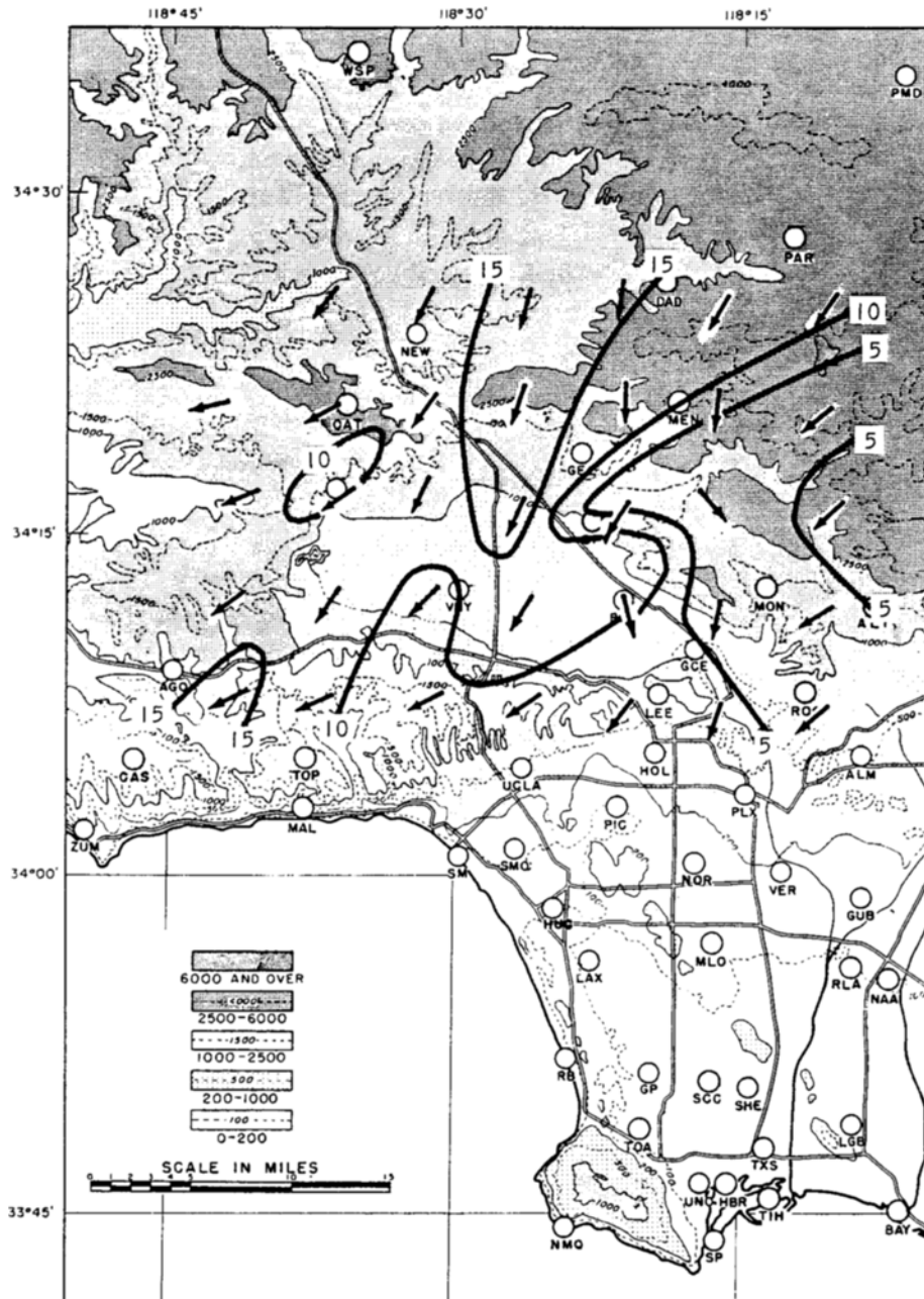
Figure 3. Wind field during late afternoon on November 1.
