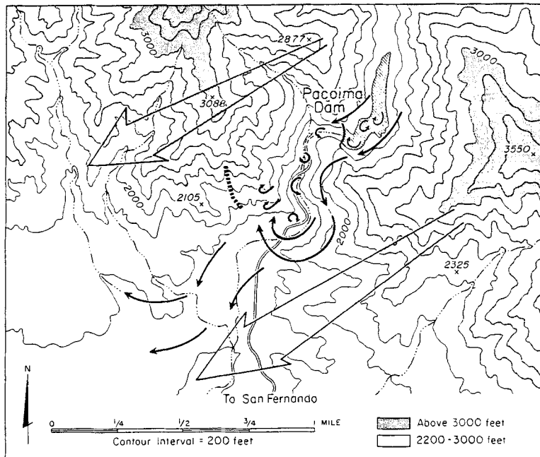
Figure 8. Air flow in the vicinity of Pacoima Canyon during the afternoon of November 1.
