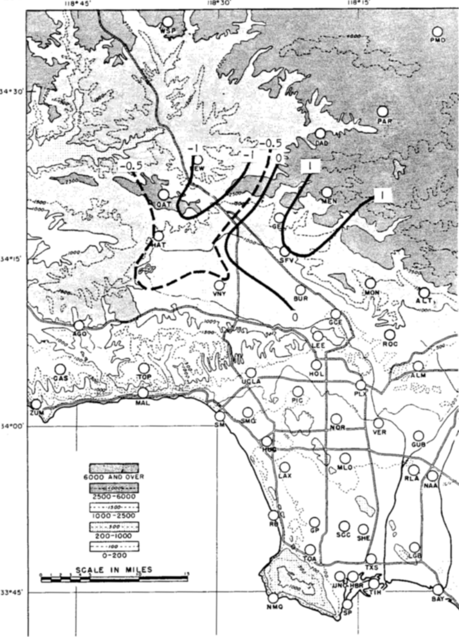
Figure 4. Vorticity field during late afternoon on November 1.
