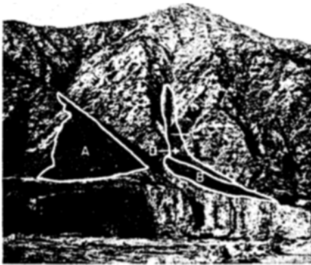
Figure 9. Pacoima Canyon area showing sections involved in fire (A, B, and C) and the site of the tragedy (D).
