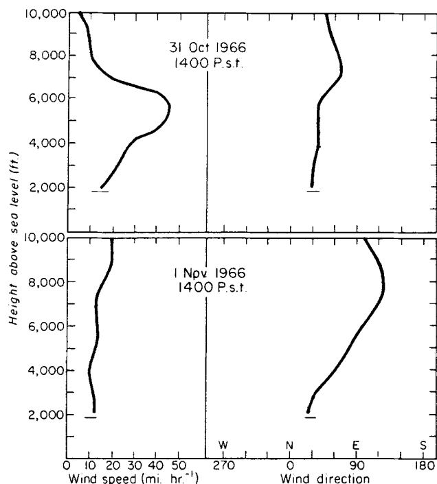
Figure 7. Rocketdyne wind profiles for October 31 and November 1.
