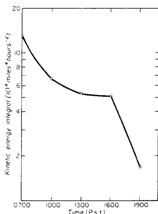
Figure 5. Kinetic energy integral for a 12-hour period on November 1.
