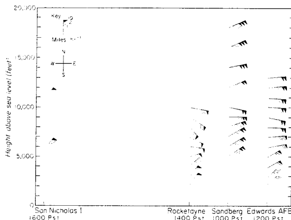
Figure 6. Wind velocity data.
