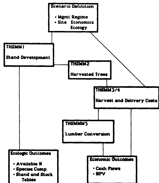
Figure 1. General structure of the tug Hill model (THSMM). The important components are numbered 1-5 and were once stand alone computer models.
