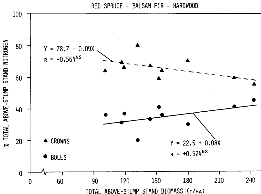
Figure 3. Relationship between total above-stump stand biomass and the proportion of total stand nitrogen contained in crowns and boles for red spruce-balsam fir-hardwood stands (data from Table 1). The correlation coefficients are not significant (NS) at \alpha = 0.05 .
