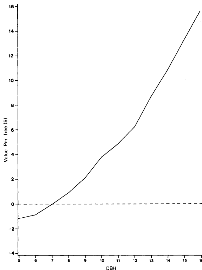
Figure 2. Graph of value per tree as diameter increases. This graph shows that trees below 7 inches DBH had negative value in our scenario; in other words they did not "pay their way out of the woods".
