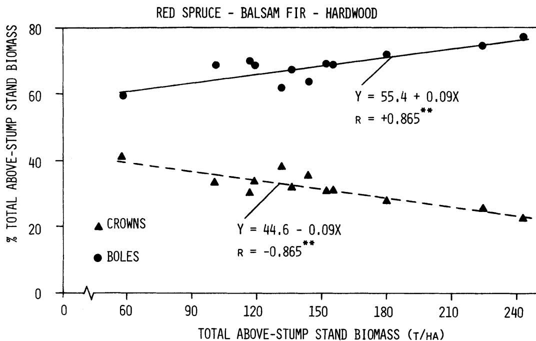
Figure 1. Relationship between total above-stump stand biomass and the proportion of that biomass contained in crowns and boles for red spruce-balsam fir-hardwood stands (data from Table 1). The correlation coefficients are highly (**) significant ( \alpha = 0.01 ).
