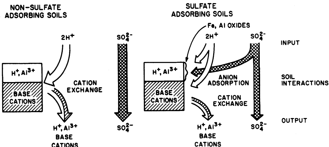
Figure 2. Schematic representation of effects of SO_4^{2-} adsorption on soil leaching by H_2SO_4 . Soil at left does not absorb SO_4^{2-} and therefore cation leaching equals H^+ input. Soil at right absorbs SO_4^{2-} , and charge balance requires an equivalent reduction in potential cation leaching.
