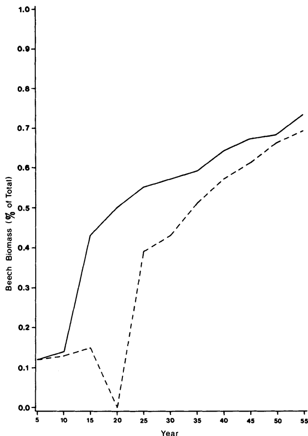
Figure 6. Graph of percent biomass which is beech by year. The solid line is from the 7 inch minimum diameter harvest and the dashed line is from the harvest which includes all trees. The rotation lengths are those optimal for a 4% interest rate given the type of harvest described.
