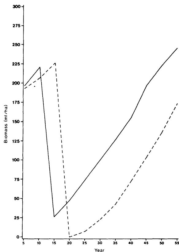
Figure 5. Graph of biomass (metric tons) per hectare by year. The solid line is the 7 inch minimum diameter harvest and the dashed line is the harvest which includes all trees. The rotation lengths are those optimal for a 4% interest rate given the type of harvest described.
