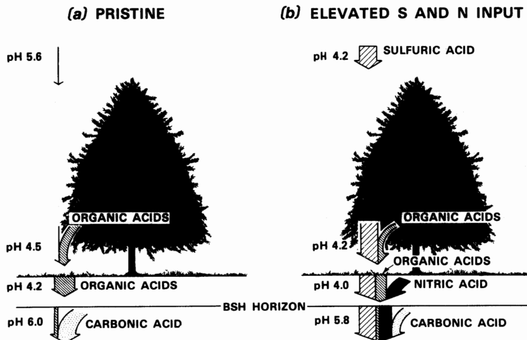
Figure 1. Schematic representation of leaching by organic and carbonic acids in (a) unpolluted and (b) polluted northern/subalpine forests.
