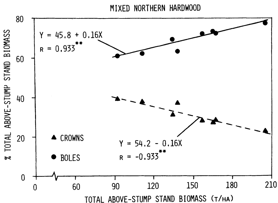
Figure 2. Relationship between total above-stump stand biomass and the proportion of that biomass contained in crowns and boles for mixed northern hardwood stands (data from Table 1). The correlation coefficients are highly (**) significant ( \alpha = 0.01 ).
