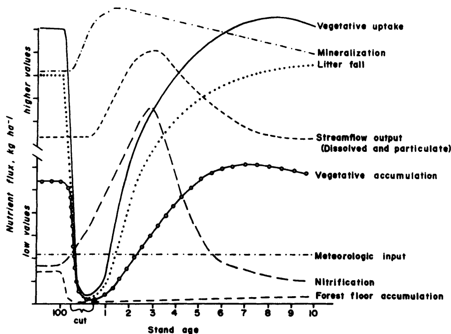
Figure 1.--Hypothetical curves of changes in fluxes of nitrogen.
