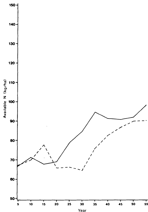
Figure 4. Graph of available nitrogen per hectare by year. The solid line is the 7 inch minimum diameter harvest and the dashed line is the harvest which includes all trees. The rotation lengths are those optimal for a 4% interest rate given the type of harvest described.
