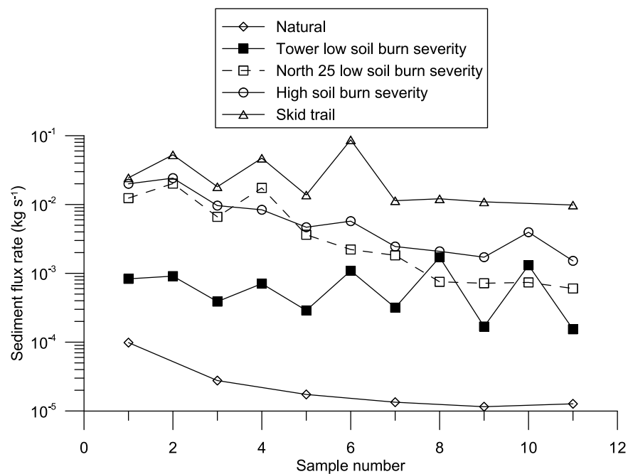
Figure 3. Mean sediment flux rate verses sample for each treatment.
