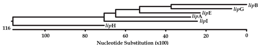
Fig. 2. Cladistic analysis of 1 Kb of six lip promoters corresponding to the Subfamily I classification from Phanerochaete chrysosporium . Each sequence in the analysis corresponds to 1 Kb upstream of the ATG codon. Analysis was done with the ClustalW (Thompson et al., 1994) algorithm on DNASTar software.
