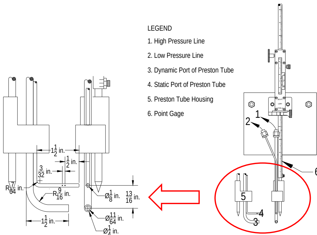
Figure 3.5: Preston Tube Schematic (Sclafani 2008)
