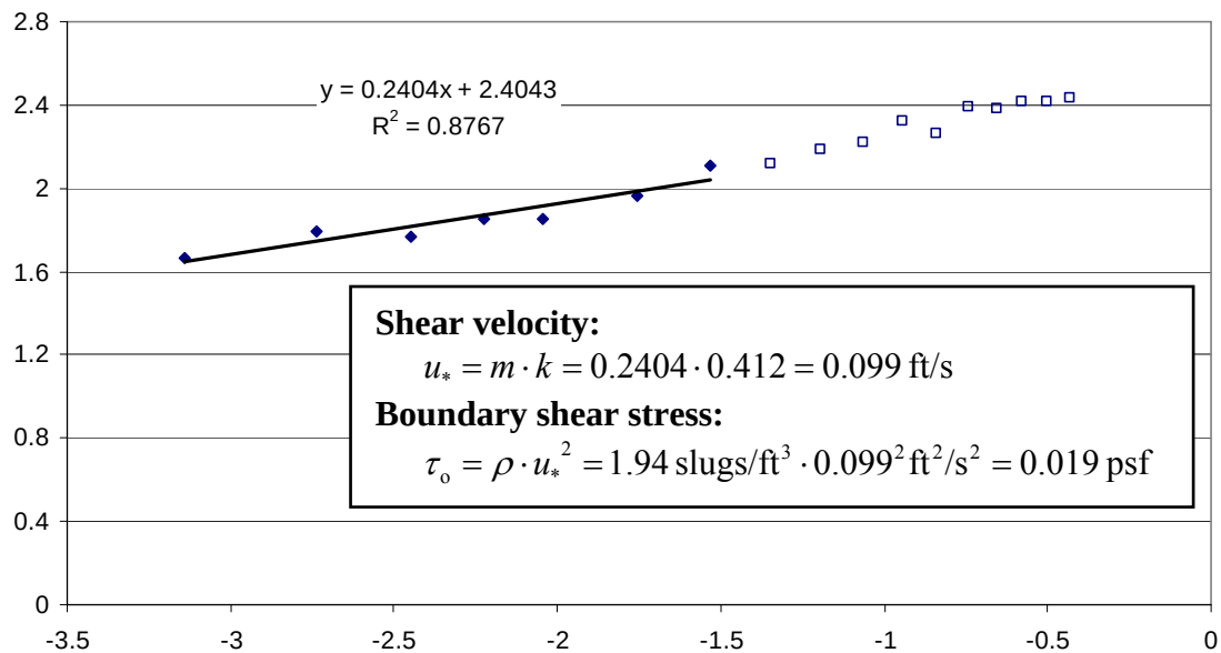
Figure 5.12: Regression of Logarithmic Profile for 16 cfs at Cross Section 14, Location c
