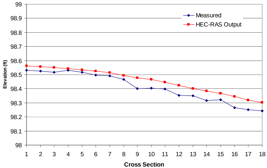
Figure 5.3: Energy Grade Line Comparison for 12 cfs
