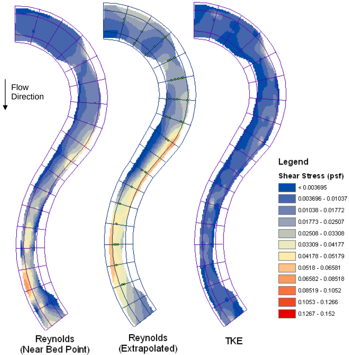
Figure 6.8: Comparisons between Reynolds and TKE Methods (12 cfs)
