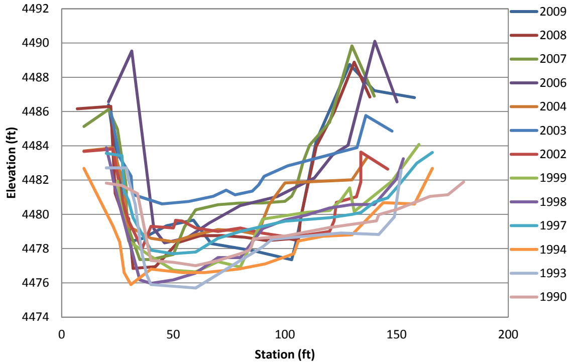
Figure F.5 SO-1683 Cross-Section
