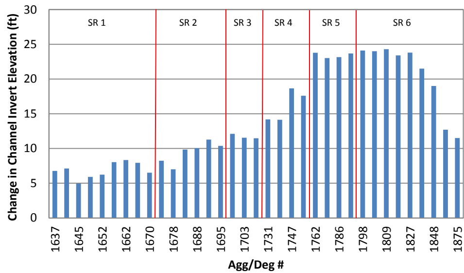
Figure 4.18 Change in Channel Thalweg Elevation from 1962 – 2002 Based on Agg/Deg Surveys
