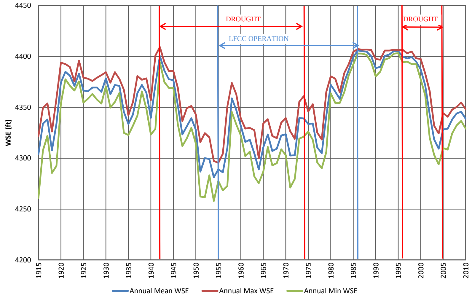
Figure 3.1 Elephant Butte Reservoir Level Time Series
