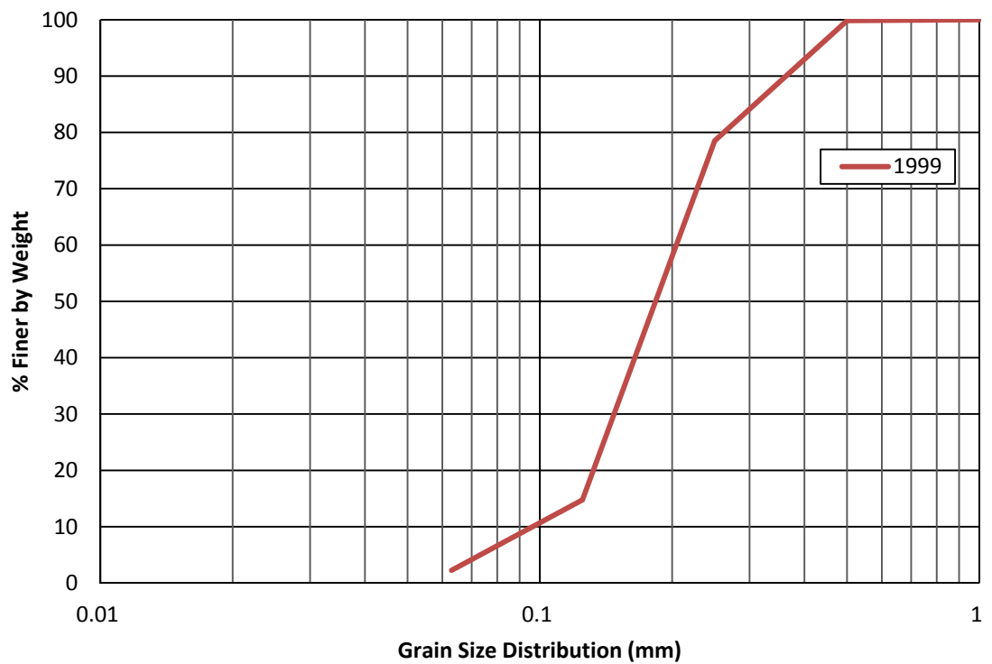
Figure 4.59 Subreach 2 (SO-1683): Annual Bed Material Grain Size Distributions
