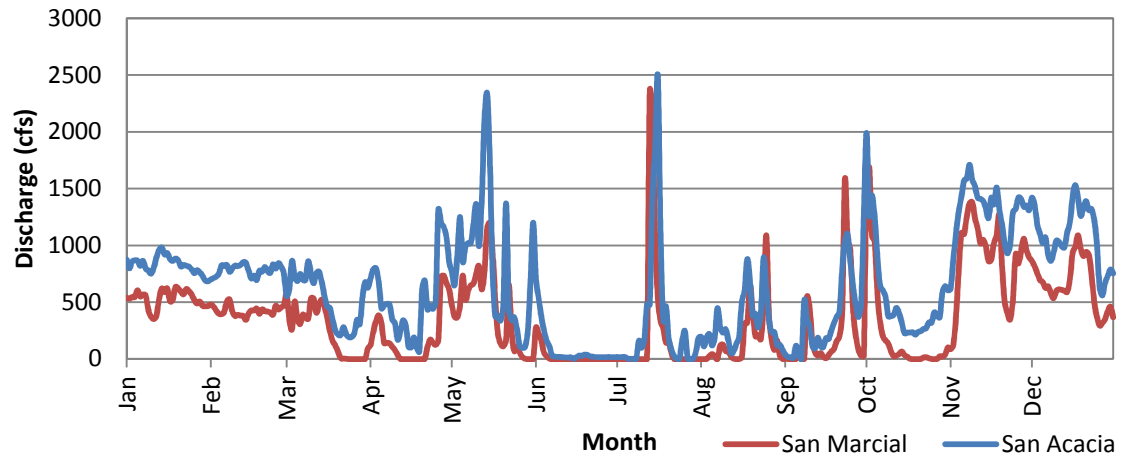
Figure B.1 1990 Daily Discharge Data
