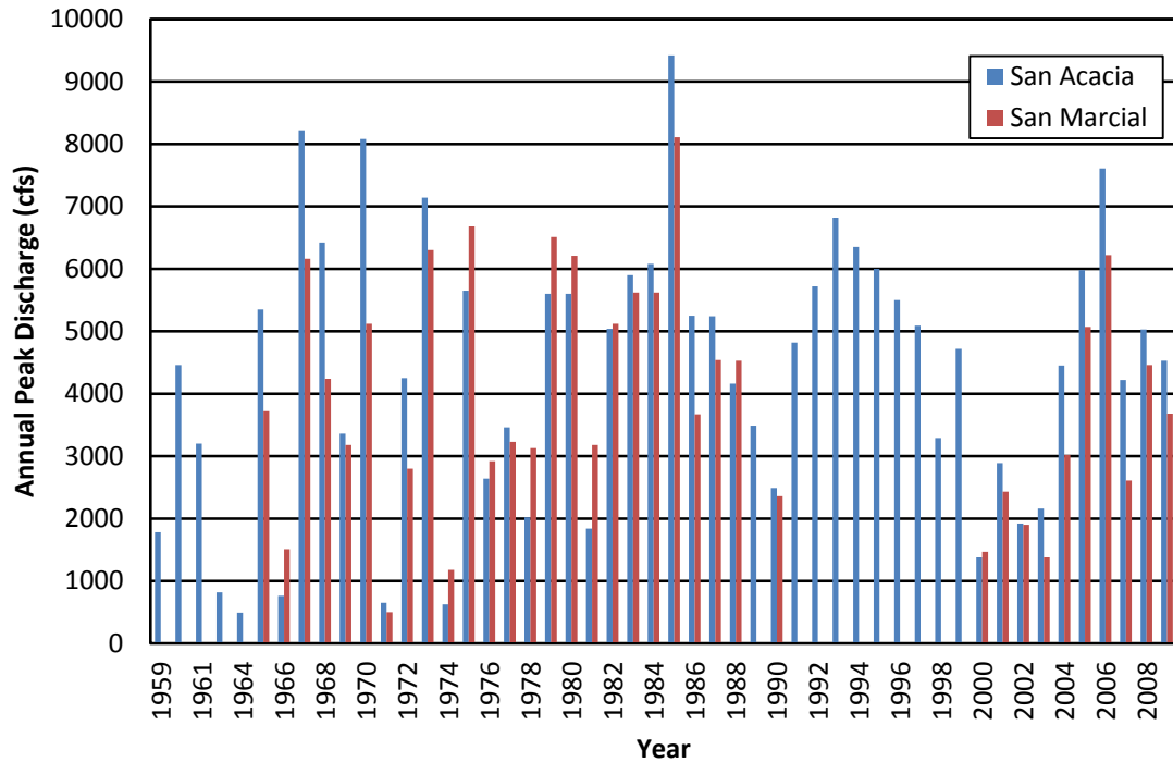
Figure 2.14 Comparison of Annual Peak Flows at San Acacia and San Marcial Gauges
