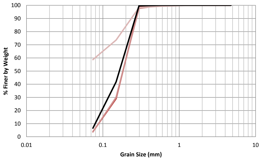
Figure H.19 EB-13 1988 Grain Size Distribution
