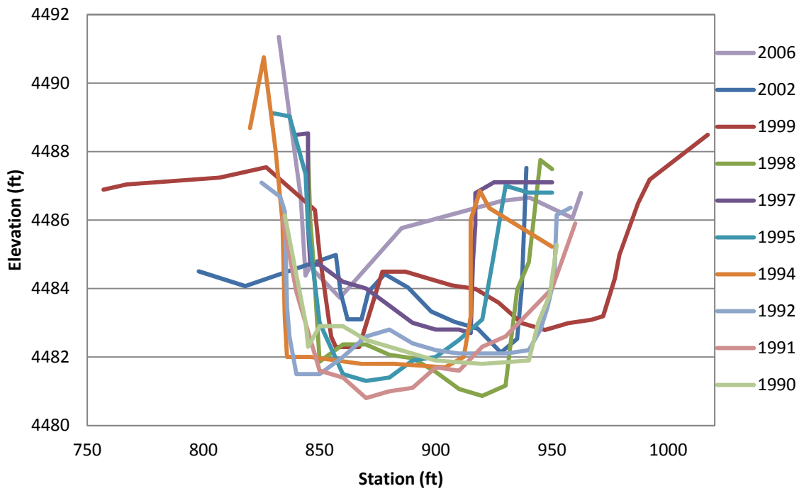
Figure F.3 SO-1666 Cross-Section
