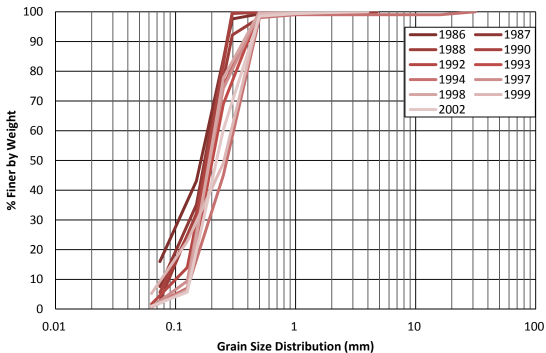
Figure 4.60 Subreach 3 (EB-10): Annual Bed Material Grain Size Distributions
