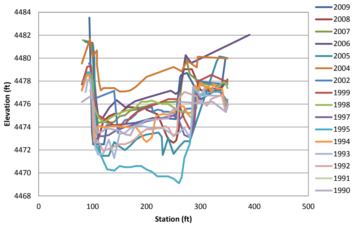
Figure F.7 SO-1701.3 Cross-Section
