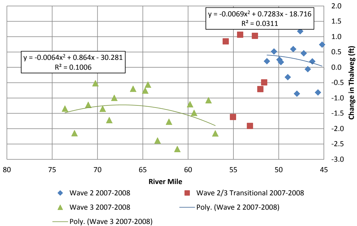
Figure G.13 2007-2008 Thalweg Change
