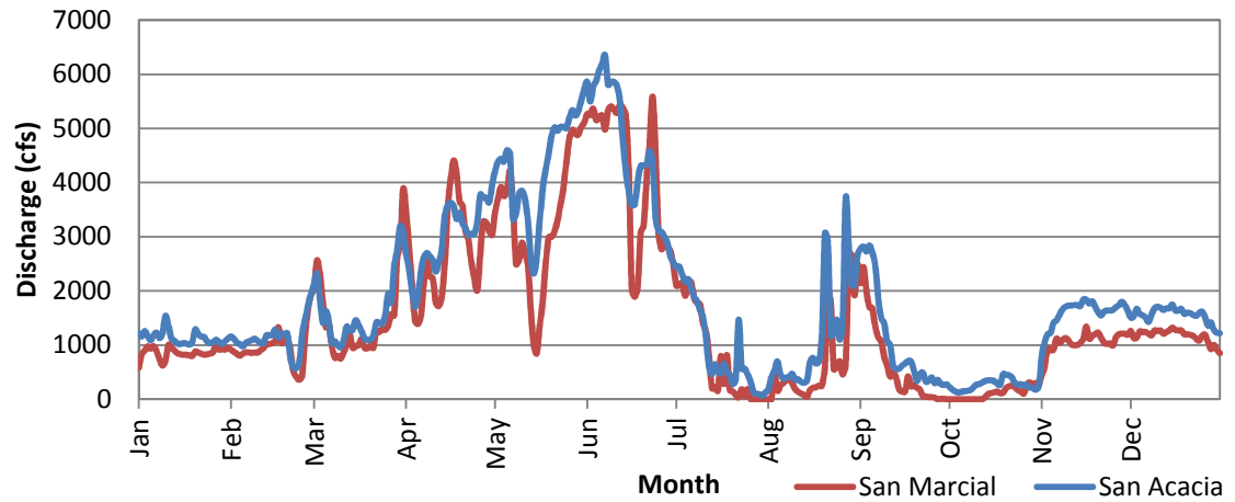
Figure B.4 1993 Daily Discharge Data
