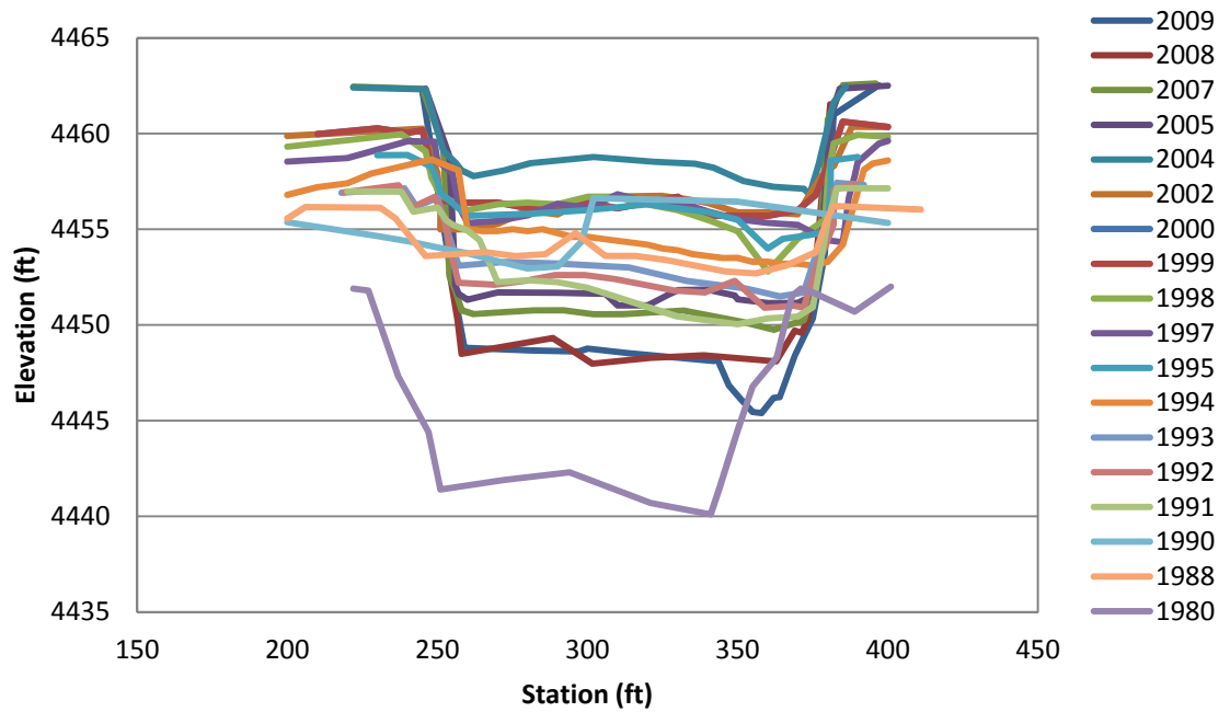
Figure F.15 EB-20 Cross-Section
