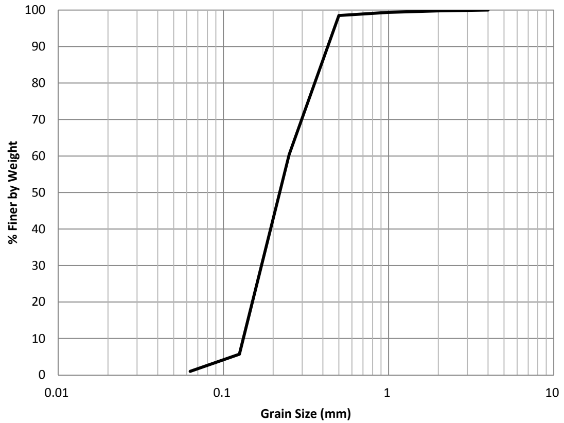
Figure H.16 EB-10 2002 Grain Size Distribution
