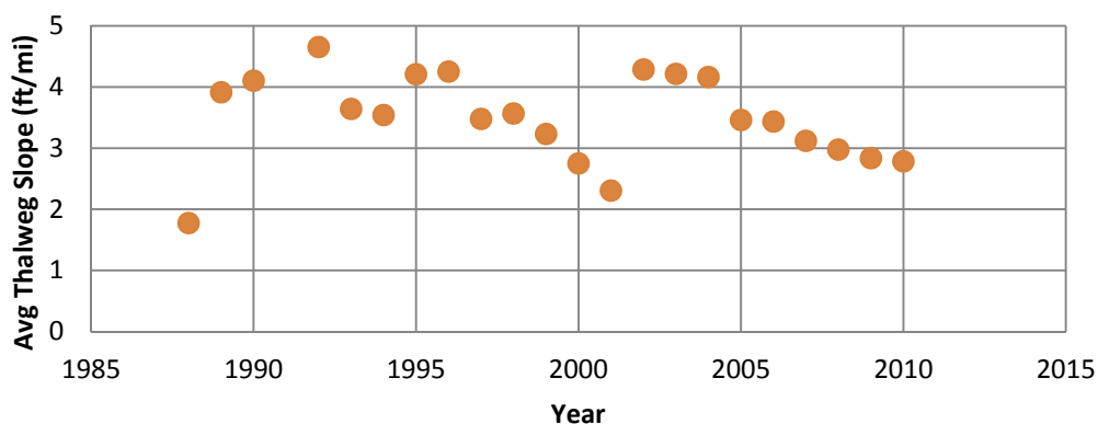
Figure 4.27 Subreach 6 Average Channel Thalweg Slope: Temporal Trend
