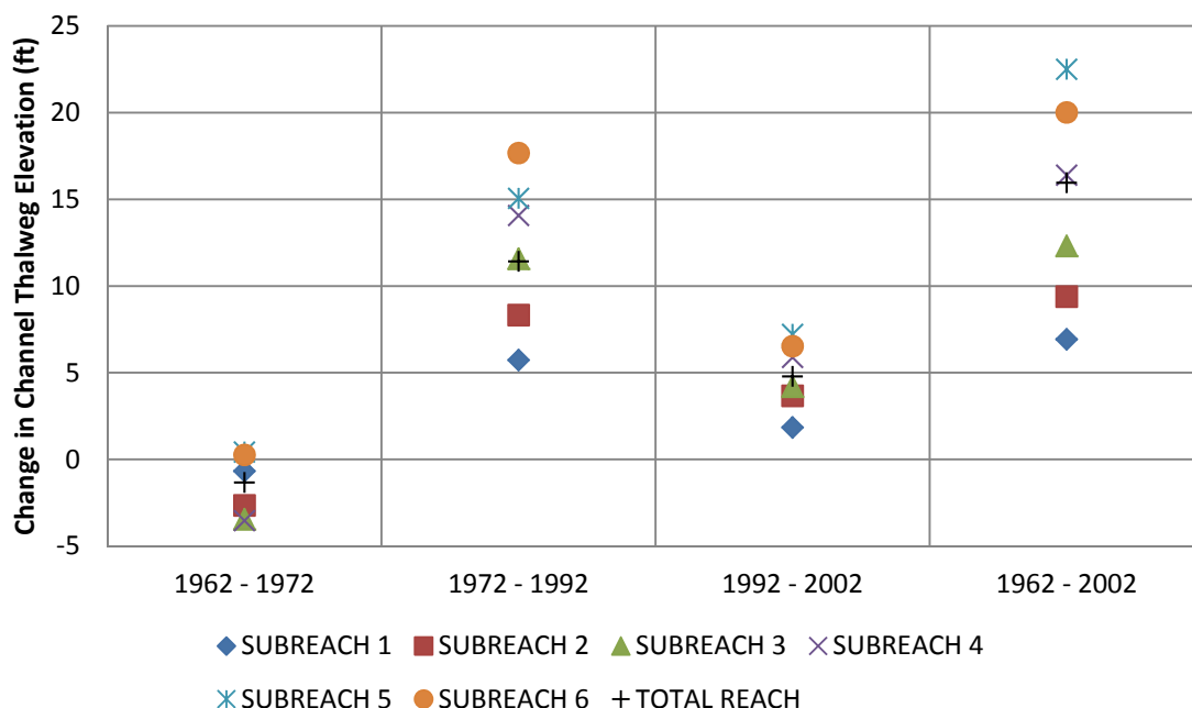
Figure 4.14 Change in Channel Thalweg Elevation from Agg/Deg Surveys
