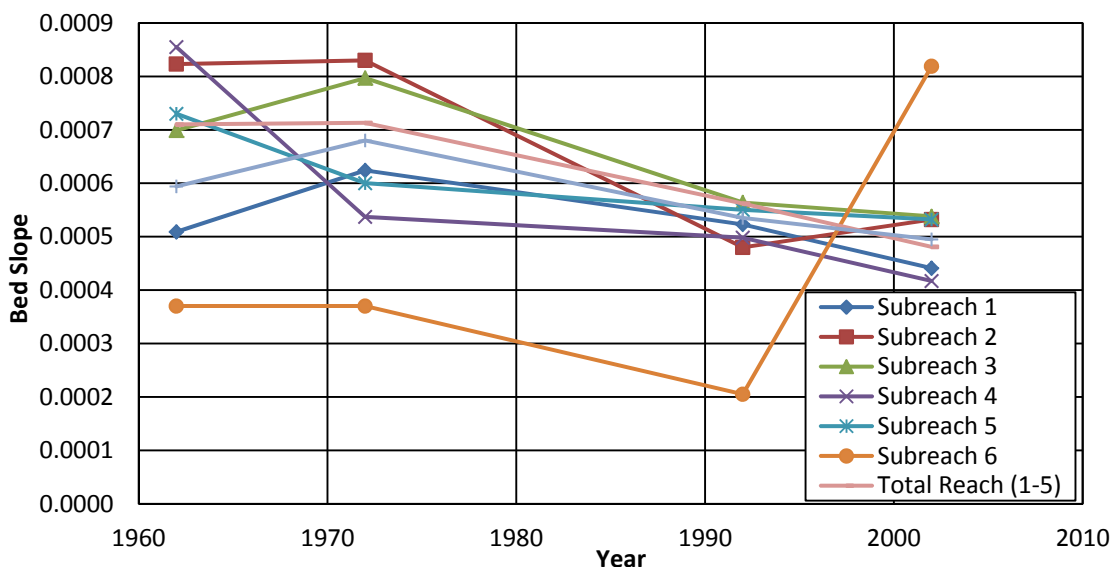
Figure 4.13 Bed Slope from Agg/Deg Surveys
