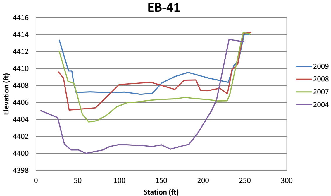
Figure 4.36 Subreach 6: EB-41 Surveyed Cross-Sections
