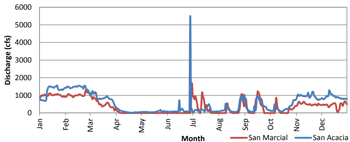
Figure B.7 1996 Daily Discharge Data
