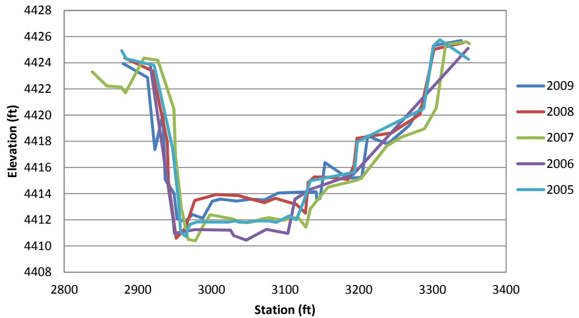
Figure F.35 EB-38 Cross-Section
