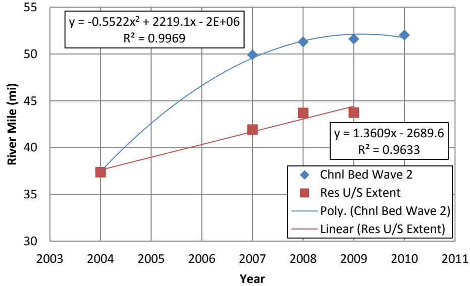
Figure 4.50 Rate of Wave 2 Propagation Upstream
