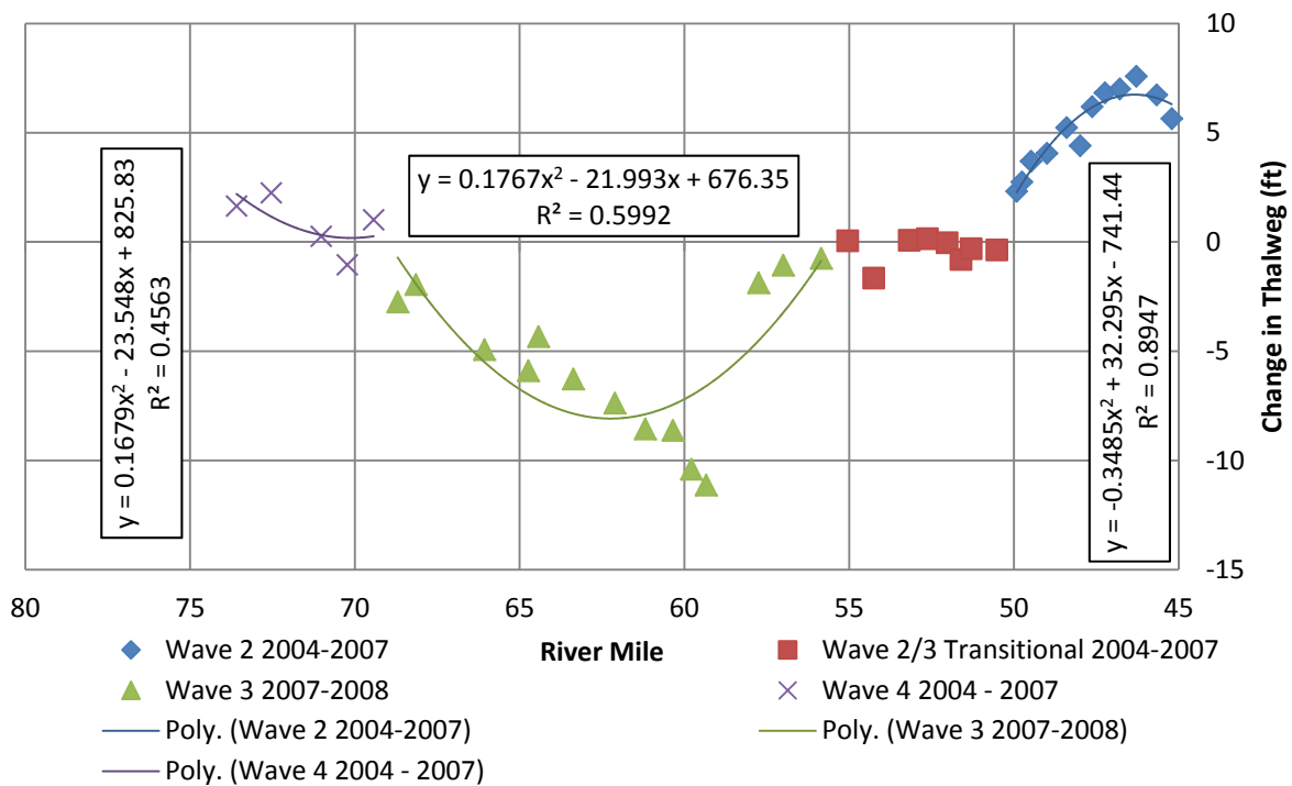
Figure G. 12 2004-2007 Thalweg Change
