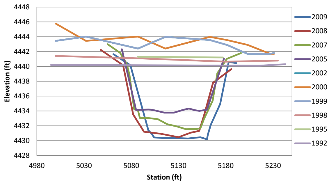
Figure F.22 EB-28 Cross-Section
