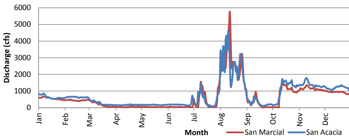
Figure B.17 2006 Daily Discharge Data
