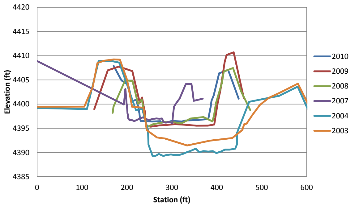
Figure F.47 EB-49 Cross-Section
