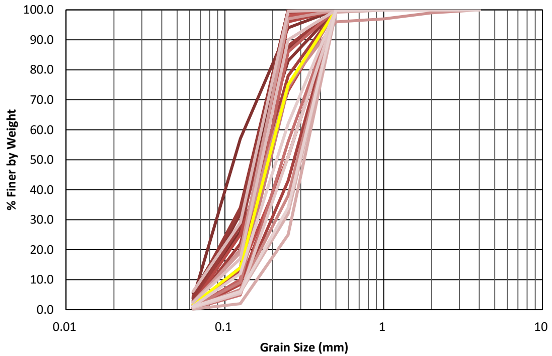
Figure 4.55 EB-10 1992 Bed Material Grain Size Distributions
