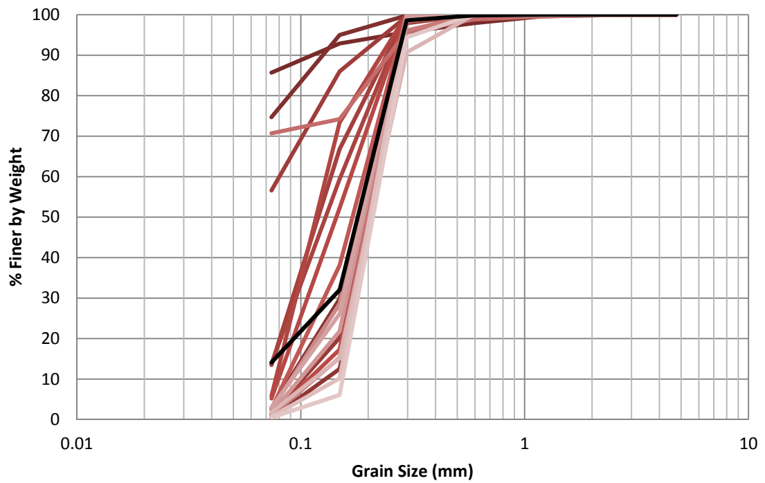
Figure H.17 EB-13 1986 Grain Size Distribution
