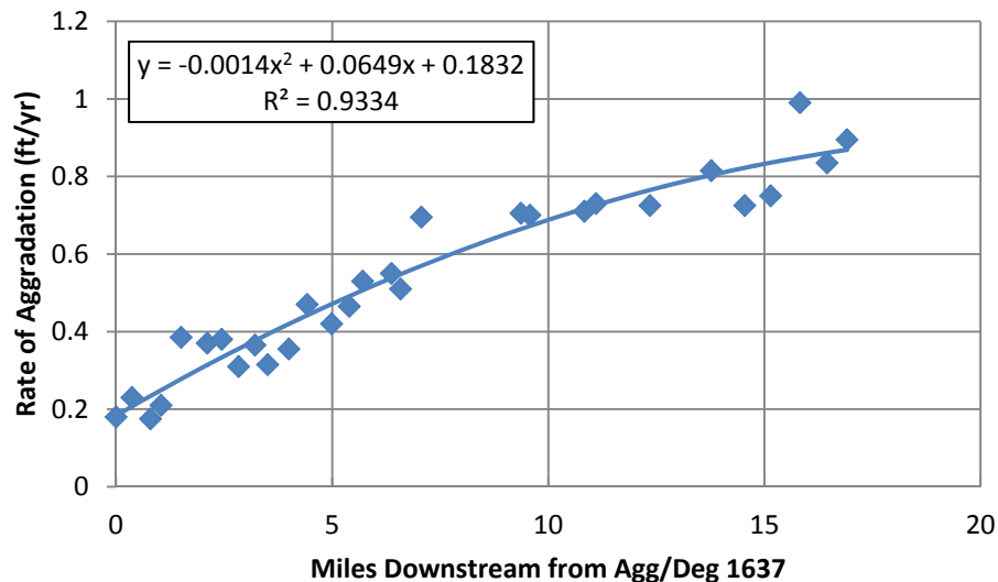
Figure 4.20 Rate of Channel Aggradation between 1972 and 1992
