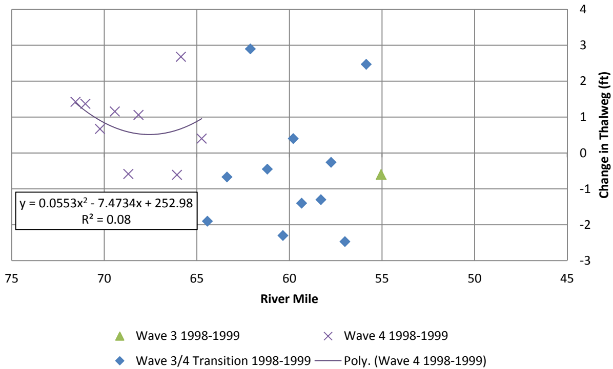
Figure G.8 1998-1999 Thalweg Change
