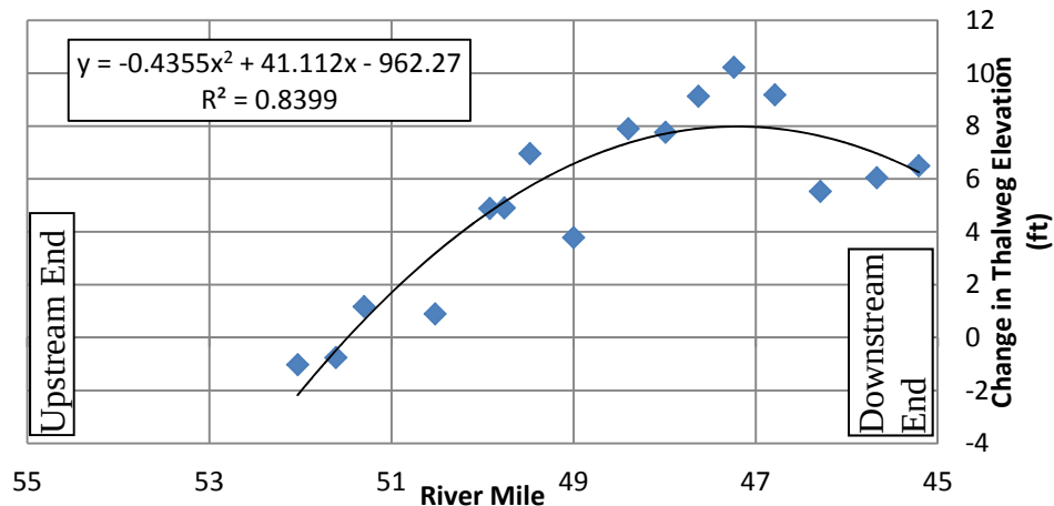
Figure 4.46 Magnitude of Aggradation from 2004-2009
