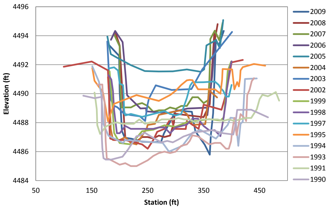
Figure F.2 SO-1652.7 Cross-Section
