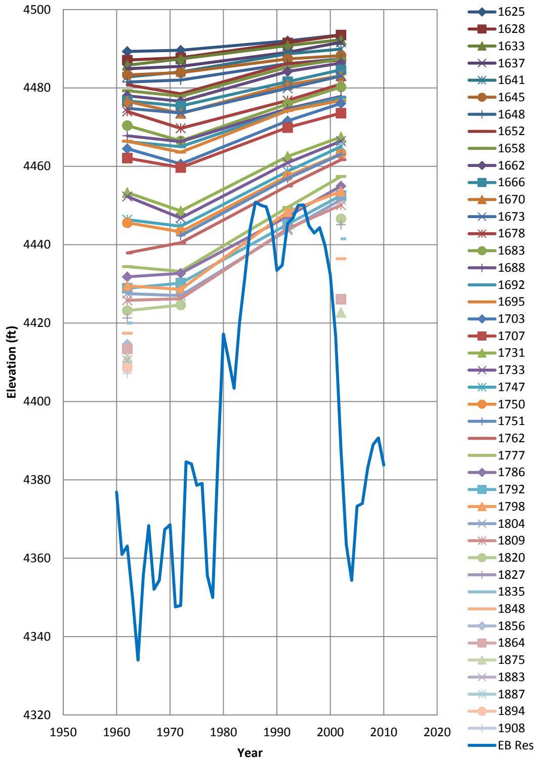
Figure 4.19 Temporal Trend in Thalweg Elevation at Agg/Deg Lines
