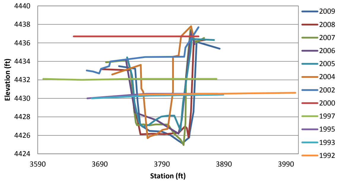
Figure F.26 EB-30 Cross-Section
