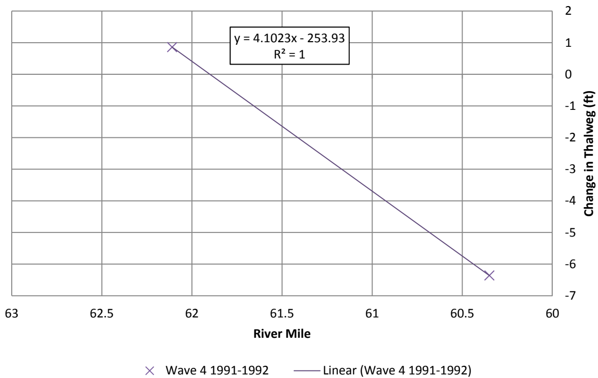
Figure G.2 1991-1992 Thalweg Change
