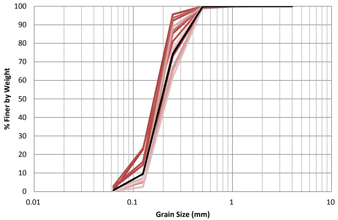
Figure H.12 EB-10 1994 Grain Size Distribution
