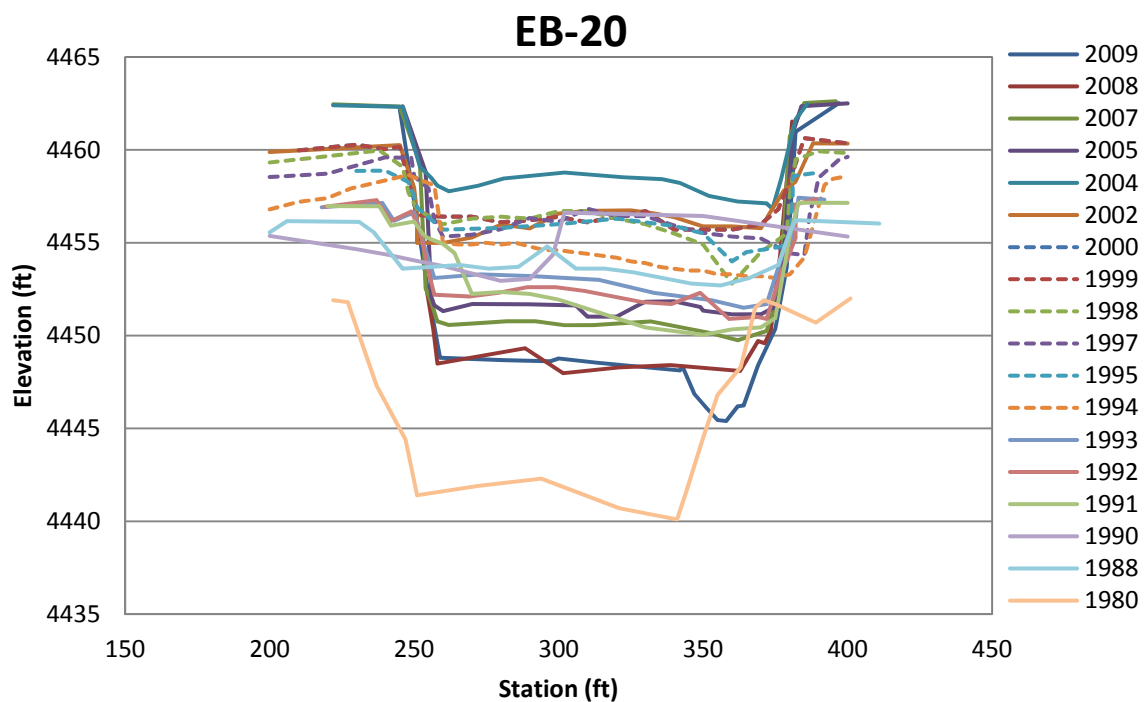
Figure 4.33 Subreach 5: EB-20 Surveyed Cross-Sections
