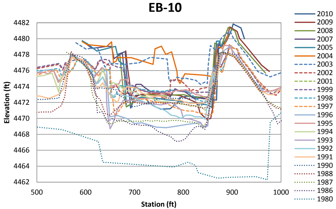
Figure 4.30 Subreach 3: EB-10 Surveyed Cross-Sections
