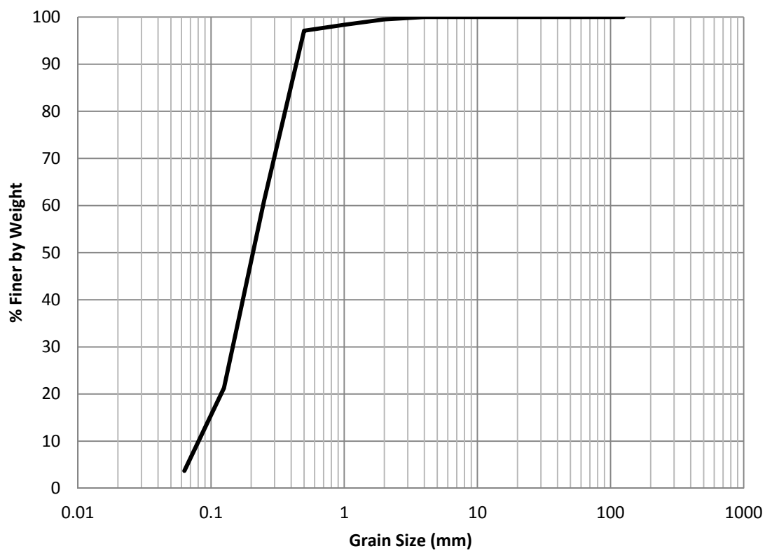
Figure H.21 EB-13 1999 Grain Size Distribution
