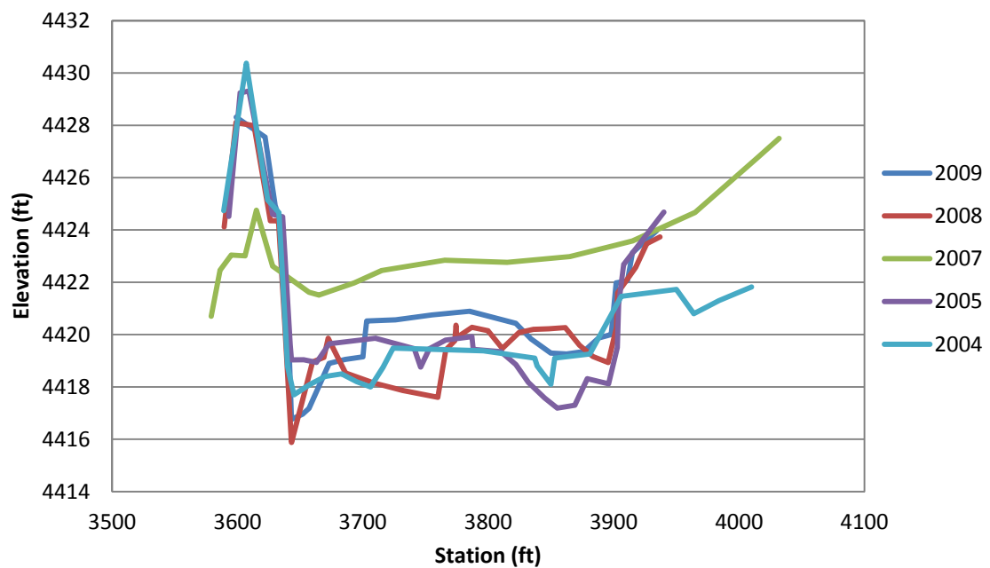
Figure F.31 EB-35 Cross-Section
