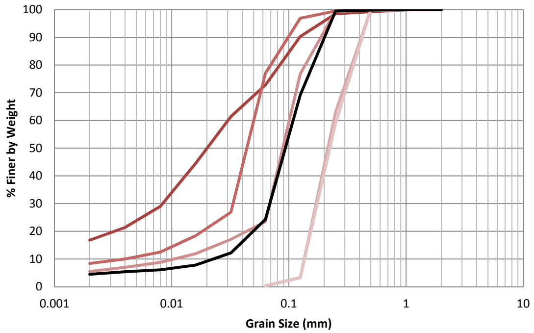
Figure H.34 EB-24 1999 Grain Size Distribution
