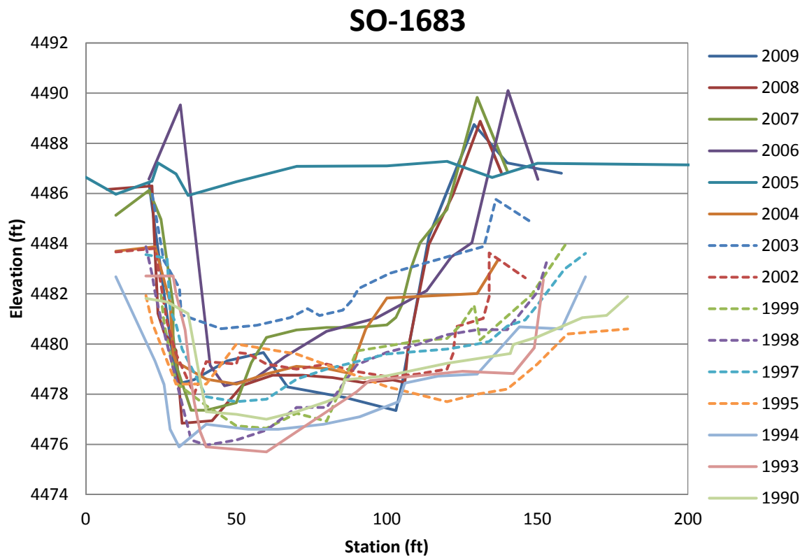
Figure 4.29 Subreach 2: SO-1683 Surveyed Cross-Sections
