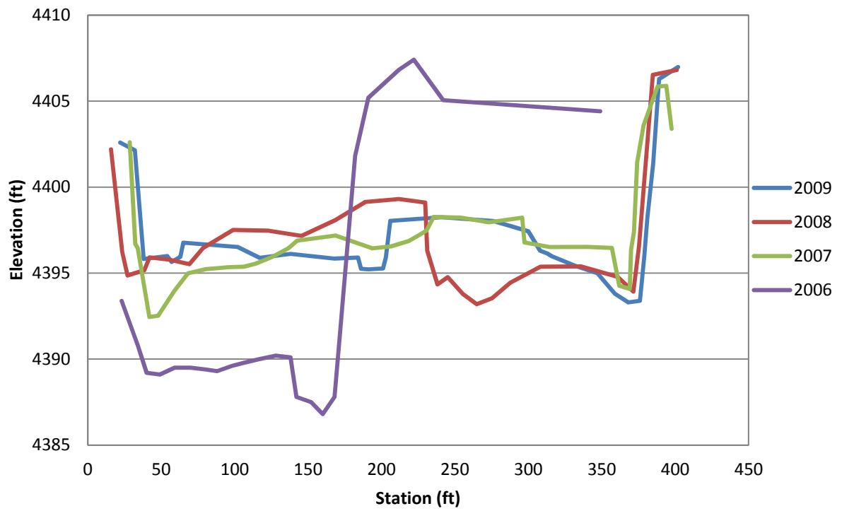
Figure F.48 EB-50 Cross-Section
