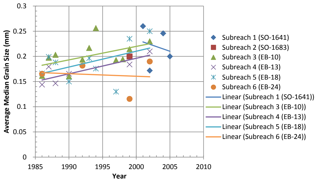
Figure 4.65 Average Median Bed Material Grain Size: Subreach Temporal Trends
