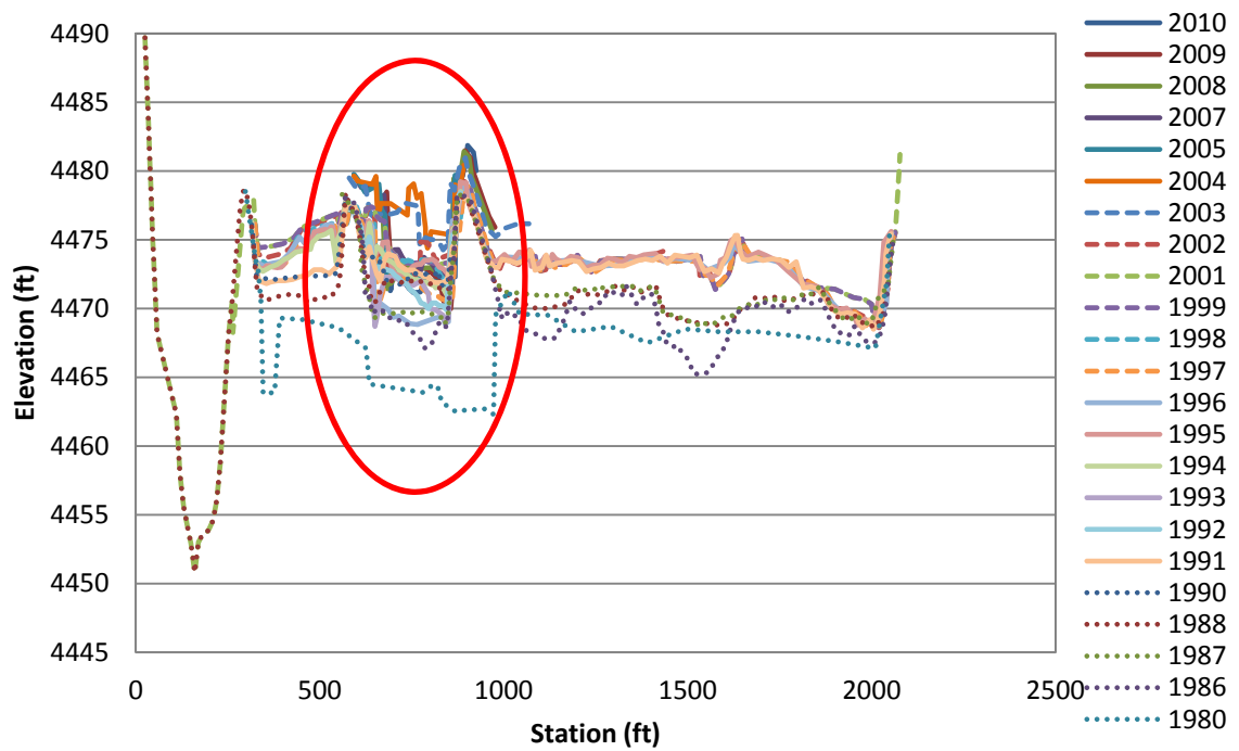
Figure F.9 EB-10 (w/Floodplain) Cross-Section
