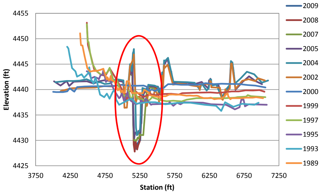
Figure F.25 EB-29 (w/Floodplain) Cross-Section
