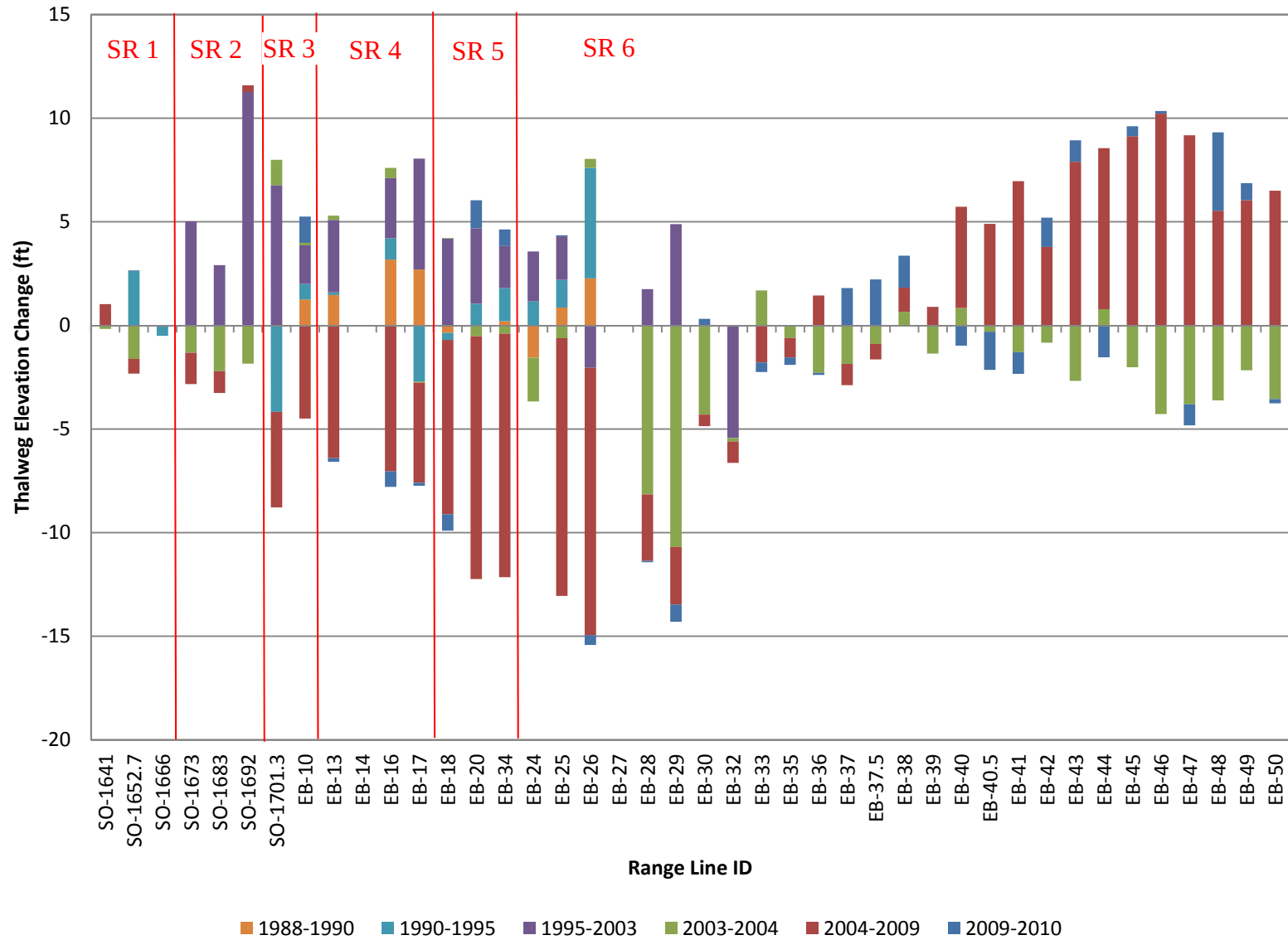
Figure 4.39 Change in Channel Thalweg Elevations at Range Lines (1988-2010)
