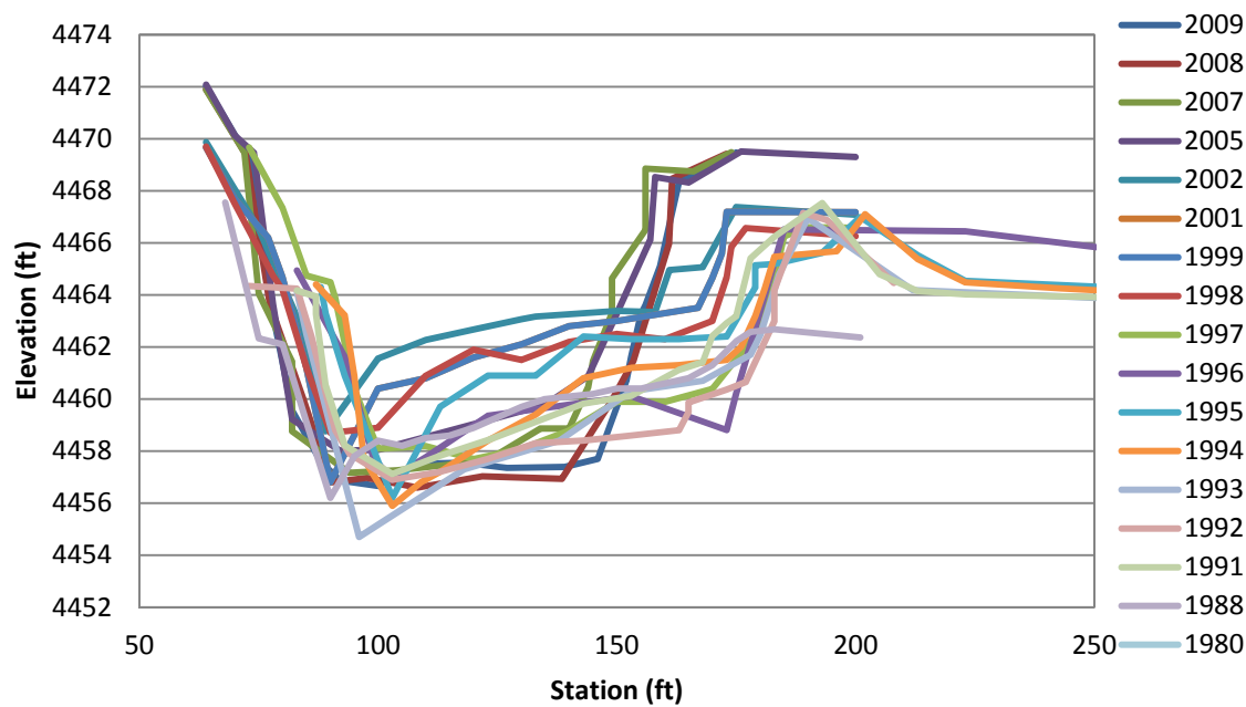
Figure F.13 EB-17 Cross-Section
