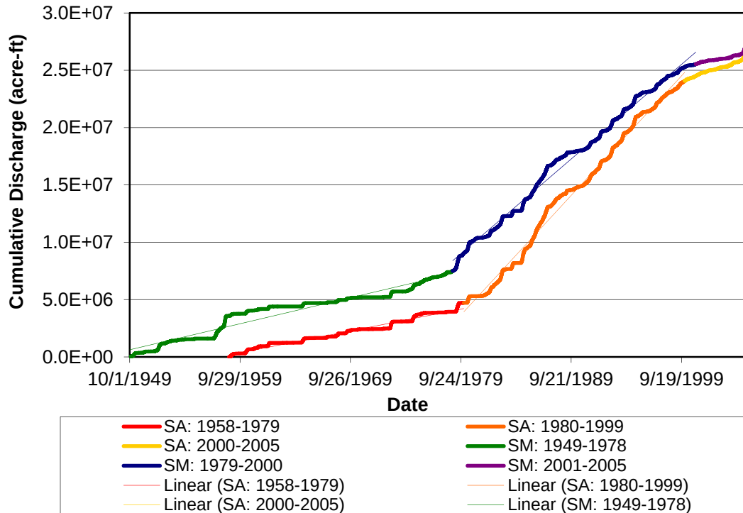
Figure 4.66 Water Discharge Single Mass Curve (Larsen et al. 2007)
