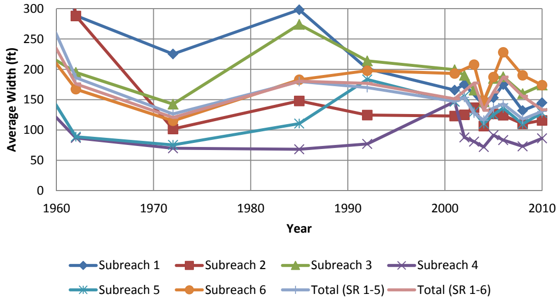
Figure 4.9 Channel Widths from GIS (1962 - 2010)
