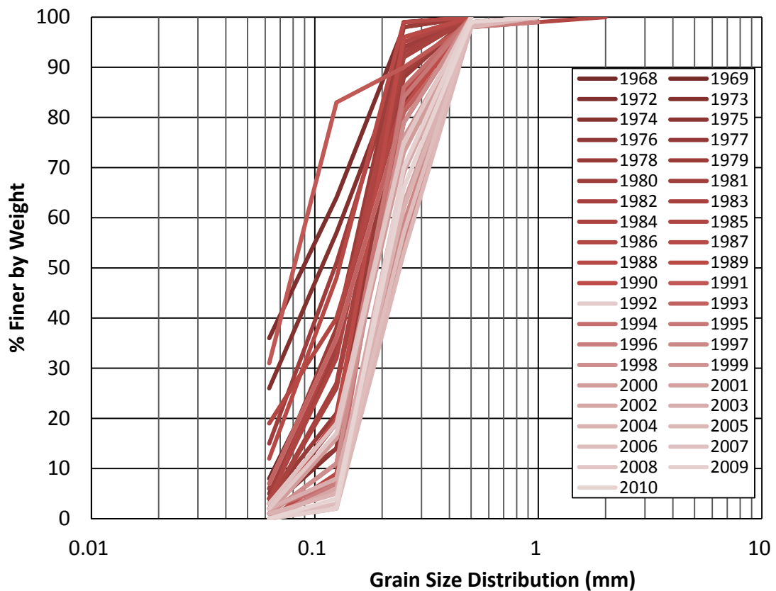
Figure 4.57 San Marcial Gauge: Annual Bed Material Grain Size Distributions
