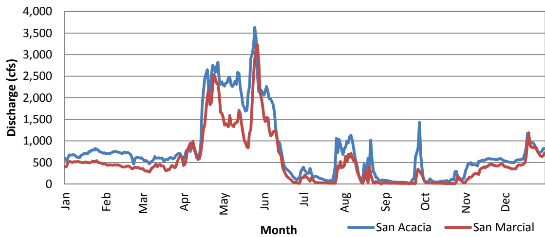
Figure B.21 2010 Daily Discharge Data
