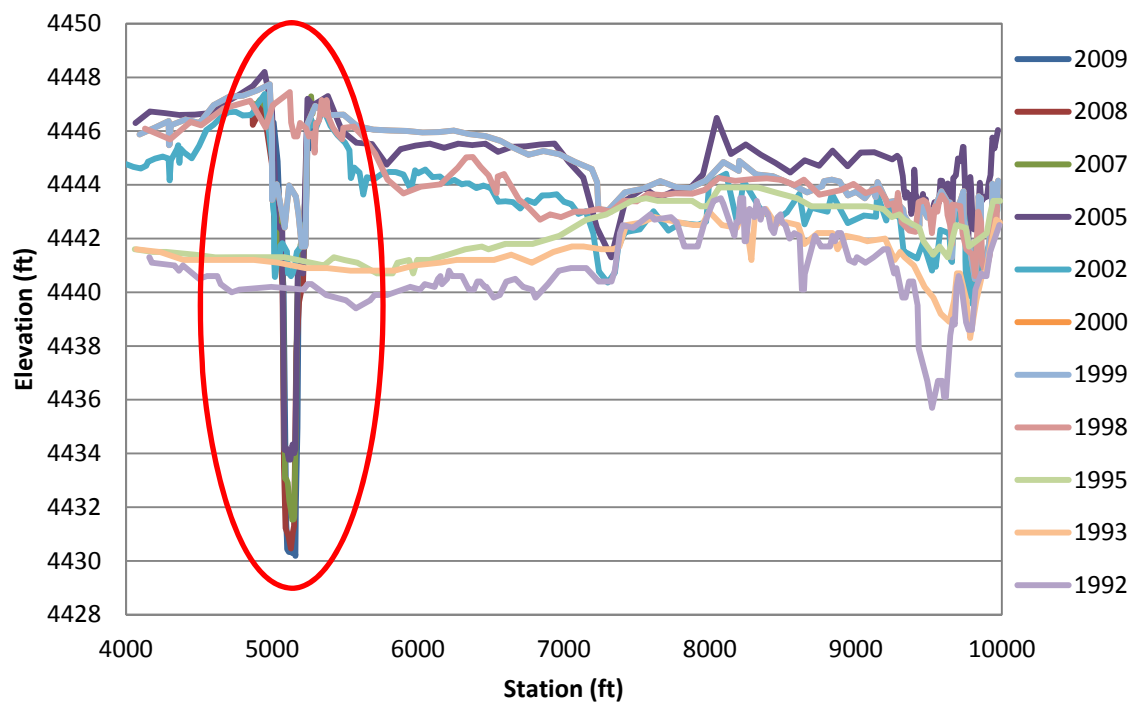
Figure F.23 EB-28 (w/Floodplain) Cross-Section
