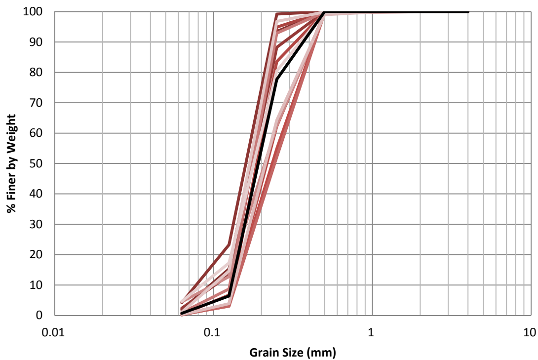
Figure H.14 EB-10 1998 Grain Size Distribution
