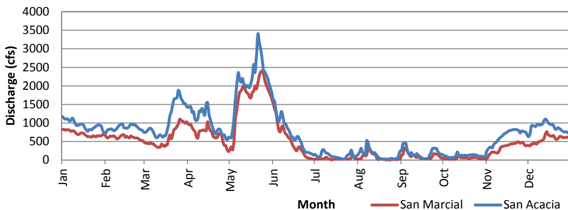
Figure B.18 2007 Daily Discharge Data
