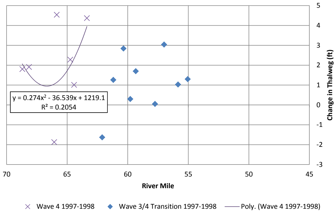
Figure G.7 1997-1998 Thalweg Change
