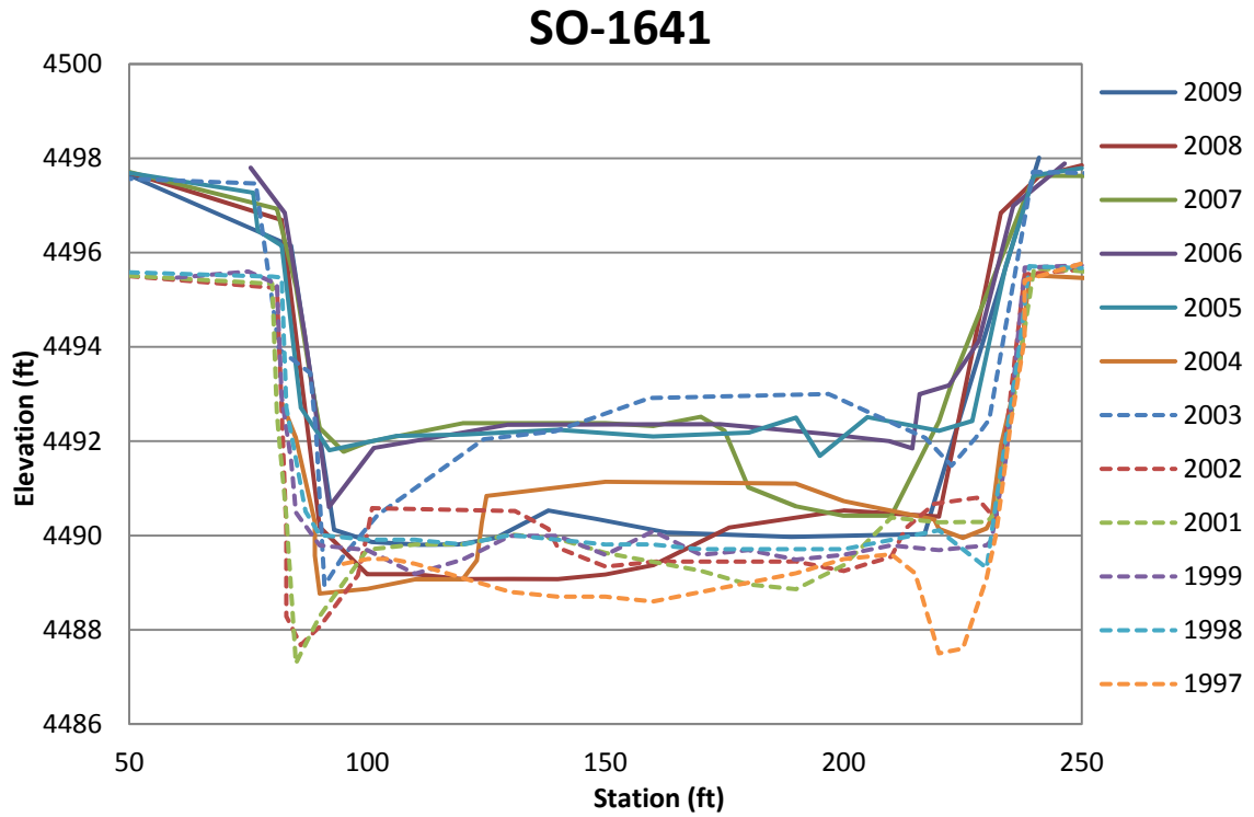
Figure 4.28 Subreach 1: SO-1641 Surveyed Cross-Sections
