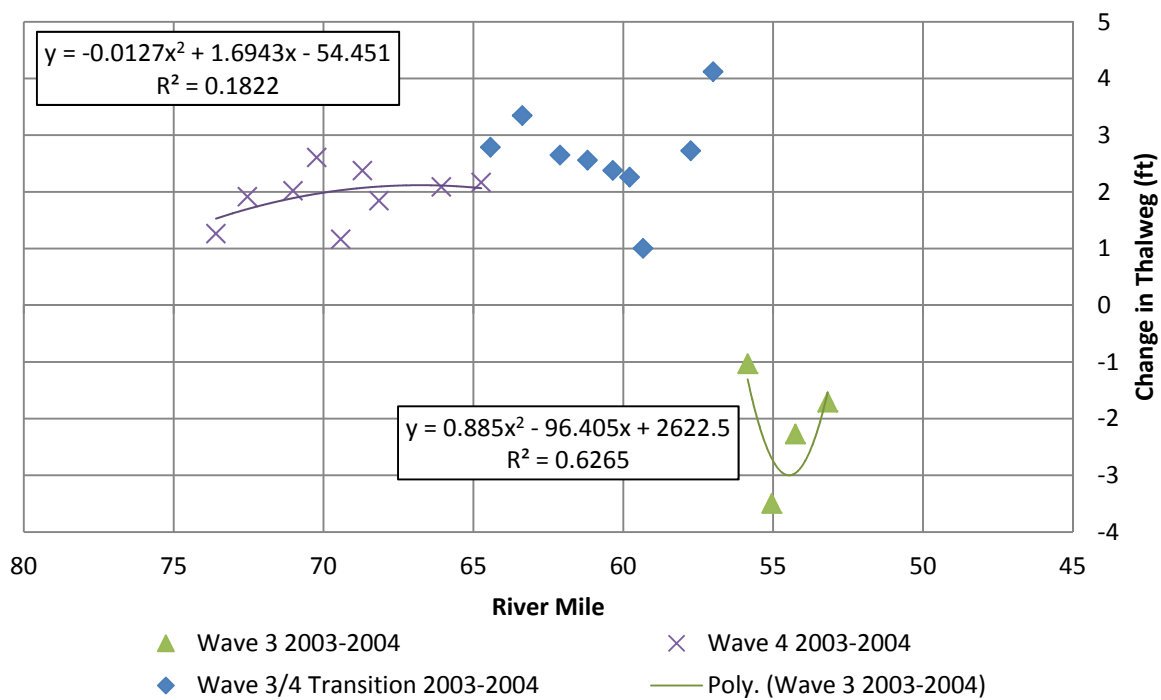
Figure G.10 2002-2003 Thalweg Change
