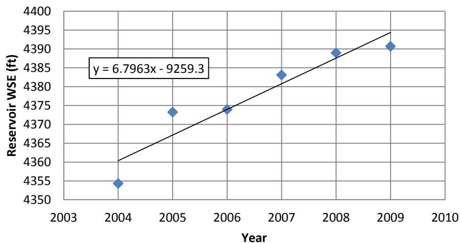
Figure 4.49 Reservoir Water Surface Elevation Change from 2004-2009 Resulting in Wave 2 Channel Aggradation
