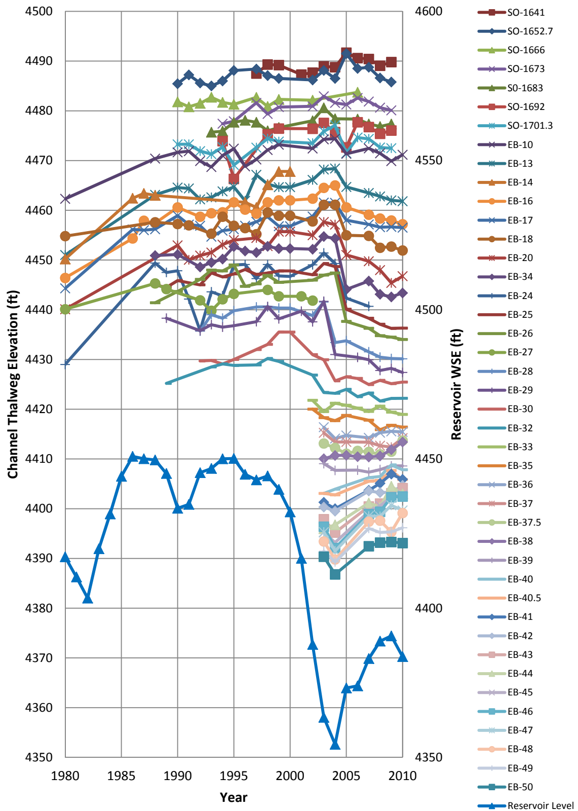
Figure 4.37 Change in Thalweg Elevation at Range Lines (1980 – 2010)
