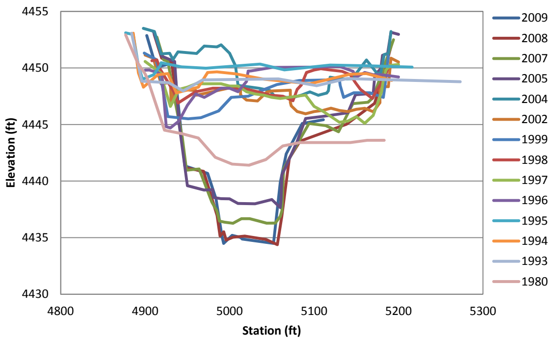
Figure F.19 EB-26 Cross-Section
