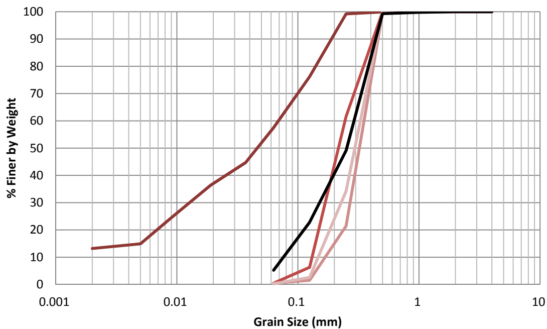
Figure H.14 EB-10 1998 Grain Size Distribution
