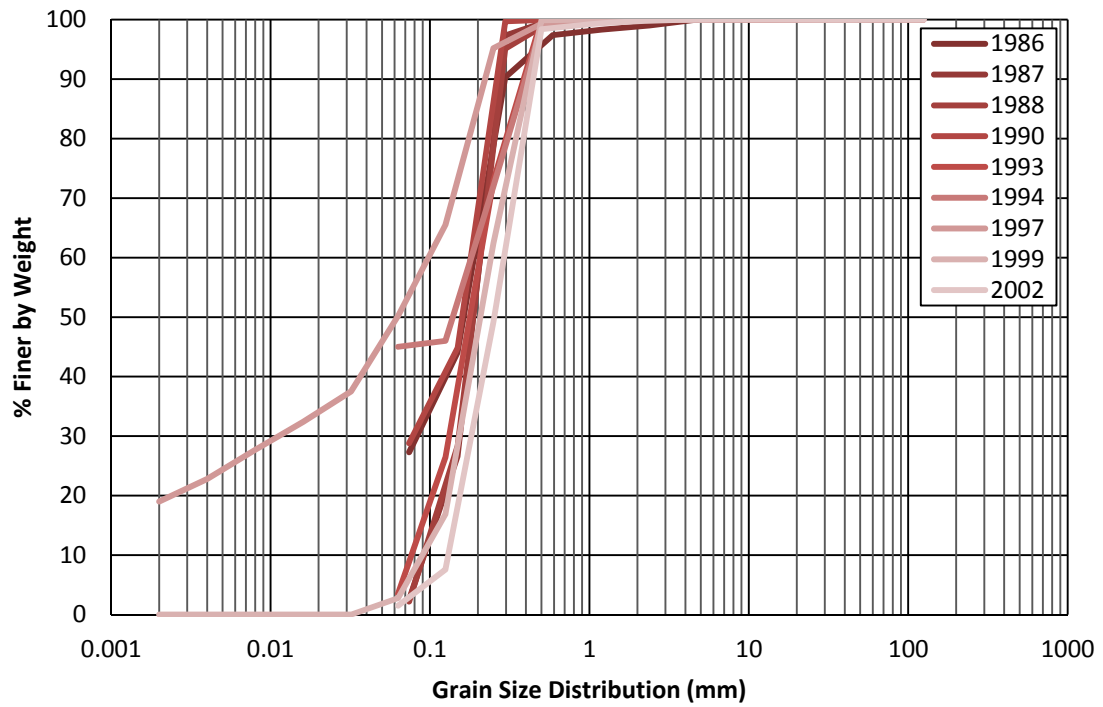
Figure 4.62 Subreach 5 (EB-18): Annual Bed Material Grain Size Distributions
