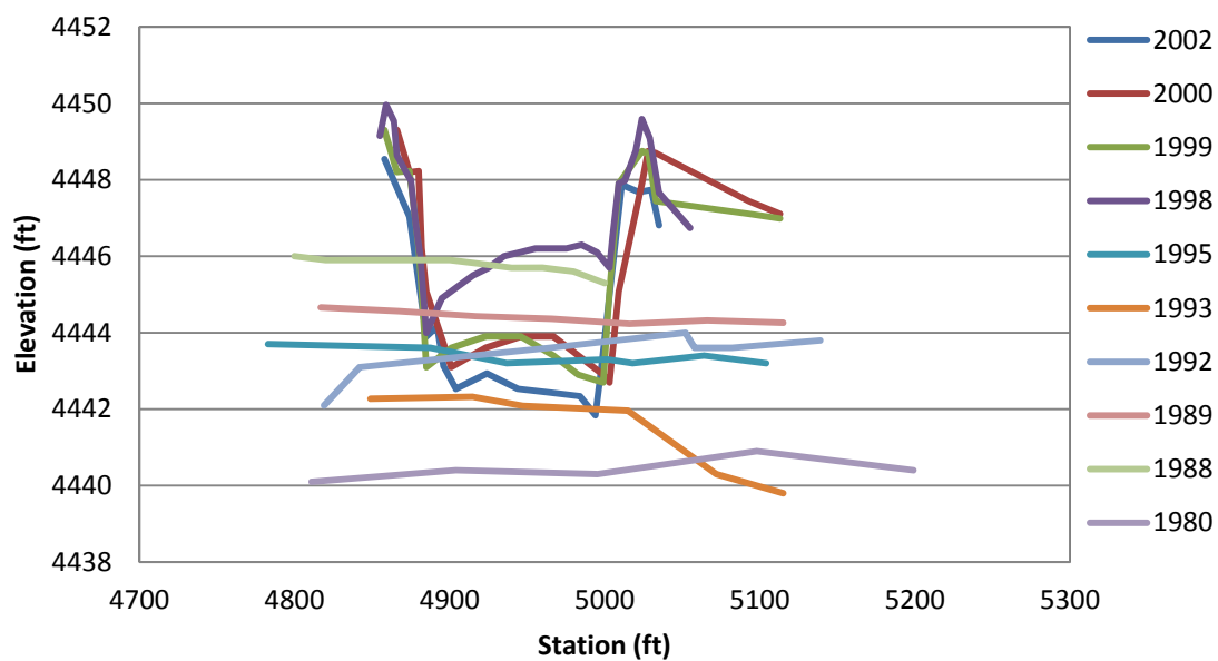
Figure F.20 EB-27 Cross-Section
