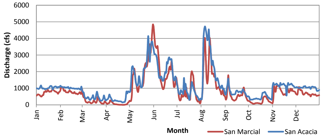
Figure B.10 1999 Daily Discharge Data
