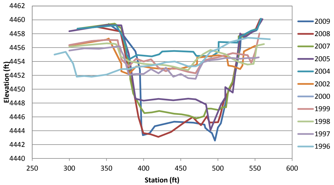
Figure F.16 EB-34 Cross-Section
