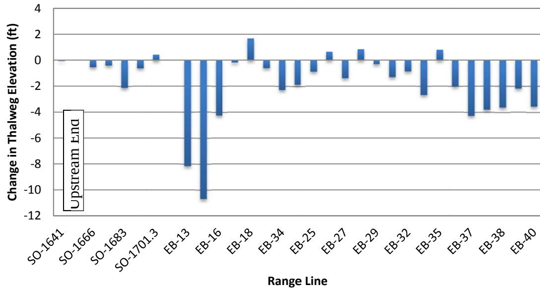
Figure 4.40 Magnitude of Aggradation and Degradation at Range Lines (2003-2004)
