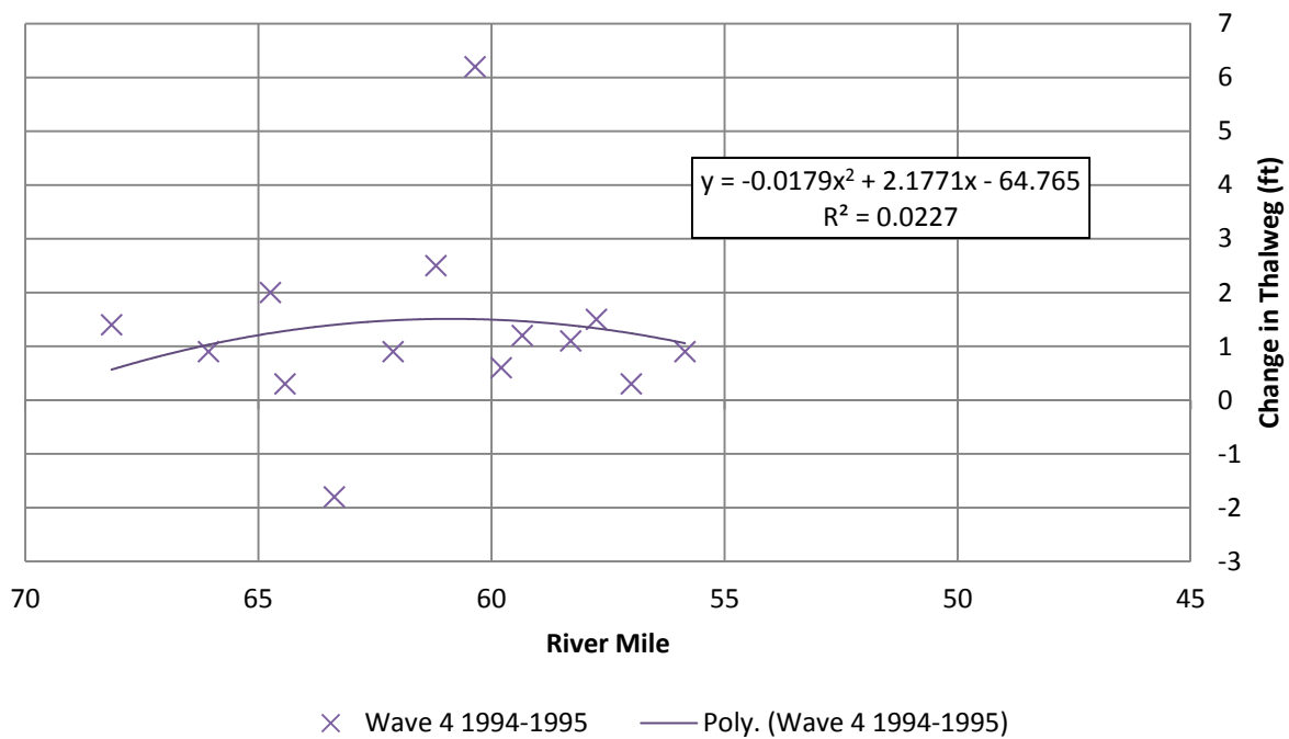
Figure G.5 1994-1995 Thalweg Change
