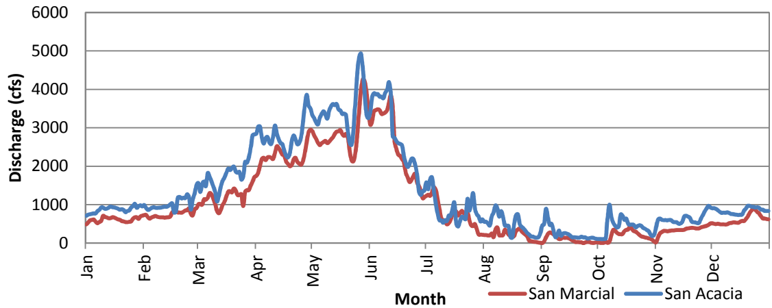
Figure B.19 2008 Daily Discharge Data
