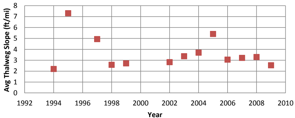
Figure 4.23 Subreach 2 Average Channel Thalweg Slope: Temporal Trend
