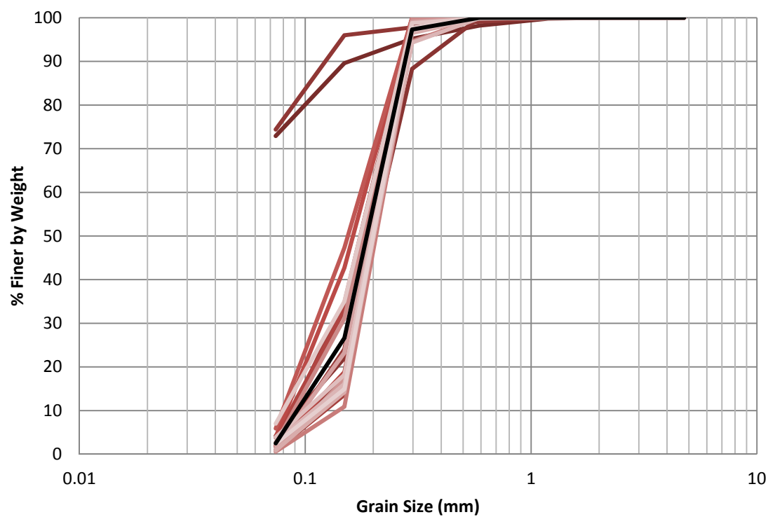
Figure H.23 EB-18 1986 Grain Size Distribution
