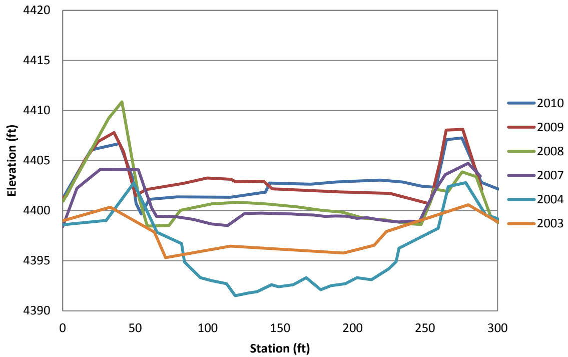
Figure F.45 EB-47 Cross-Section
