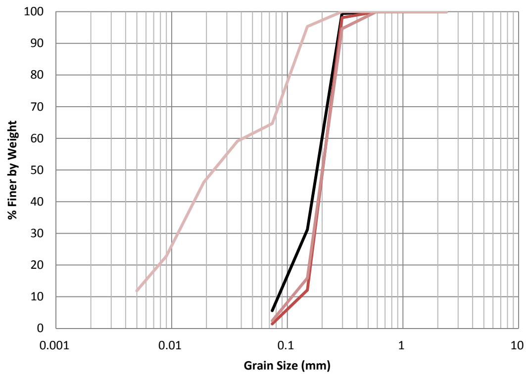
Figure H.9 EB-10 1990 Grain Size Distribution
