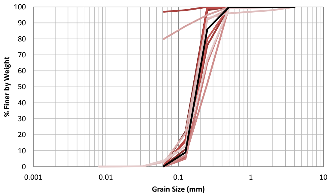
Figure H.32 EB-24 1986 Grain Size Distribution
