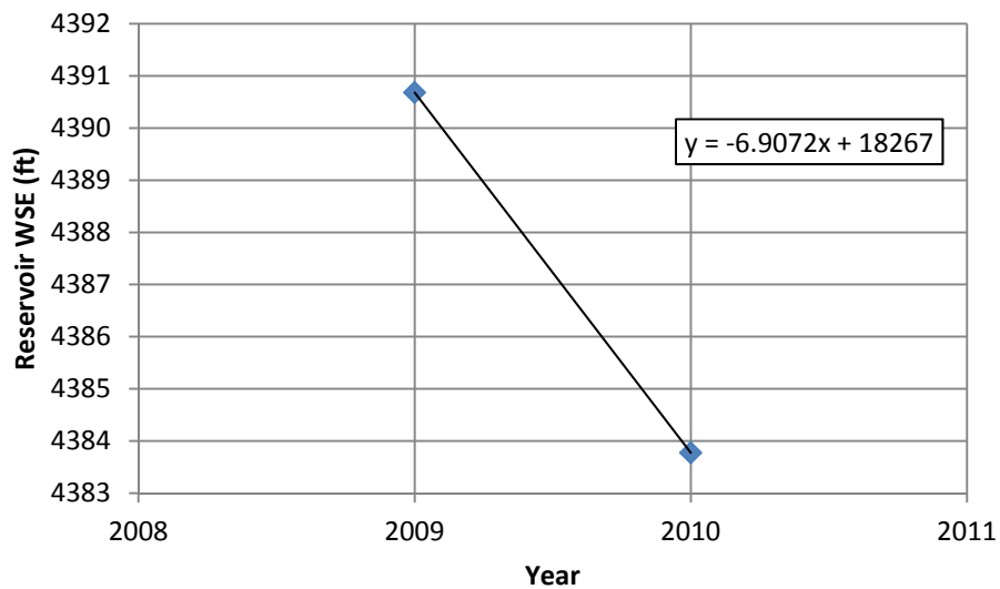
Figure 4.47 Reservoir Water Surface Elevation Change from 2009-2010 Resulting in Wave 1 Channel Degradation
