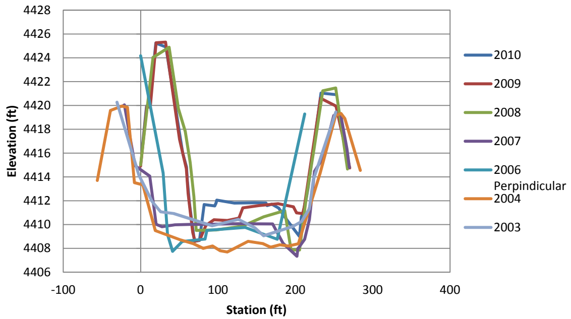
Figure F.36 EB-39 Cross-Section
