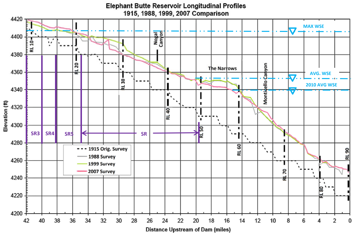
Figure 95 - Elephant Butte Reservoir Longitudinal Profiles
