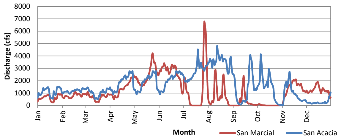
Figure B.2 1991 Daily Discharge Data
