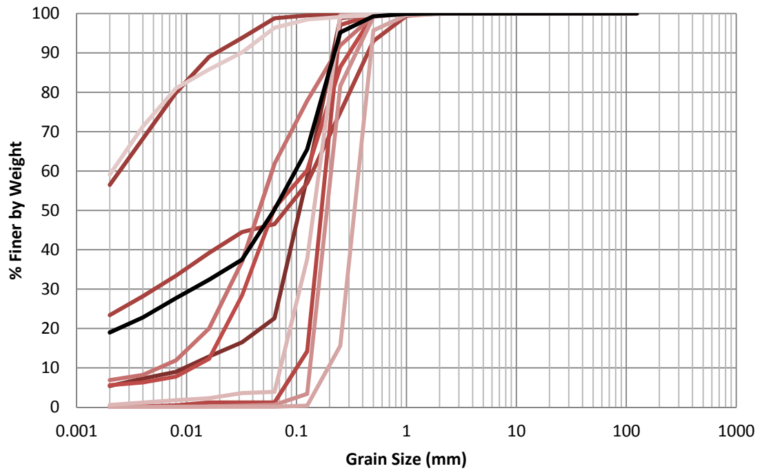
Figure H.29 EB-18 1997 Grain Size Distribution
