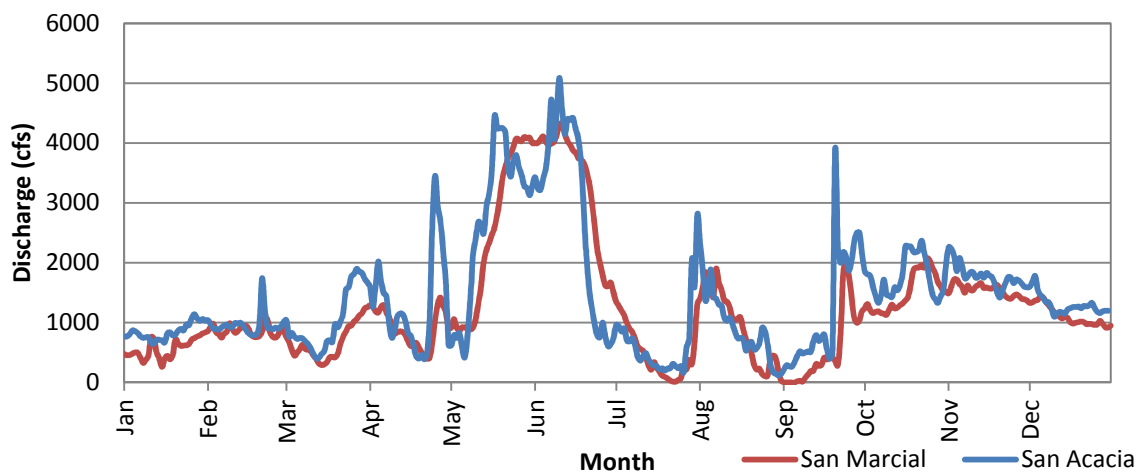
Figure B.8 1997 Daily Discharge Data
