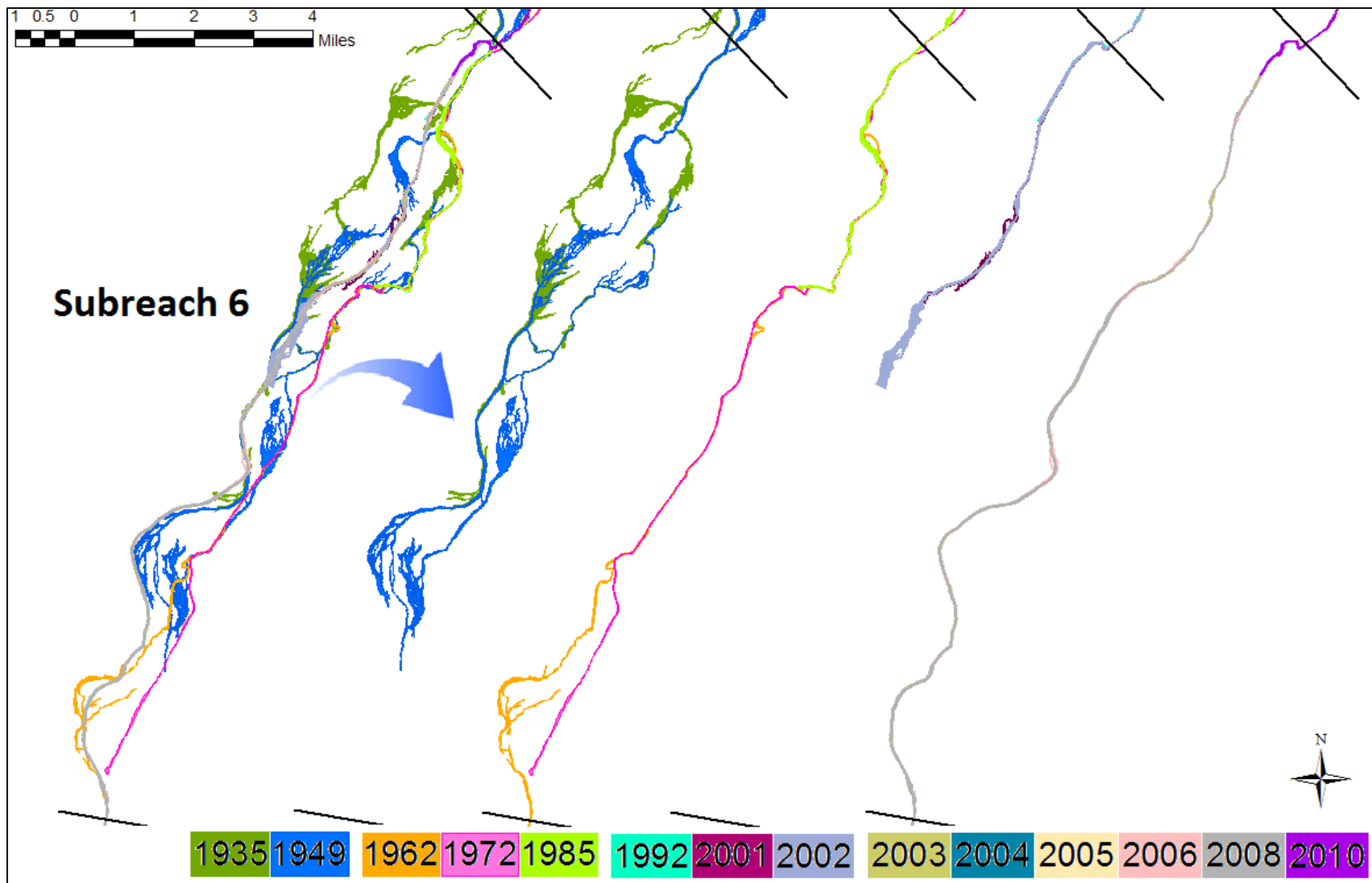
Figure 4.7 Subreach 6 Channel Planforms from Aerial Photography
