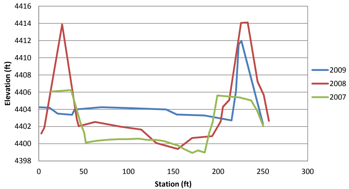
Figure F.44 EB-46 Cross-Section
