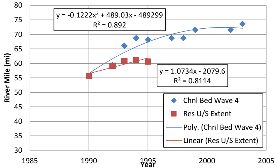
Figure 4.54 Rate of Wave 4 Propagation Upstream
