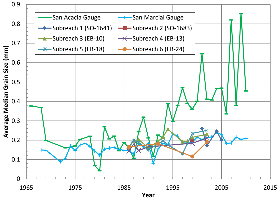
Figure 4.64 Average Median Bed Material Grain Size Temporal Trends
