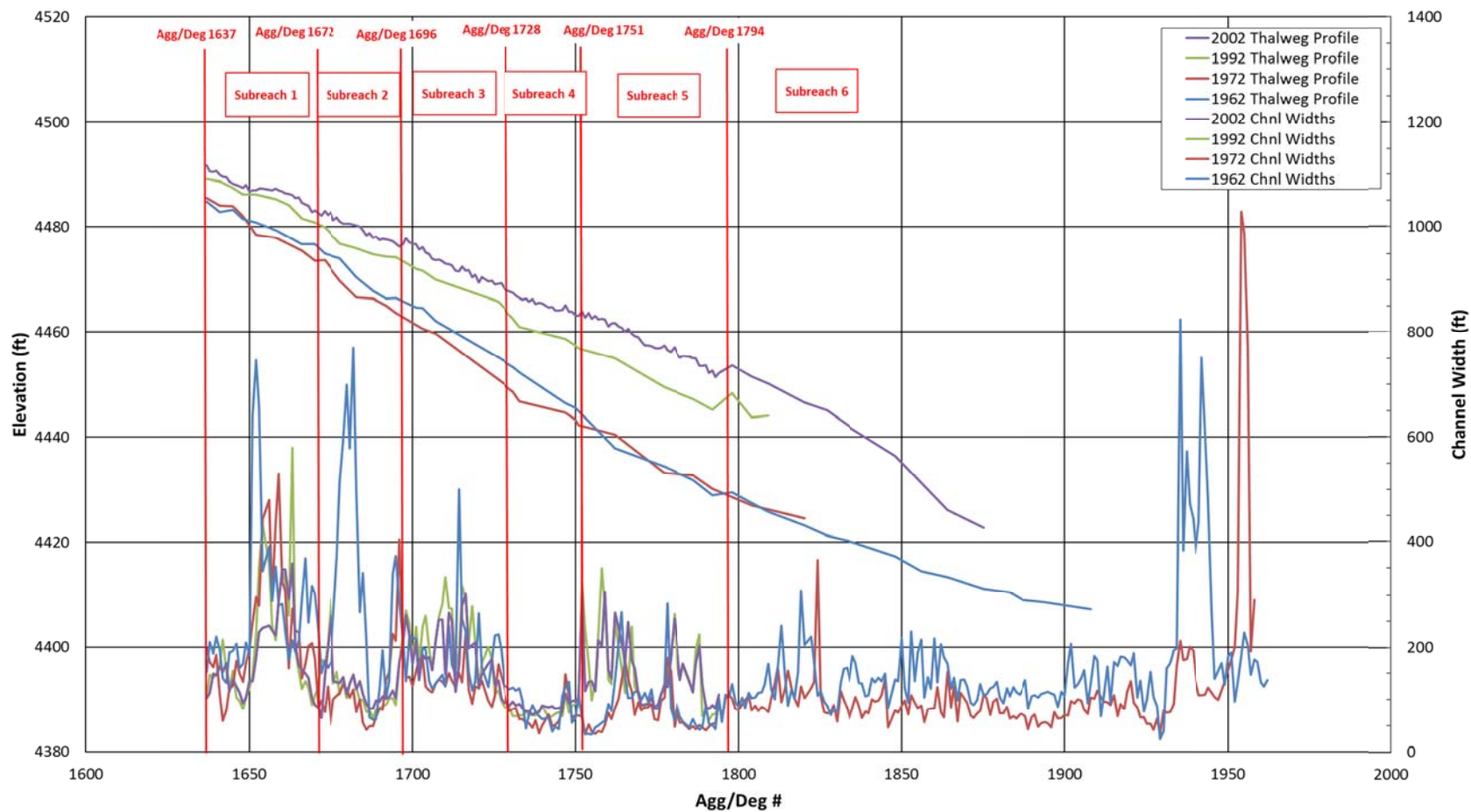
Figure 2.2 Profile of Elephant Butte Reach Widths and Thalweg at Agg/Deg Lines
