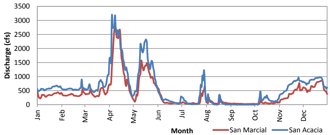
Figure B. 15 2004 Daily Discharge Data
