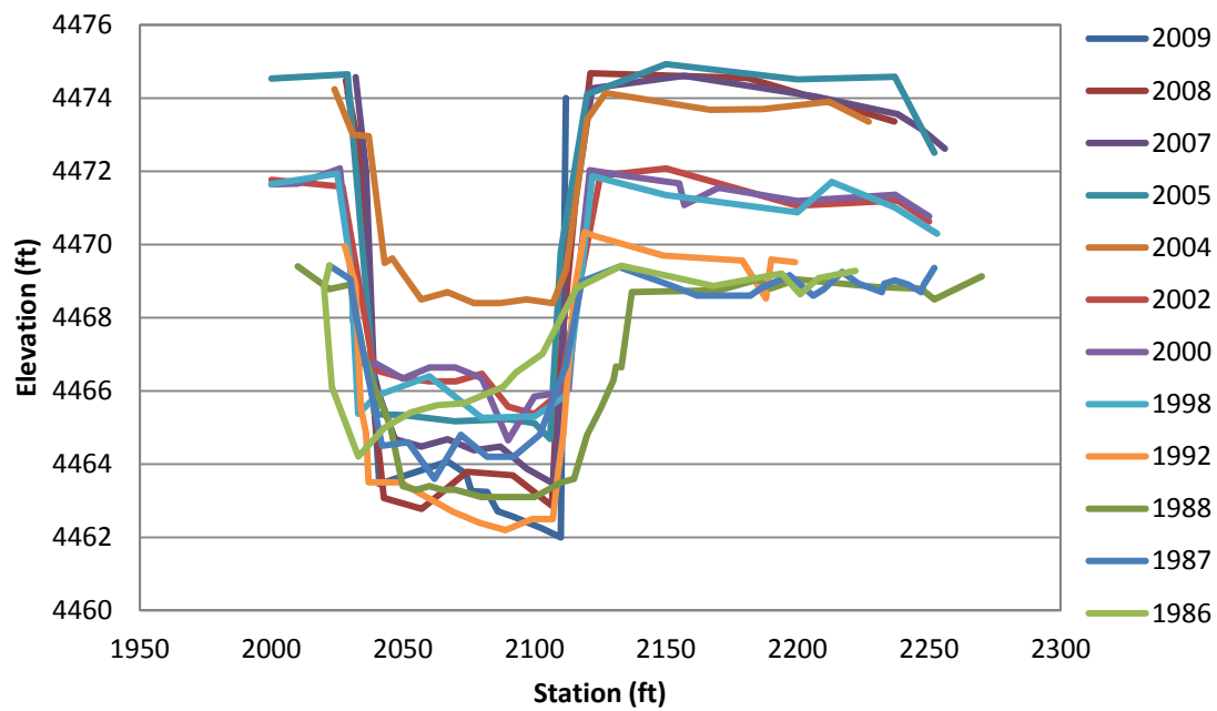
Figure F.10 EB-13 Cross-Section
