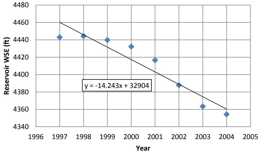
Figure 4.51 Reservoir Water Surface Elevation Change from 1997-2004 Resulting in Wave 3 Channel Degradation
