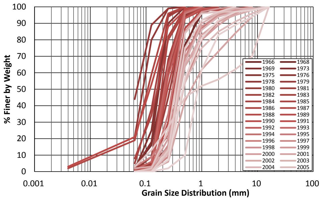
Figure 4.56 San Acacia Gauge: Annual Bed Material Grain Size Distributions
