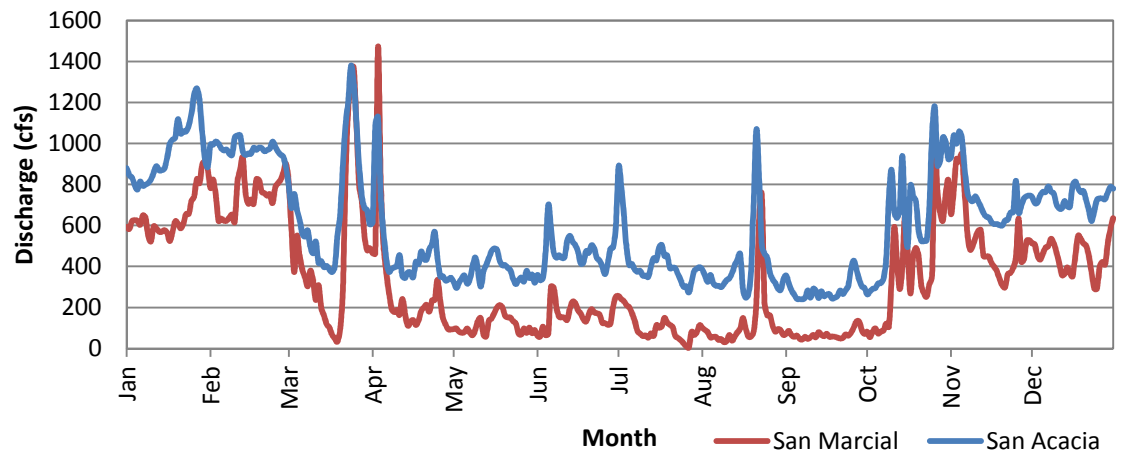
Figure B.11 2000 Daily Discharge Data
