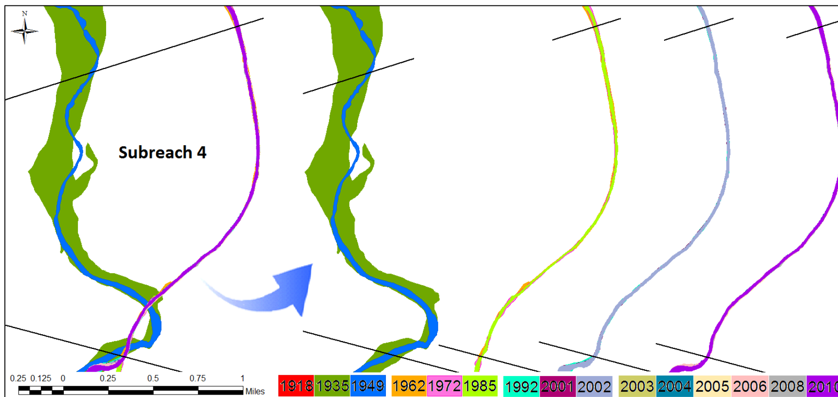
Figure 4.5 Subreach 4 Channel Planforms from Aerial Photography
