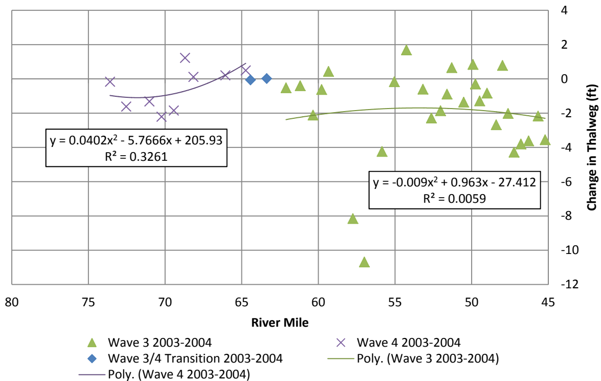
Figure G.11 2003-2004 Thalweg Change
