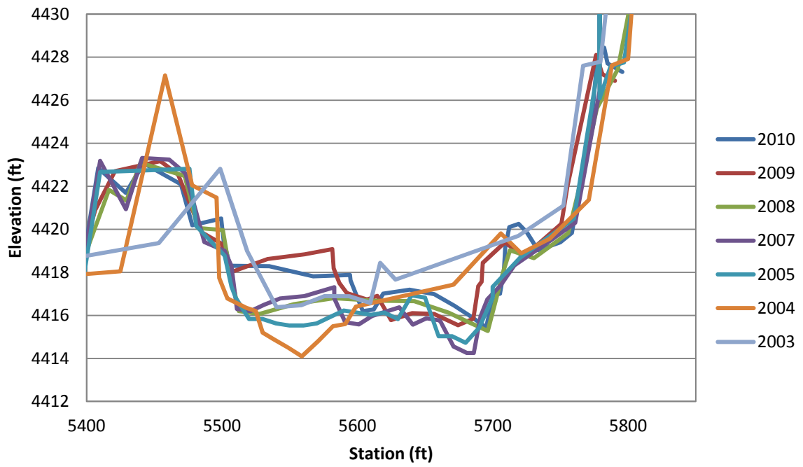
Figure F.32 EB-36 Cross-Section
