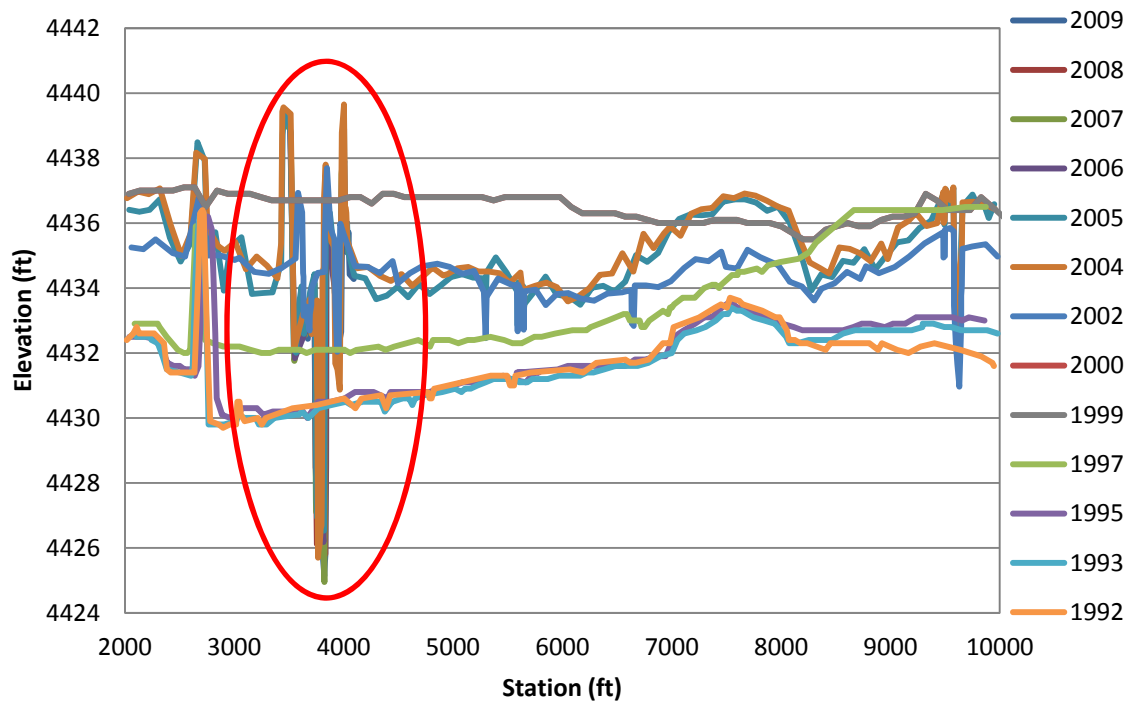
Figure F.27 EB-30 (w/Floodplain) Cross-Section
