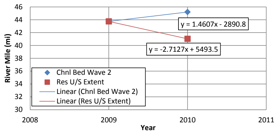
Figure 4.48 Rate of Wave 1 Propagation Upstream
