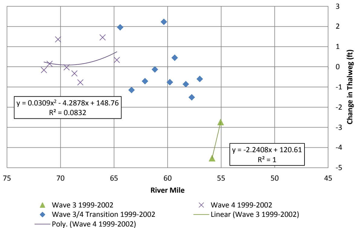
Figure G.9 1999-2002 Thalweg Change
