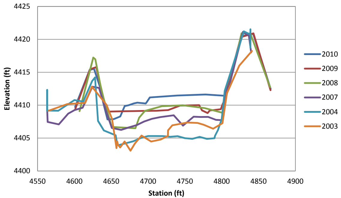
Figure F.37 EB-40 Cross-Section
