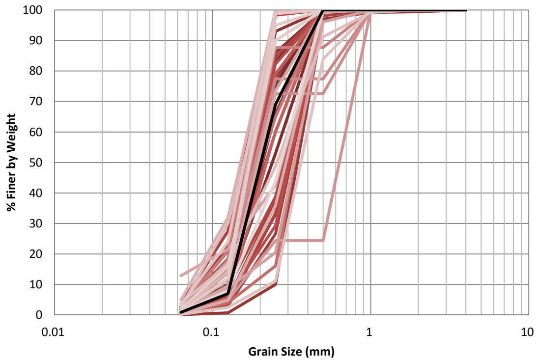
Figure H.10 EB-10 1992 Grain Size Distribution
