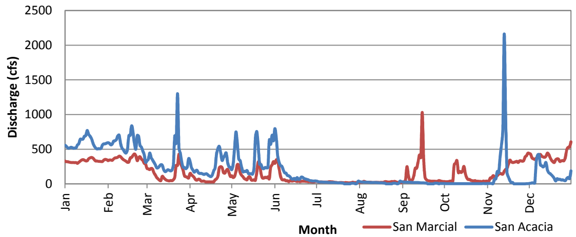
Figure B.14 2003 Daily Discharge Data
