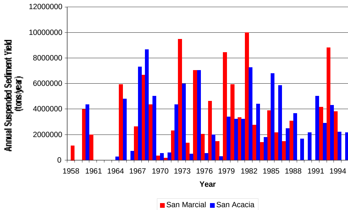
Figure 2.15: Annual Suspended Sediment Yield at San Acacia and San Marcial Gauges
