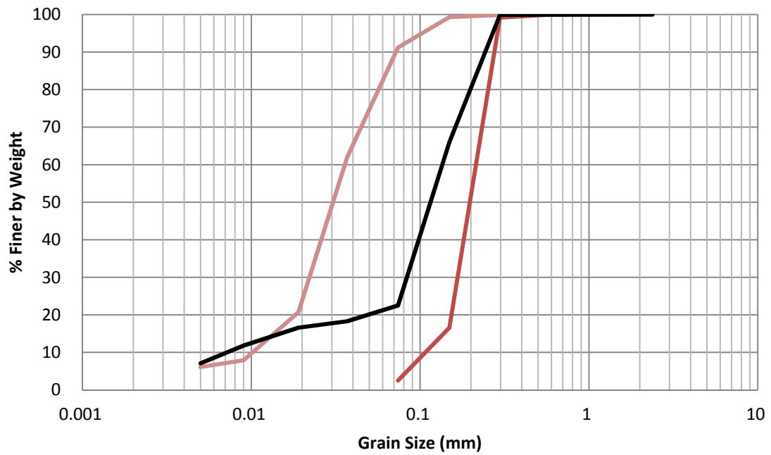
Figure H.19 EB-13 1988 Grain Size Distribution
