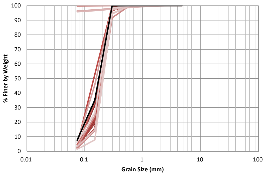
Figure H.7 EB-10 1987 Grain Size Distribution
