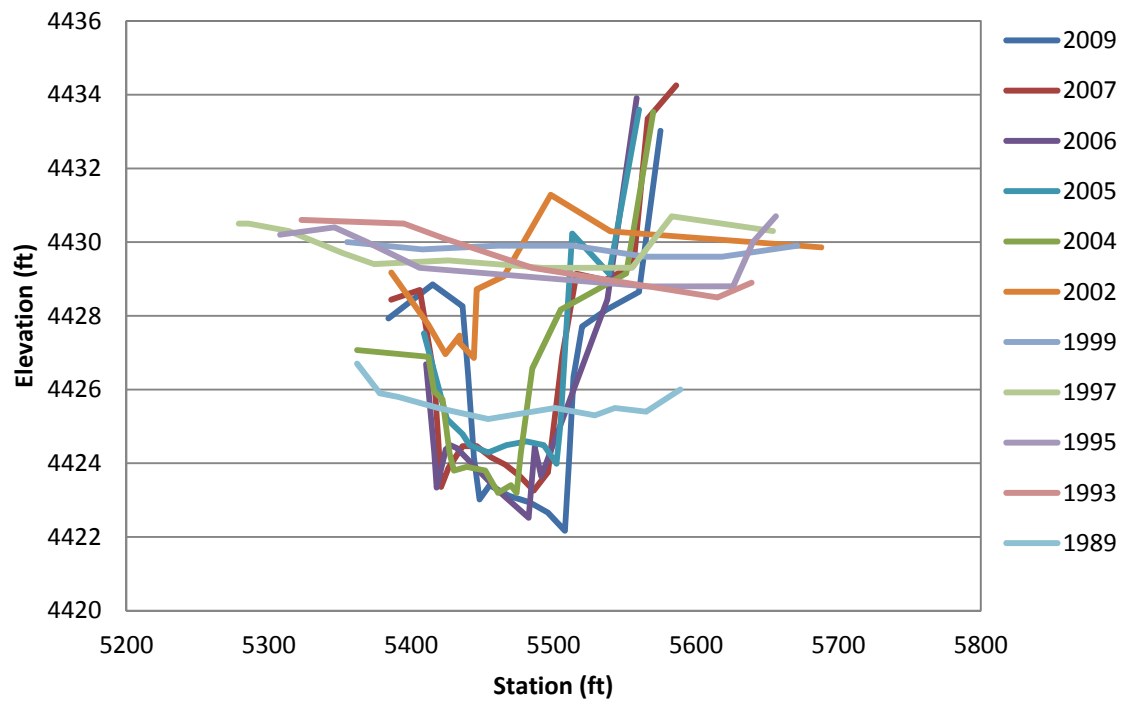
Figure F.28 EB-32 Cross-Section
