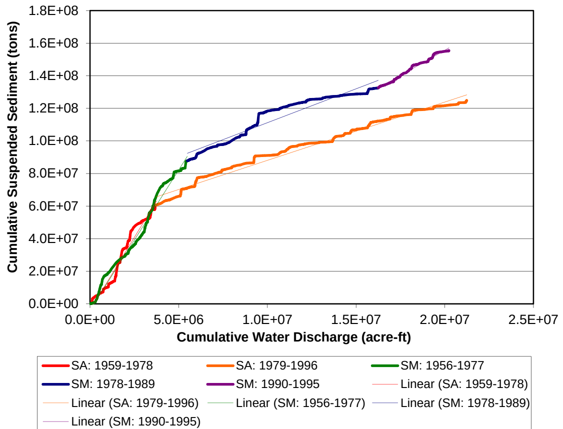
Figure 4.68 Suspended Sediment Concentration Double Mass Curves (Larsen et al. 2007)
