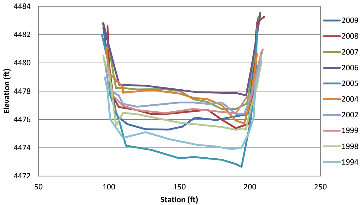
Figure F.6 SO-1692 Cross-Section
