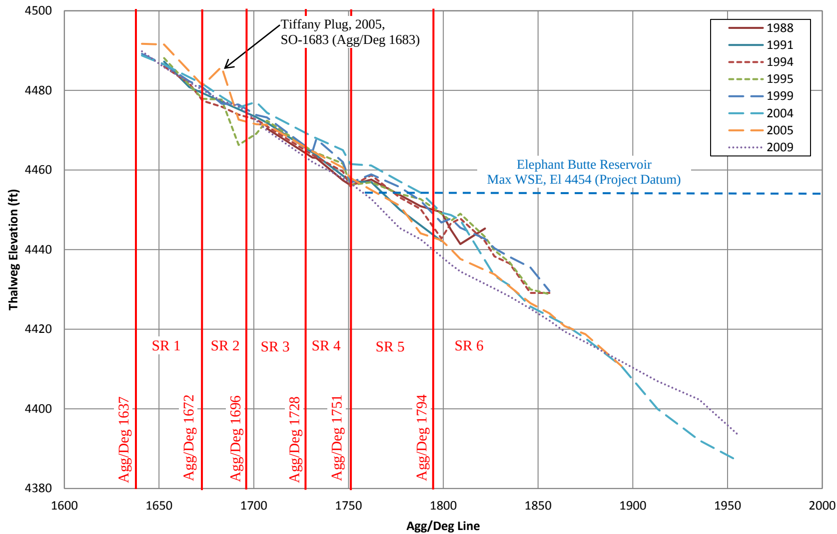
Figure 4.21 Thalweg Elevation Profile From Range Line Survey Data
