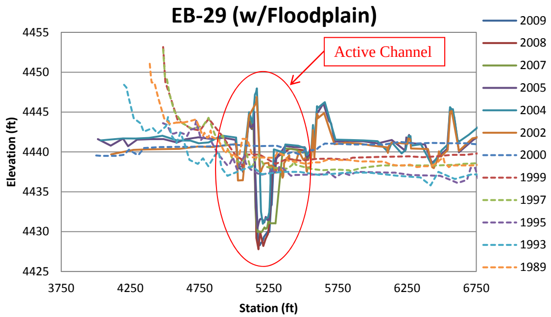
Figure 4.35 Subreach 6: EB-29 (w/Floodplain) Surveyed Cross-Sections
