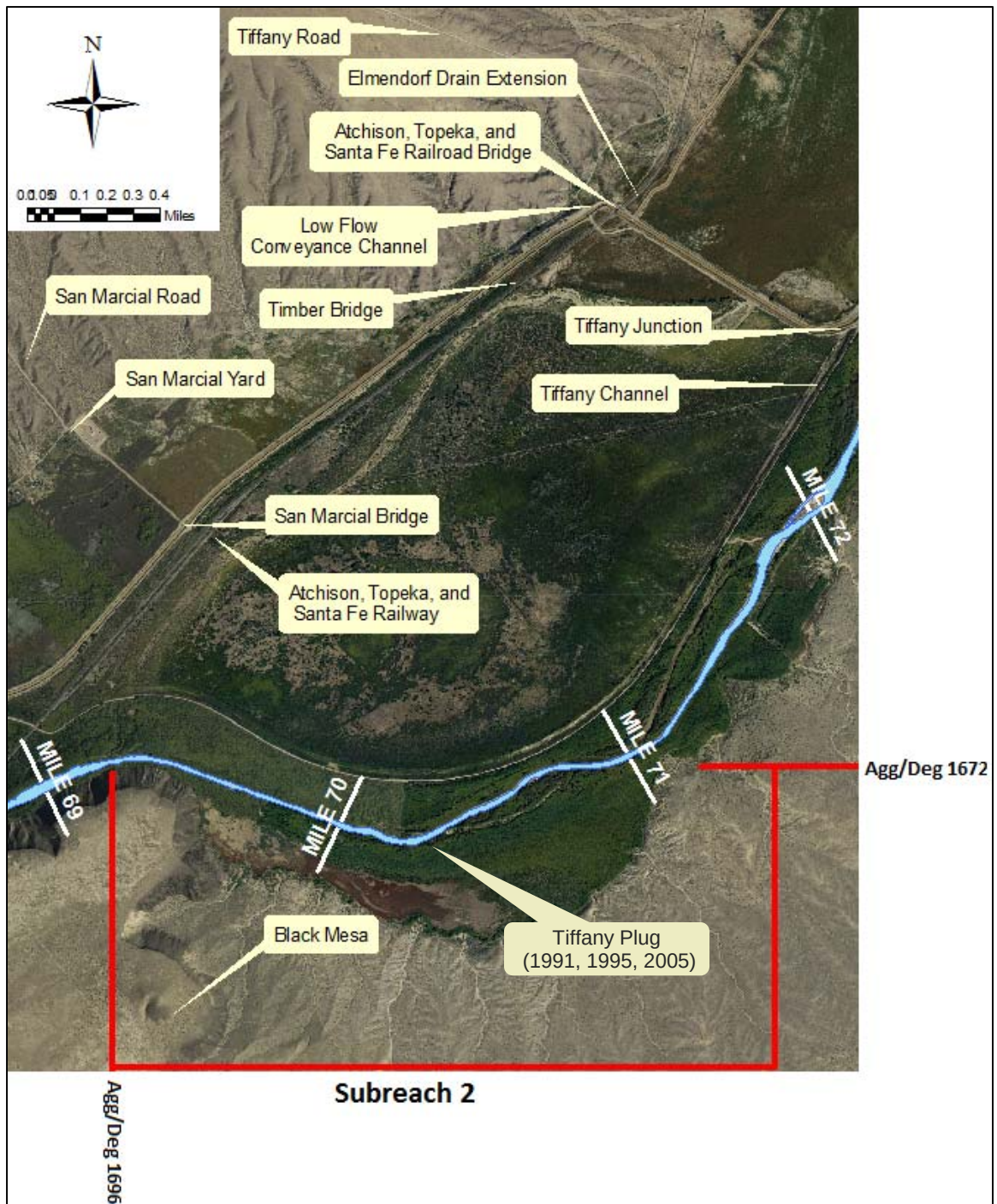
Figure 2.4 2008 Aerial Photo of Subreach 2
