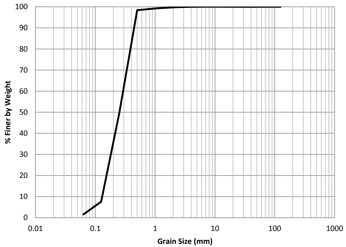
Figure H.31 EB-18 2002 Grain Size Distribution
