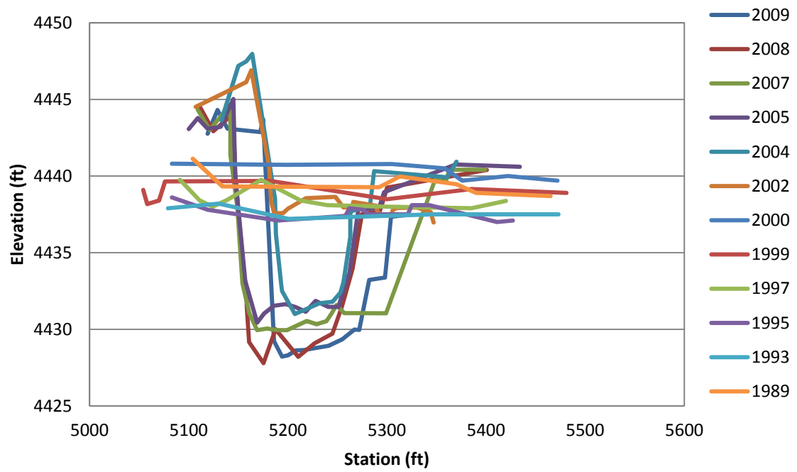
Figure F.24 EB-29 Cross-Section
