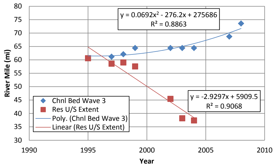
Figure 4.52 Rate of Wave 3 Propagation Upstream
