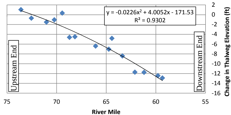
Figure 4.45 Magnitude of Degradation from 2004 to 2009
