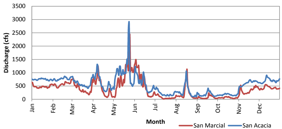
Figure B.12 2001 Daily Discharge Data
