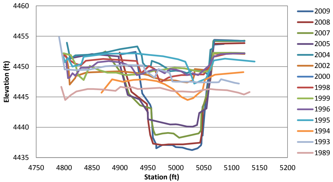
Figure F.18 EB-25 Cross-Section
