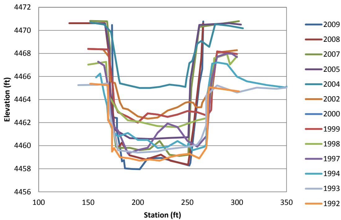
Figure F.12 EB-16 Cross-Section
