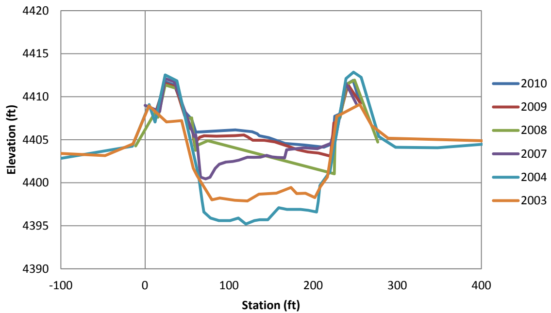
Figure F.41 EB-43 Cross-Section
