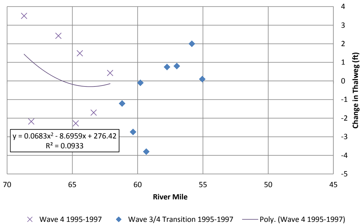
Figure G.6 1995-1997 Thalweg Change
