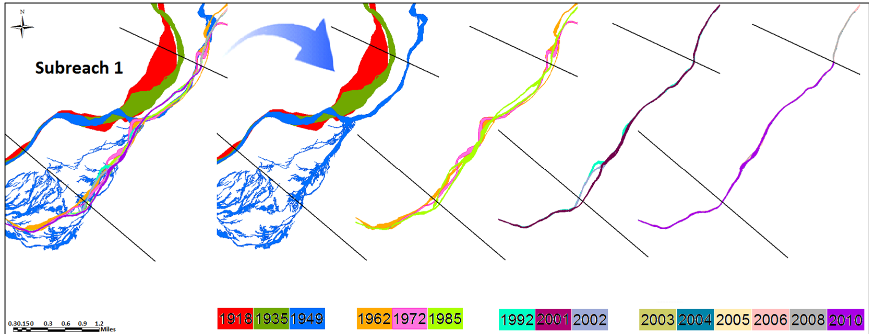
Figure 4.2 Subreach 1 Channel Planforms from Aerial Photography
