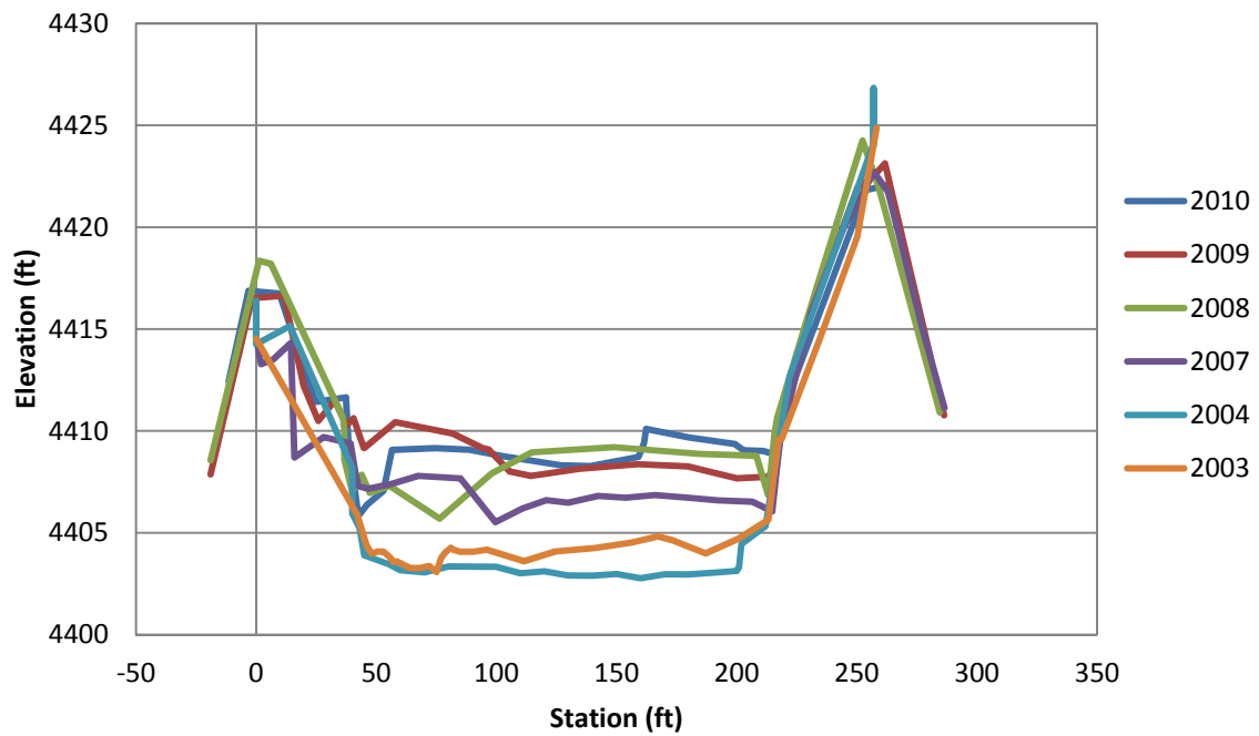
Figure F.38 EB-40.5 Cross-Section
