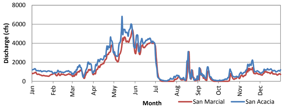
Figure B.5 1994 Daily Discharge Data
