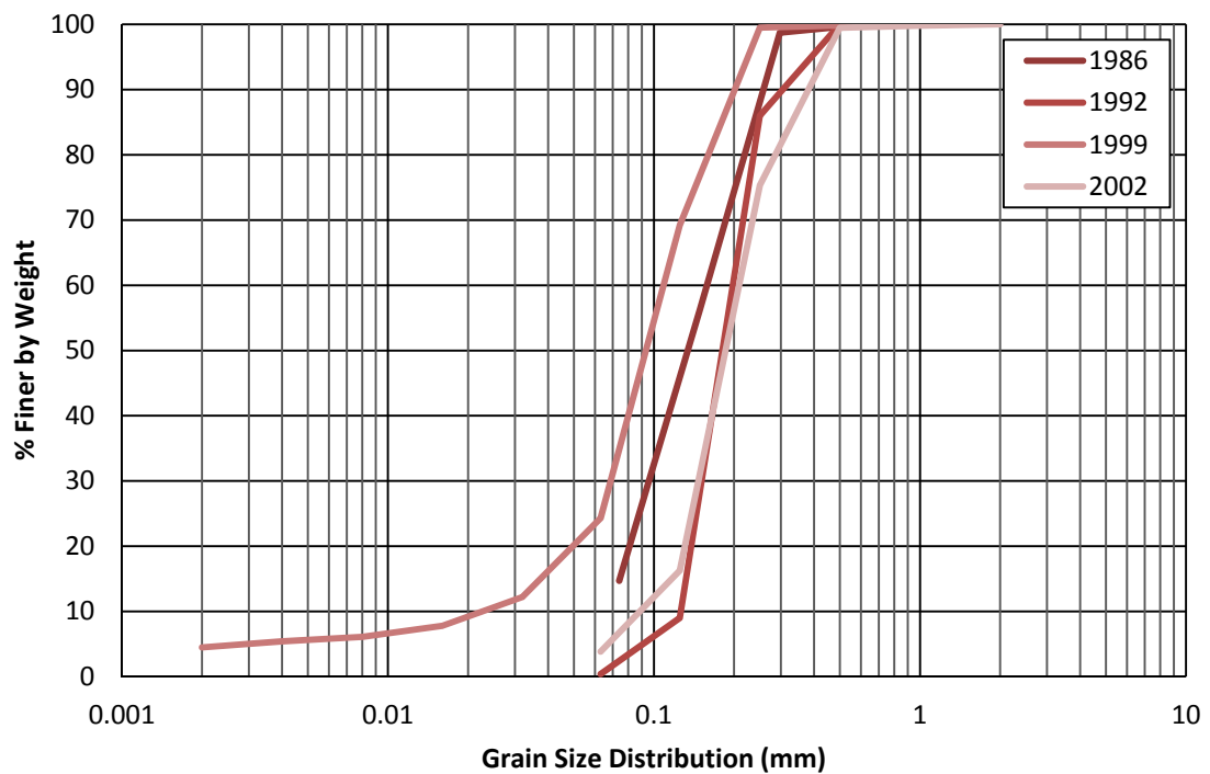
Figure 4.63 Subreach 6 (EB-24): Annual Bed Material Grain Size Distributions
