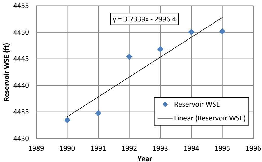
Figure 4.53 Reservoir Water Surface Elevation Change from 1990-1995 Resulting in Wave 4 Channel Aggradation
