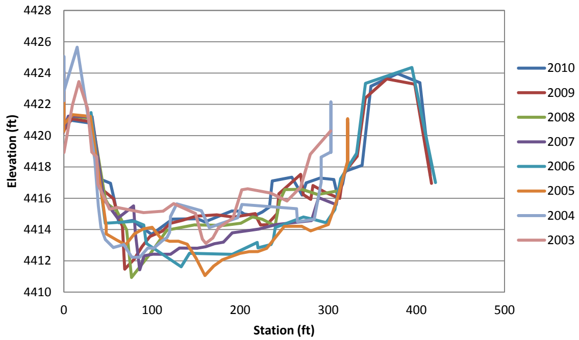
Figure F.34 EB-37.5 Cross-Section
