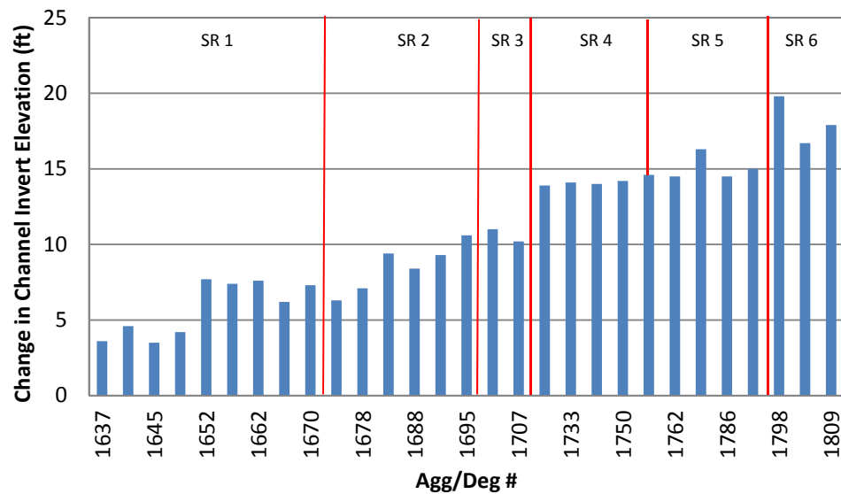
Figure 4.16 Change in Channel Thalweg Elevation (1972 – 1992) Based on Agg/Deg Surveys
