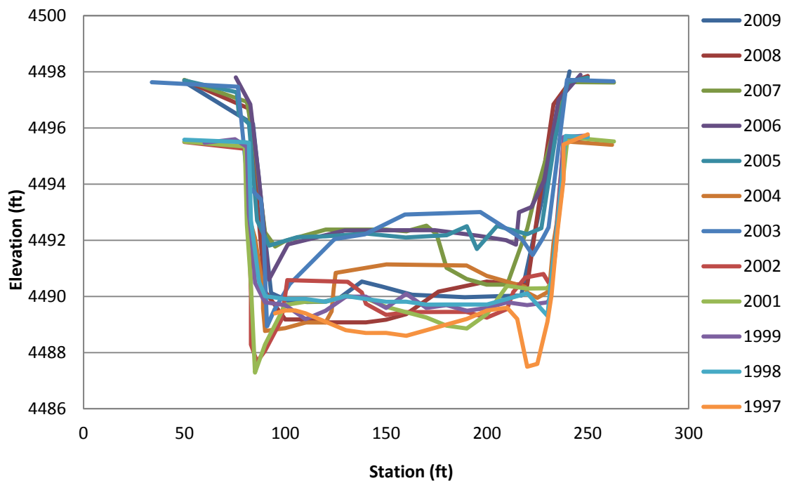
Figure F.1 SO-1641 Cross-Section
