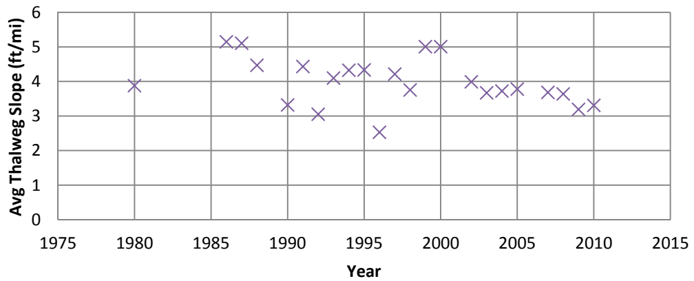
Figure 4.25 Subreach 4 Average Channel Thalweg Slope: Temporal Trend
