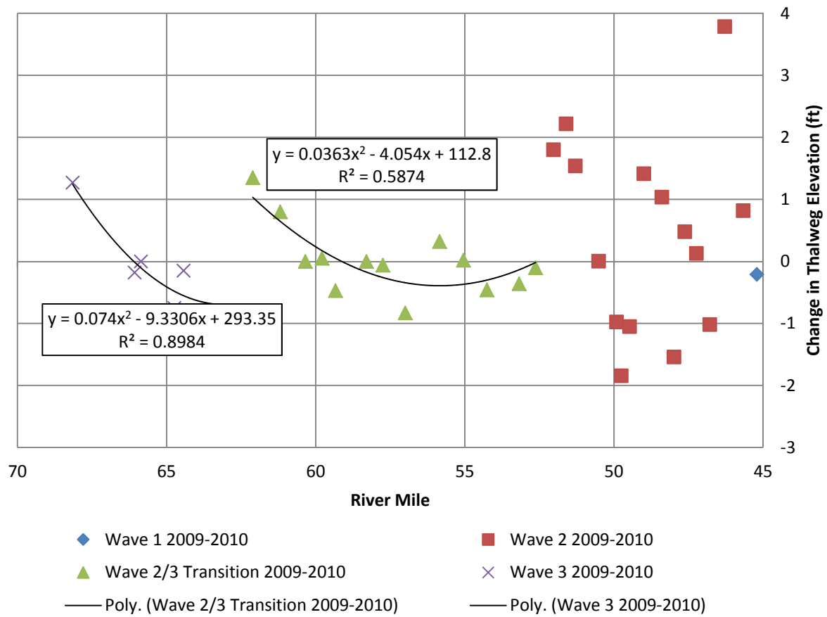
Figure G.15 2009-2010 Thalweg Change
