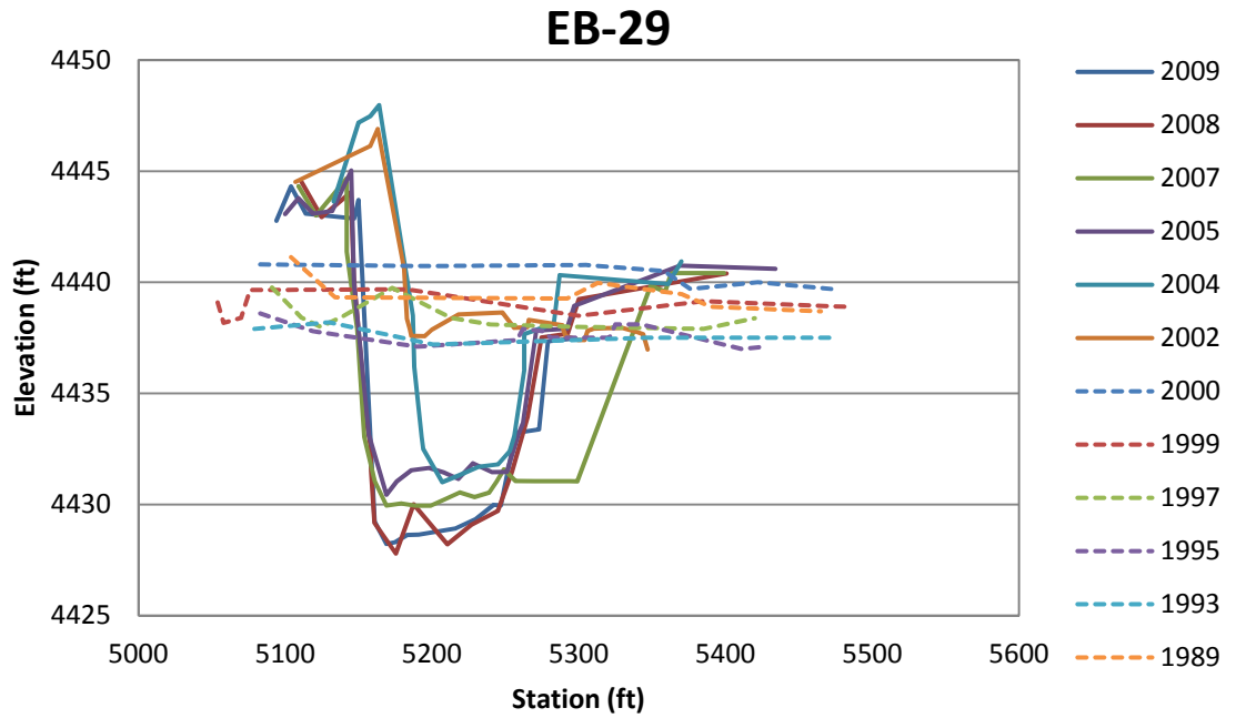
Figure 4.34 Subreach 6: EB-29 Surveyed Cross-Sections
