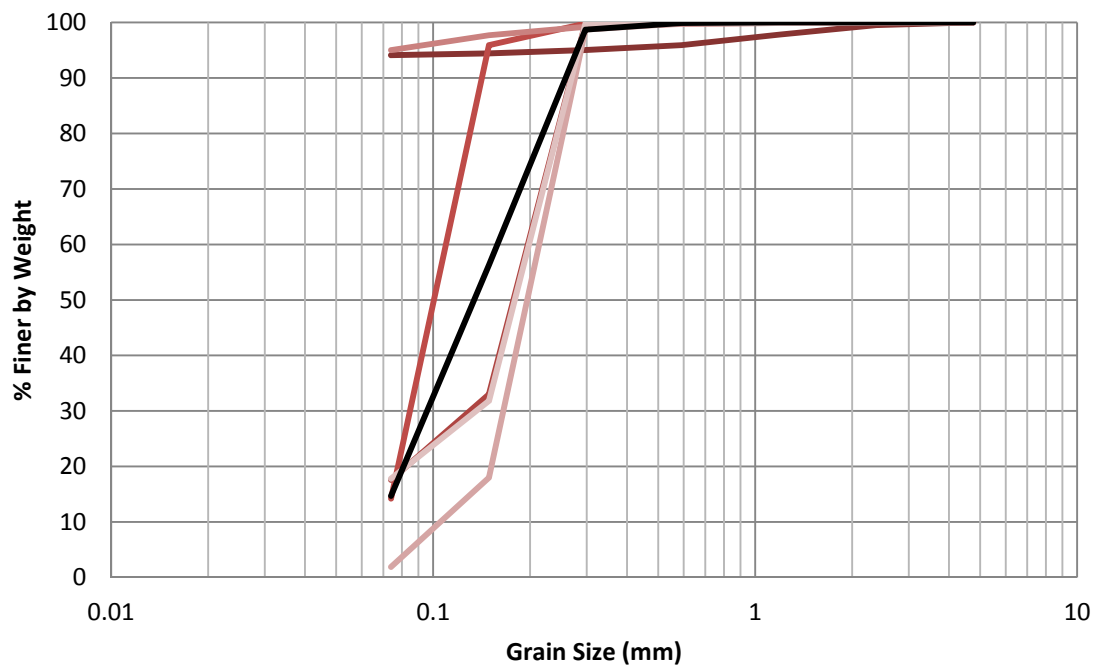
Figure H.32 EB-24 1986 Grain Size Distribution
