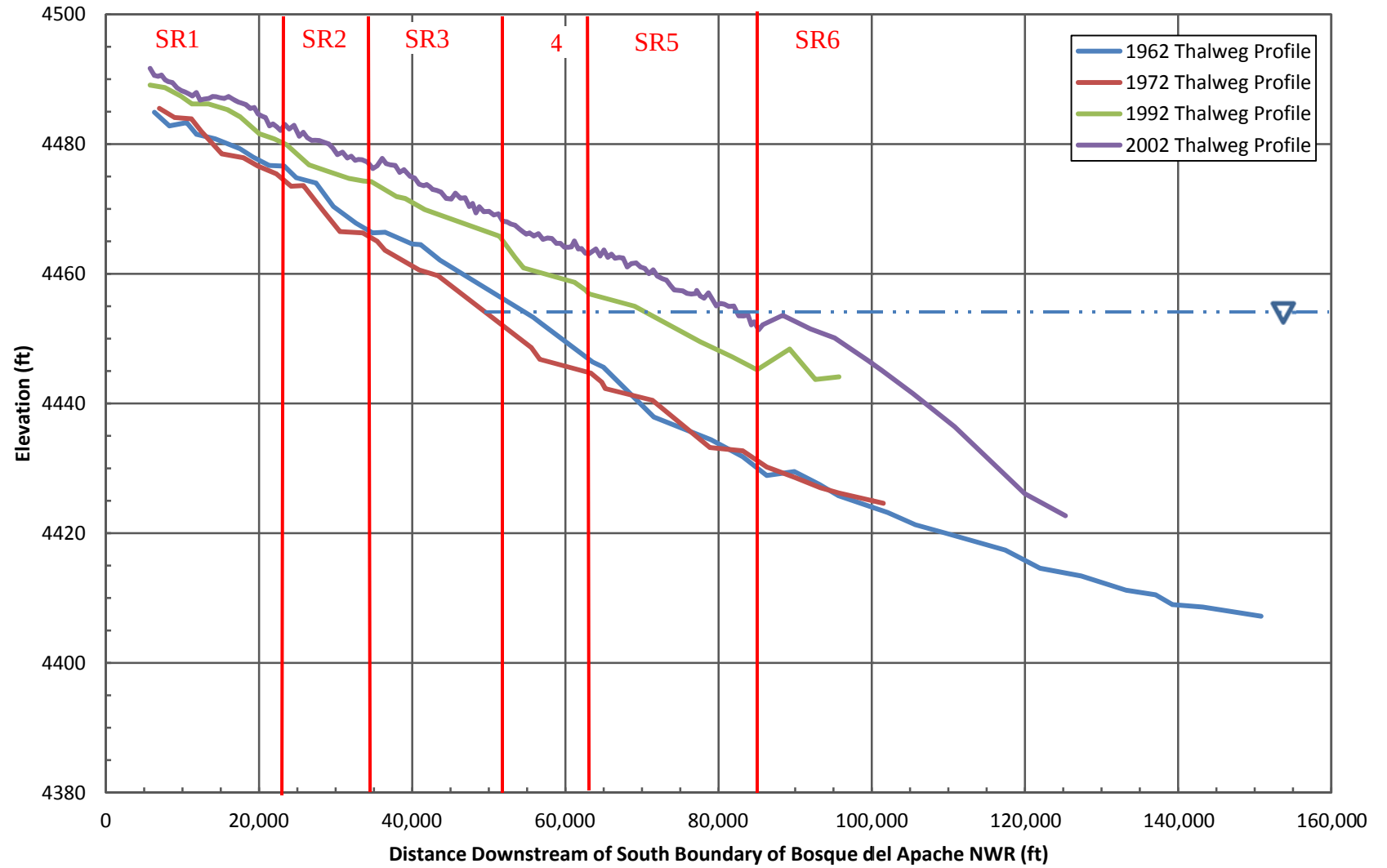
Figure 4.12 Thalweg Elevation Profile From Agg/Deg Surveys
