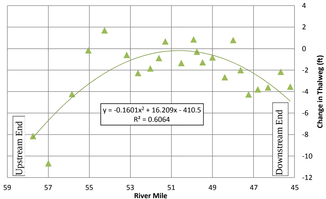
Figure 4.41 Magnitude of Aggradation and Degradation at River Miles (2003-2004)
