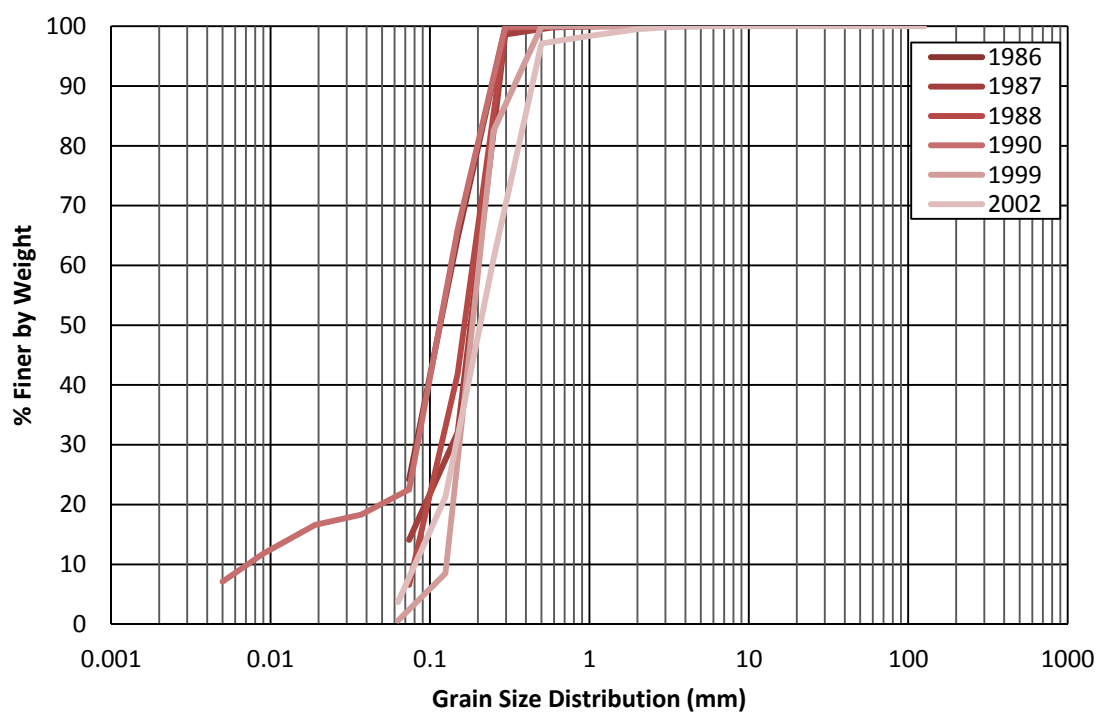
Figure 4.61 Subreach 4 (EB-13): Annual Bed Material Grain Size Distributions
