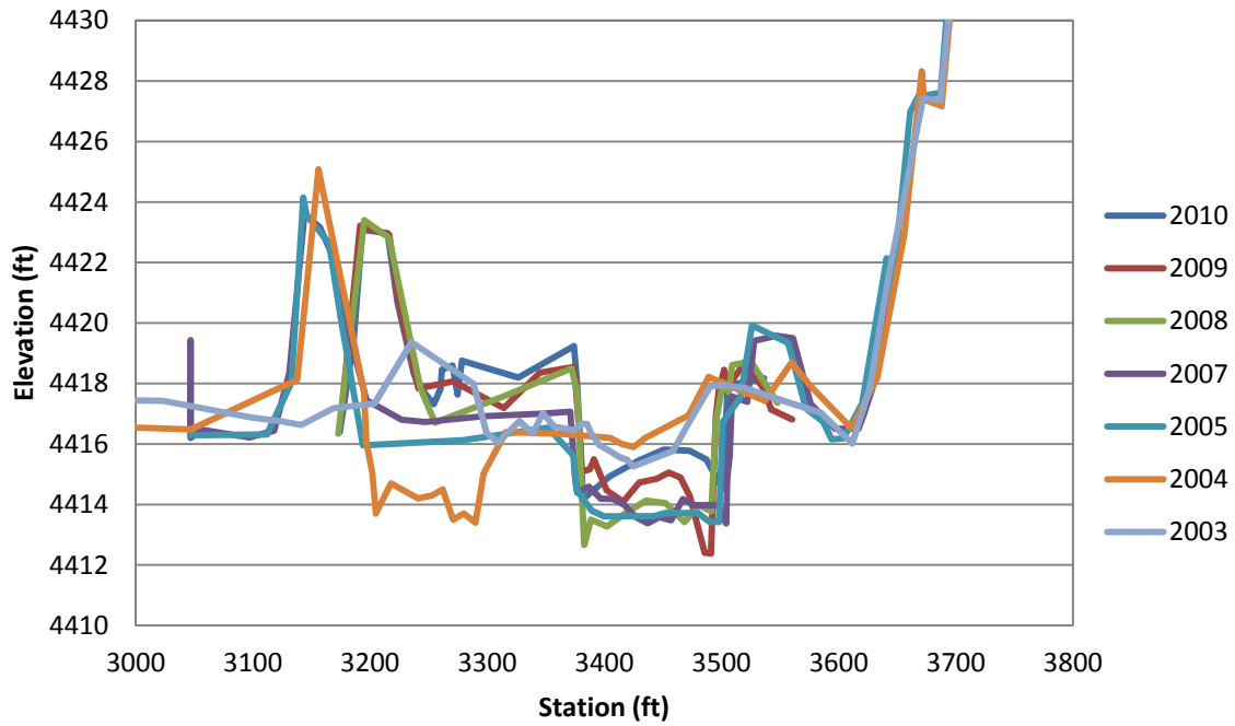
Figure F.33 EB-37 Cross-Section
