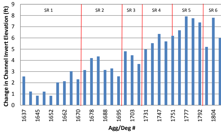
Figure 4.17 Change in Channel Thalweg Elevation from 1992 – 2002 Based on Agg/Deg Surveys
