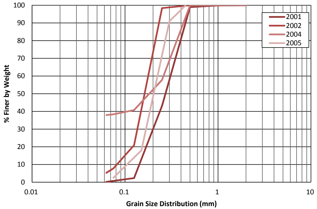
Figure 4.58 Subreach 1 (SO-1641): Annual Bed Material Grain Size Distributions
