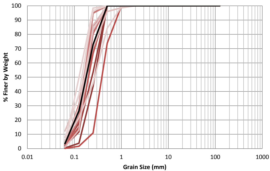
Figure H.27 EB-18 1993 Grain Size Distribution
