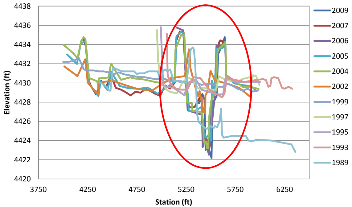
Figure F.29 EB-32 (w/Floodplain) Cross-Section
