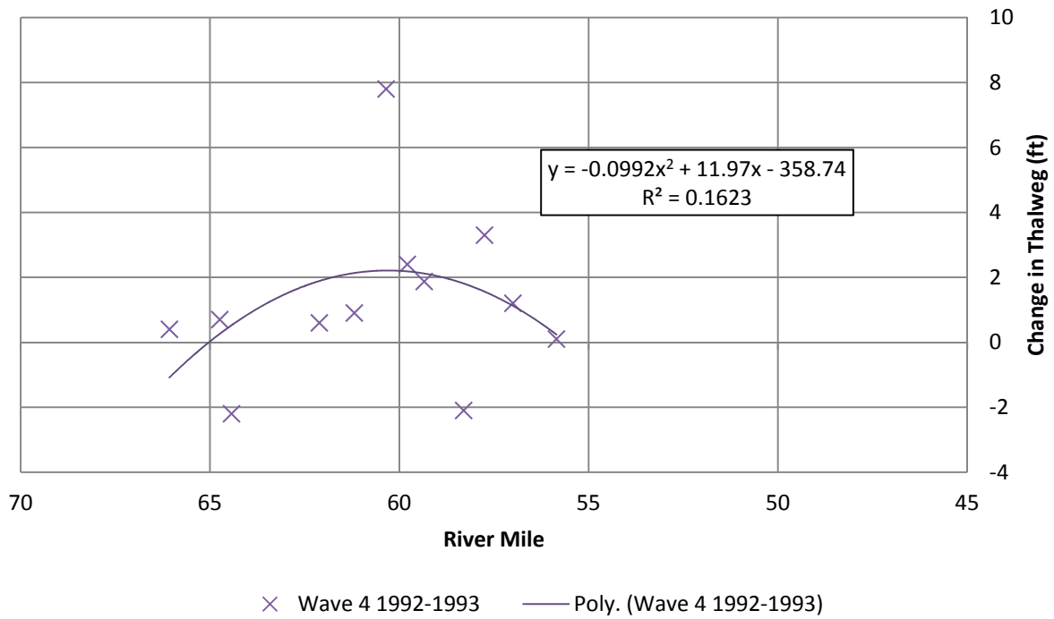
Figure G.3 1992-1993 Thalweg Change
