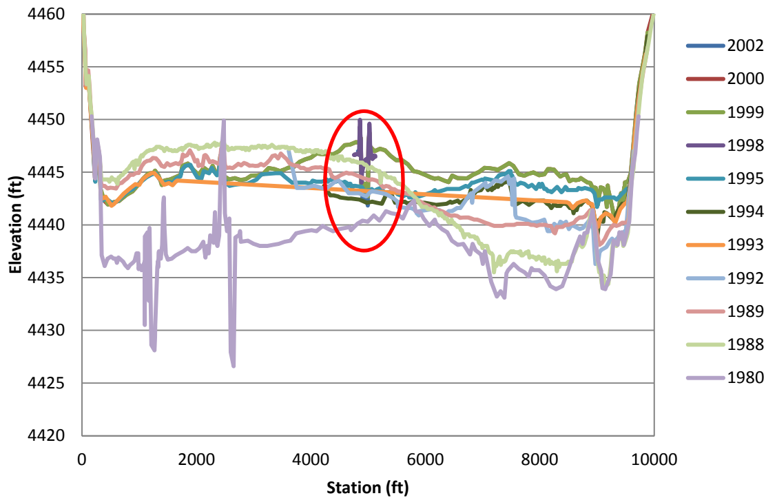
Figure F.21 EB-27 (w/Floodplain) Cross-Section
