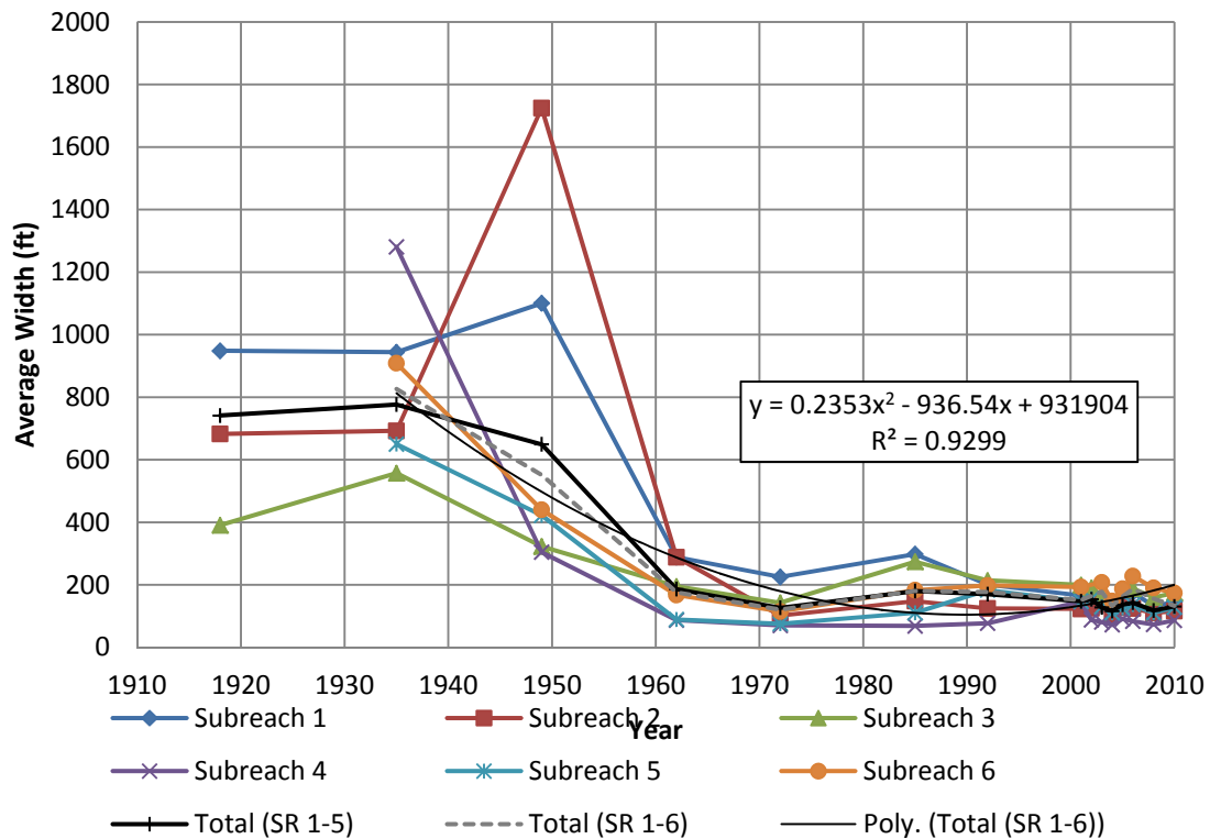
Figure 4.8 Channel Widths from GIS (1918 - 2010)
