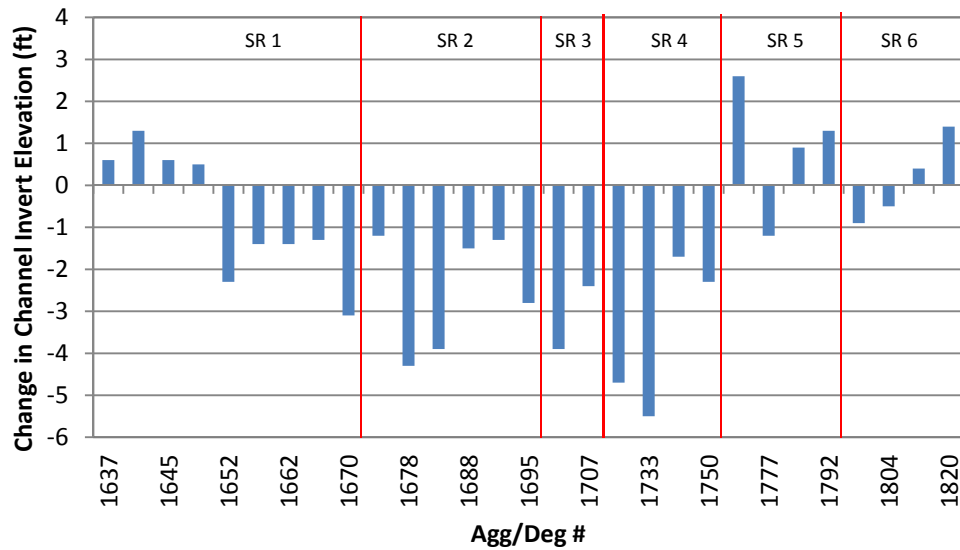
Figure 4.15 Change in Channel Thalweg Elevation (1962 – 1972) Based on Agg/Deg Surveys
