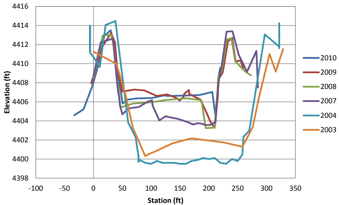
Figure F.40 EB-42 Cross-Section
