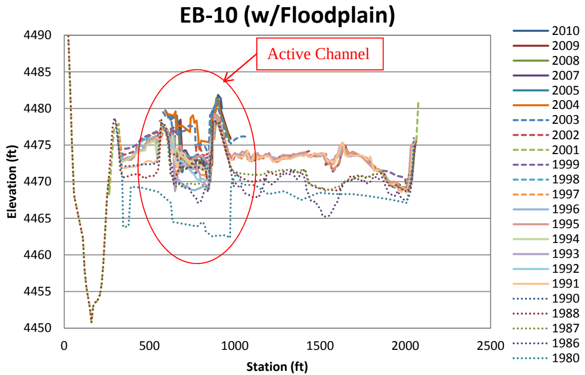
Figure 4.31 Subreach 3: EB-10 (w/Floodplain) Surveyed Cross-Sections
