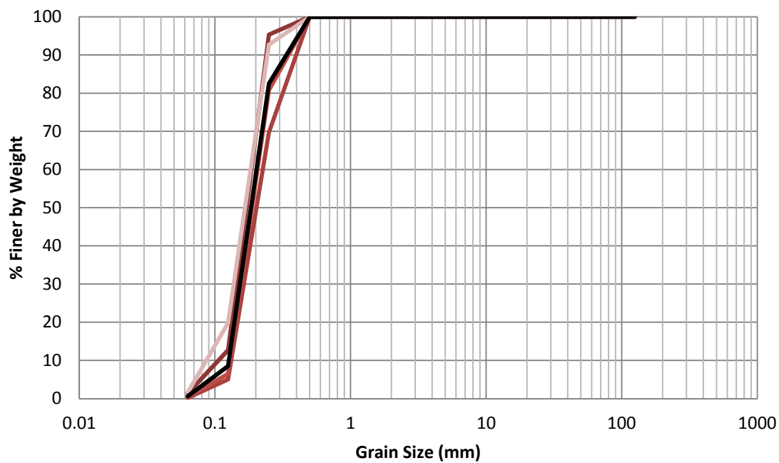
Figure H.21 EB-13 1999 Grain Size Distribution
