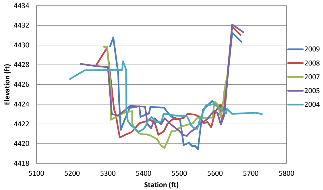
Figure F.30 EB-33 Cross-Section
