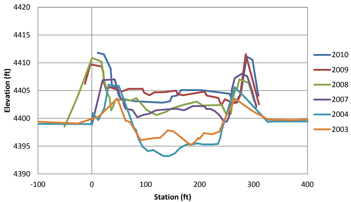
Figure F.43 EB-45 Cross-Section
