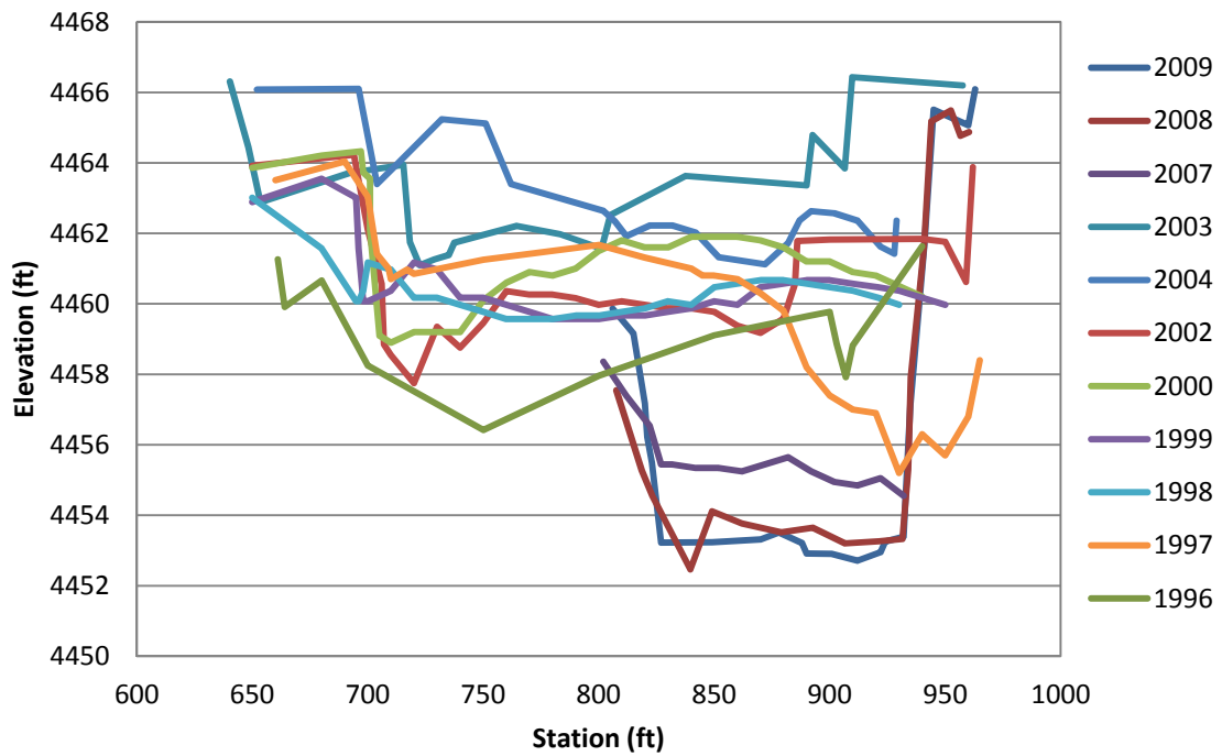
Figure F.14 EB-18 Cross-Section
