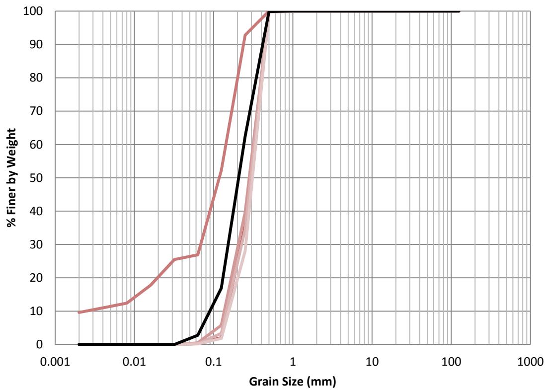
Figure H.29 EB-18 1997 Grain Size Distribution
