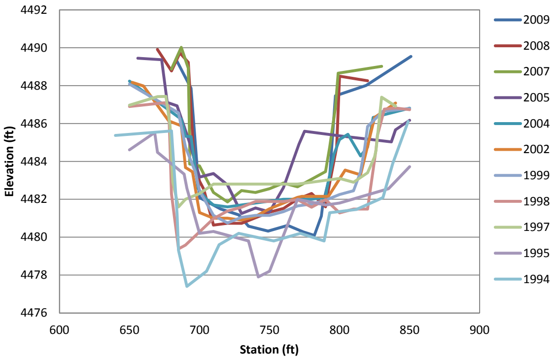
Figure F.4 SO-1673 Cross-Section
