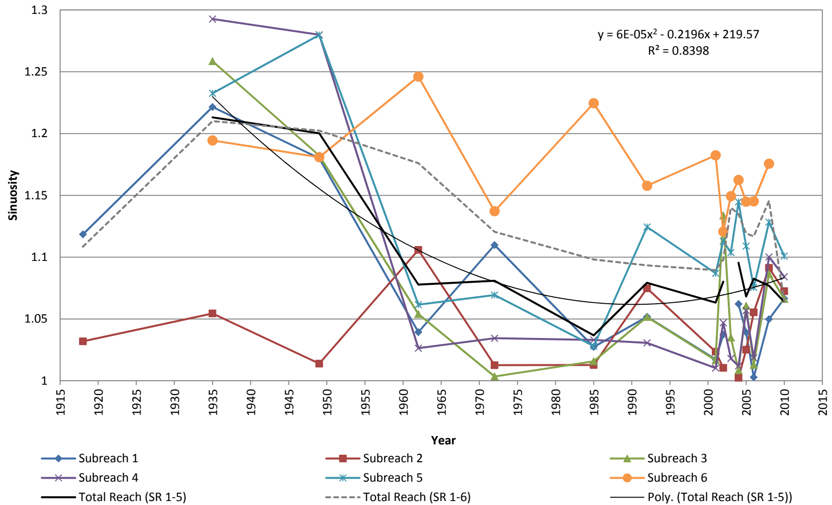
Figure 4.11 Temporal Sinuosity Trends
