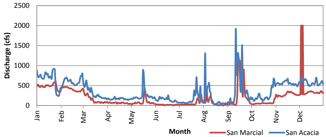
Figure B.13 2002 Daily Discharge Data
