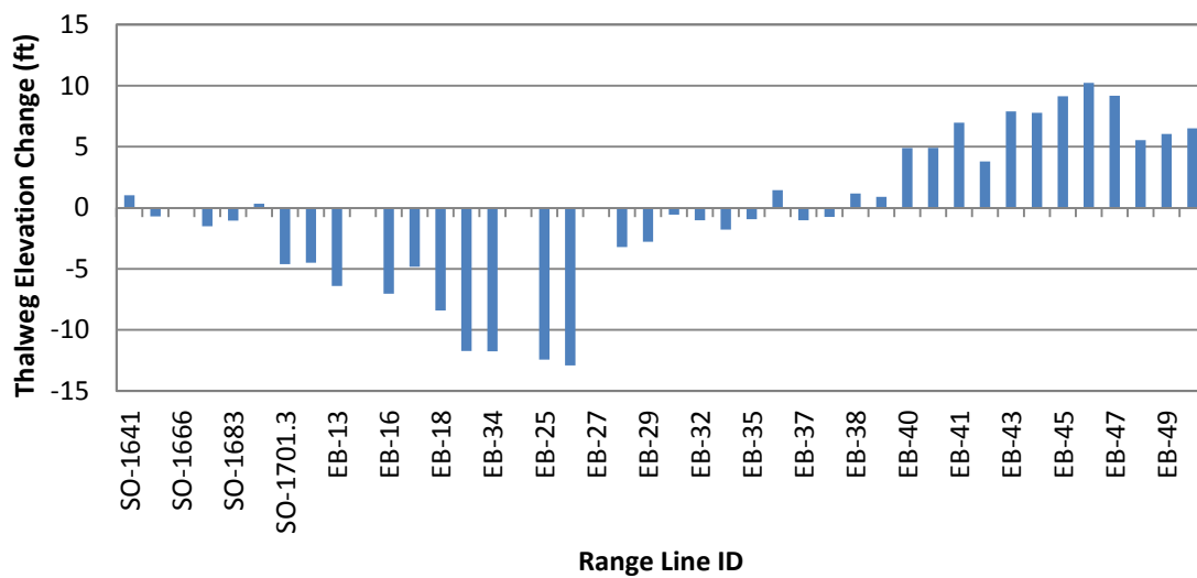
Figure 4.44 Change in Thalweg Elevation from 2004 to 2009
