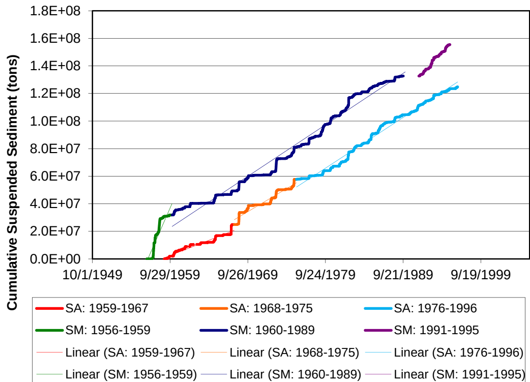
Figure 4.67 Suspended Sediment Discharge Single Mass Curve (Larsen et al. 2007)
