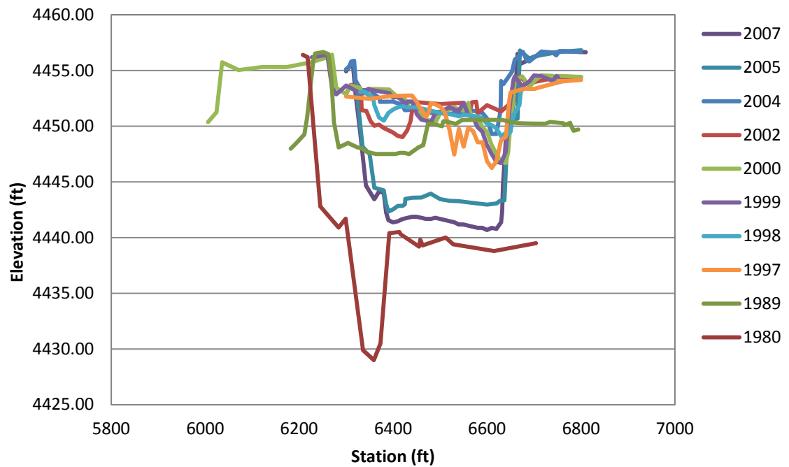
Figure F.17 EB-24 Cross-Section
