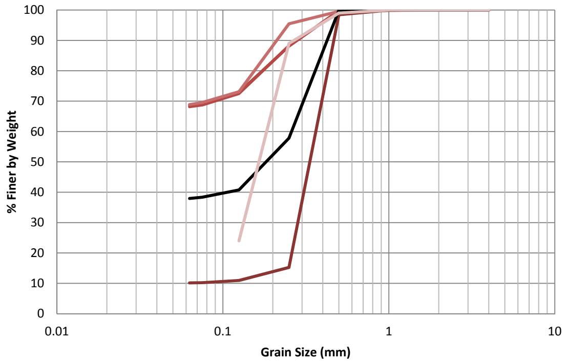
Figure H.3 SO-1641 2004 Grain Size Distribution
