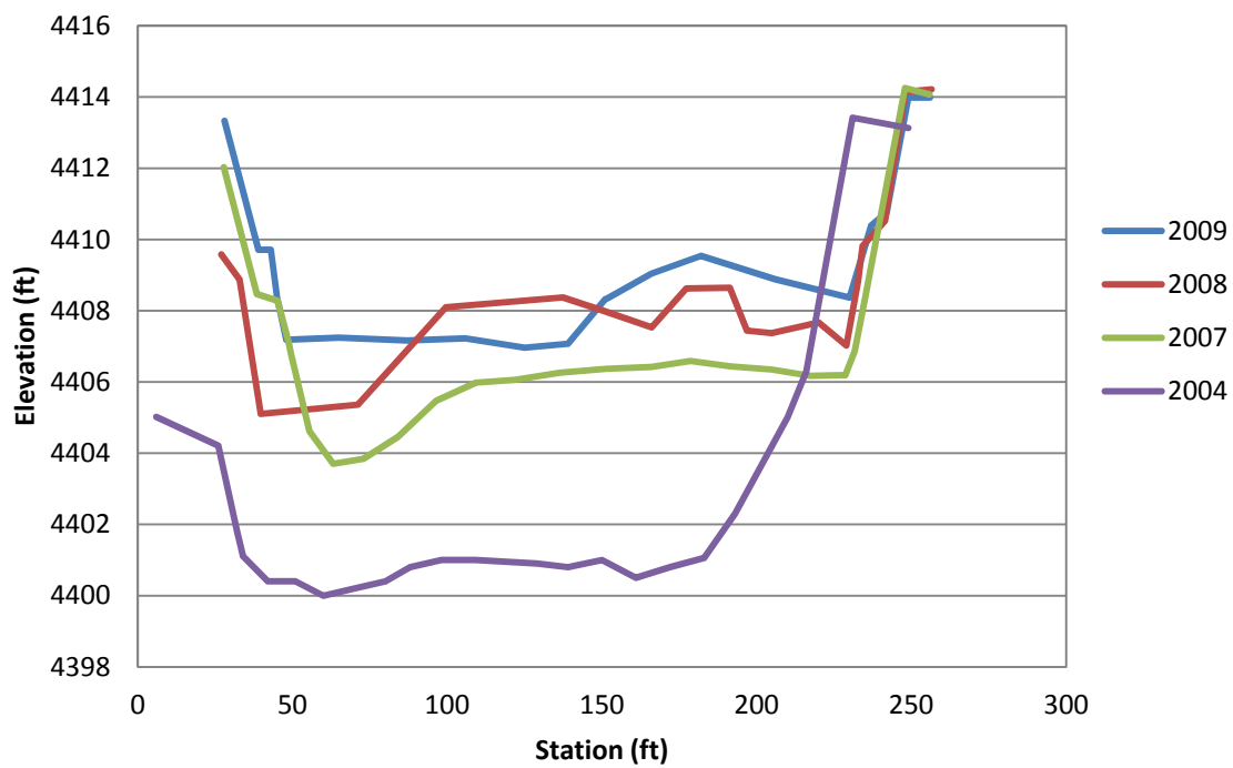
Figure F.39 EB-41 Cross-Section
