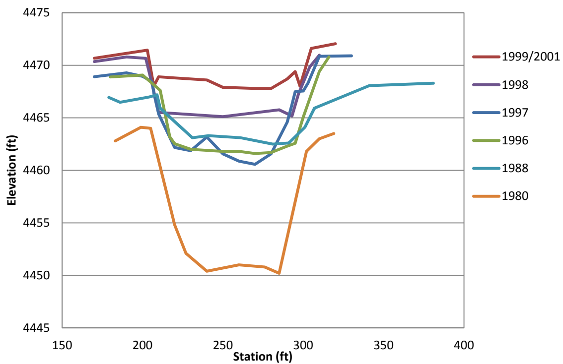
Figure F.11 EB-14 Cross-Section
