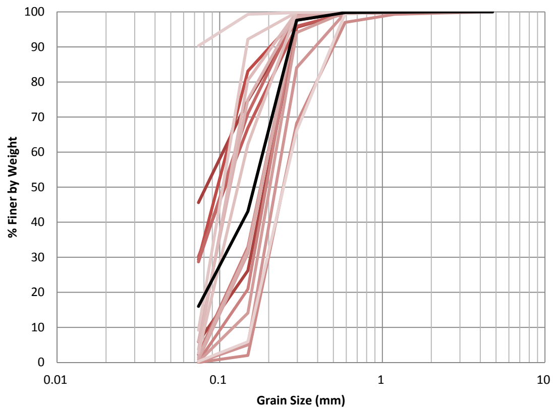
Figure H.6 EB-10 1986 Grain Size Distribution
