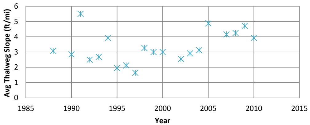
Figure 4.26 Subreach 5 Average Channel Thalweg Slope: Temporal Trend
