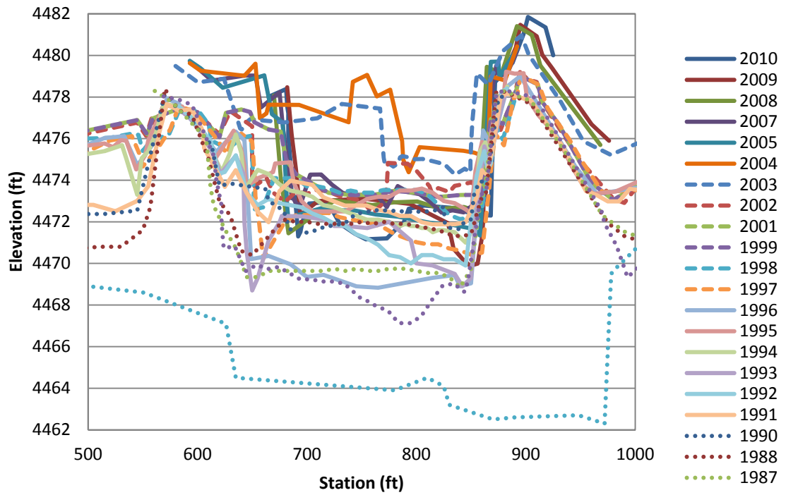
Figure F.8 EB-10 Cross-Section
