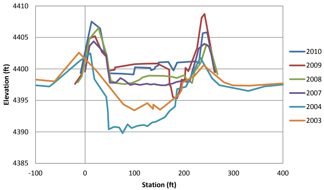
Figure F.46 EB-48 Cross-Section
