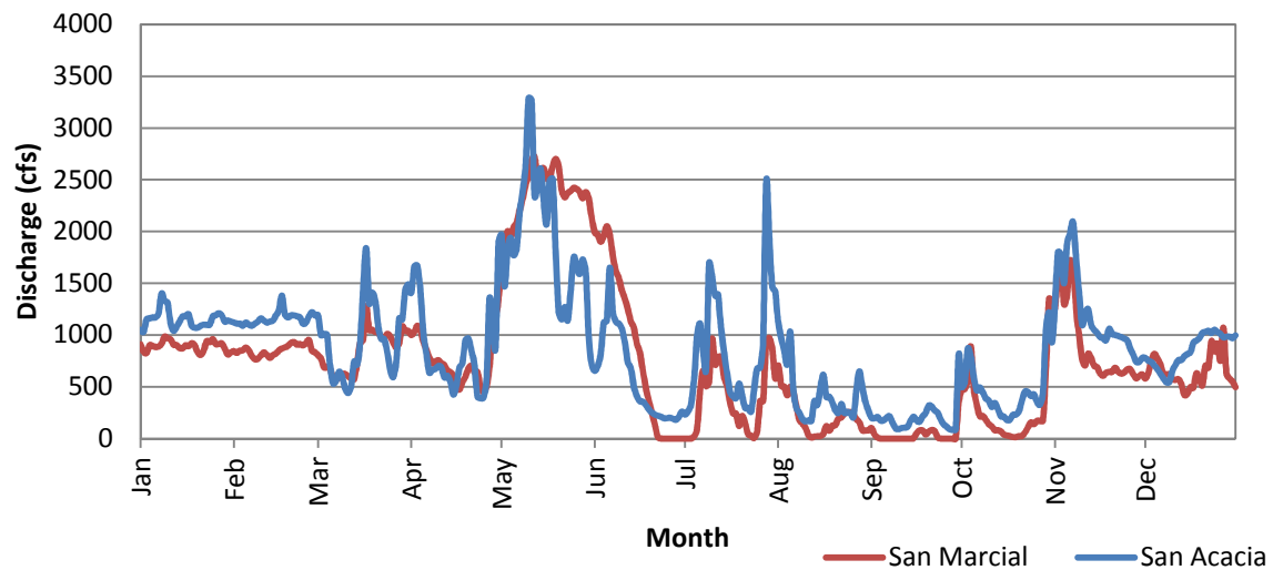
Figure B.9 1998 Daily Discharge Data
