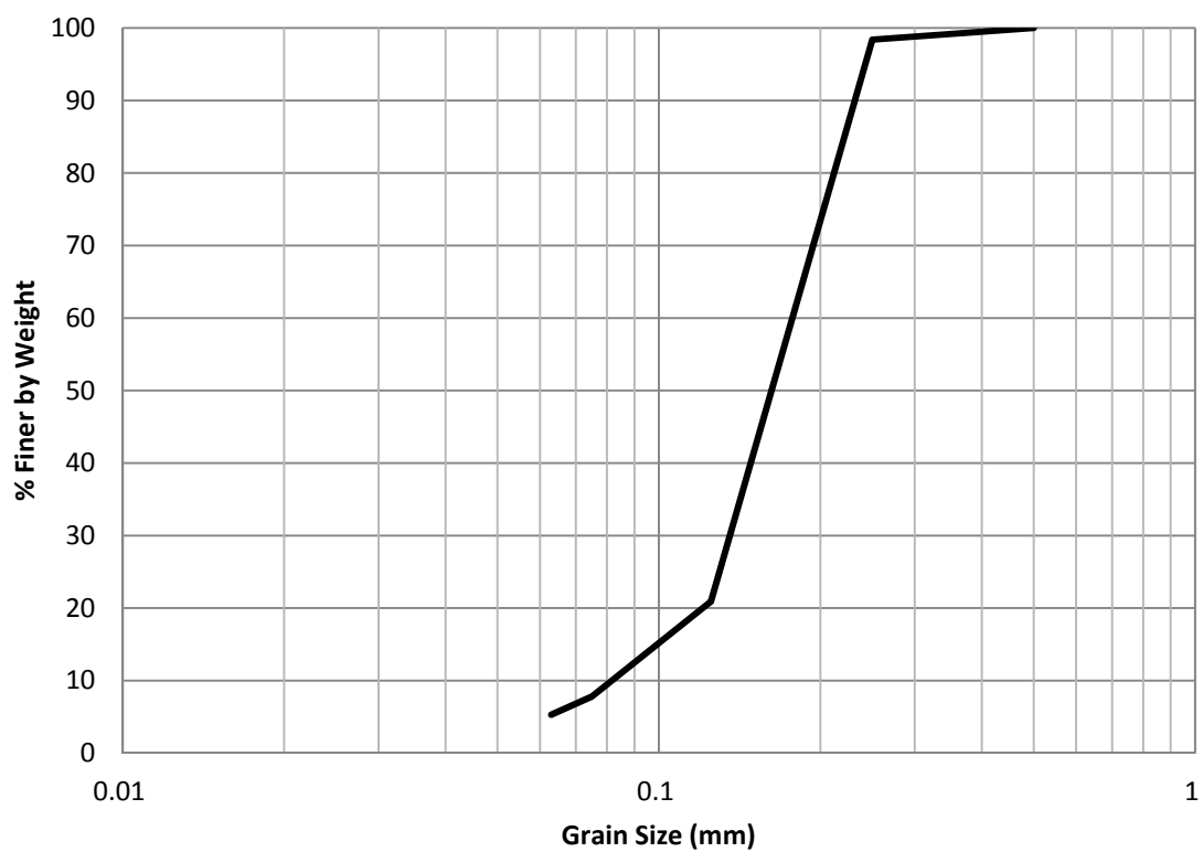
Figure H.1 SO-1641 2001 Grain Size Distribution
