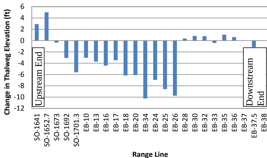
Figure 4.42 Magnitude of Aggradation and Degradation at Range Lines (2004-2005)
