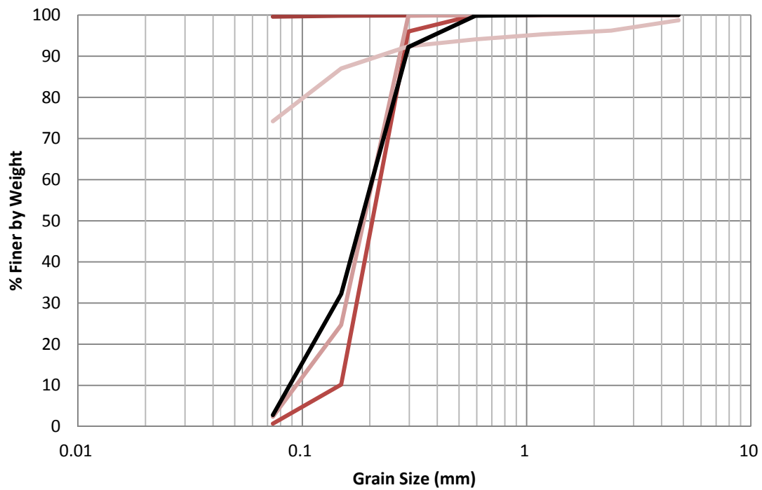
Figure H.8 EB-10 1988 Grain Size Distribution
