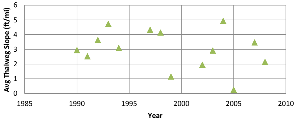
Figure 4.24 Subreach 3 Average Channel Thalweg Slope: Temporal Trend
