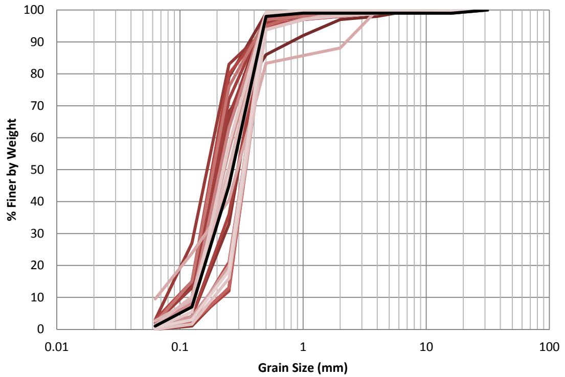
Figure H.12 EB-10 1994 Grain Size Distribution
