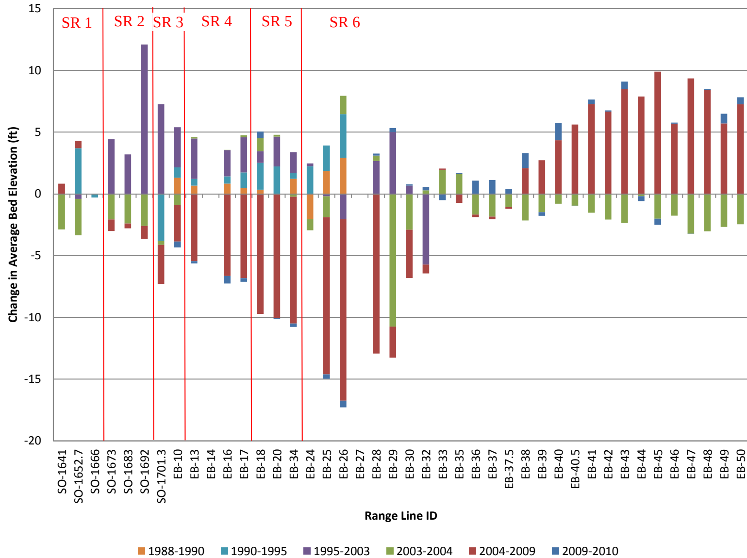
Figure 4.38 Change in Average Channel Bed Elevation at Range Lines (1988-2010)
