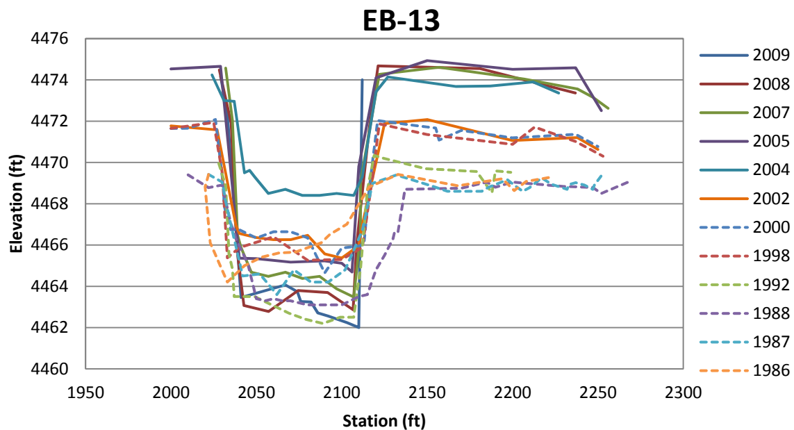
Figure 4.32 Subreach 4: EB-13 Surveyed Cross-Sections
