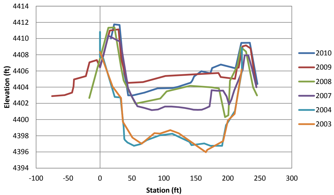
Figure F.42 EB-44 Cross-Section
