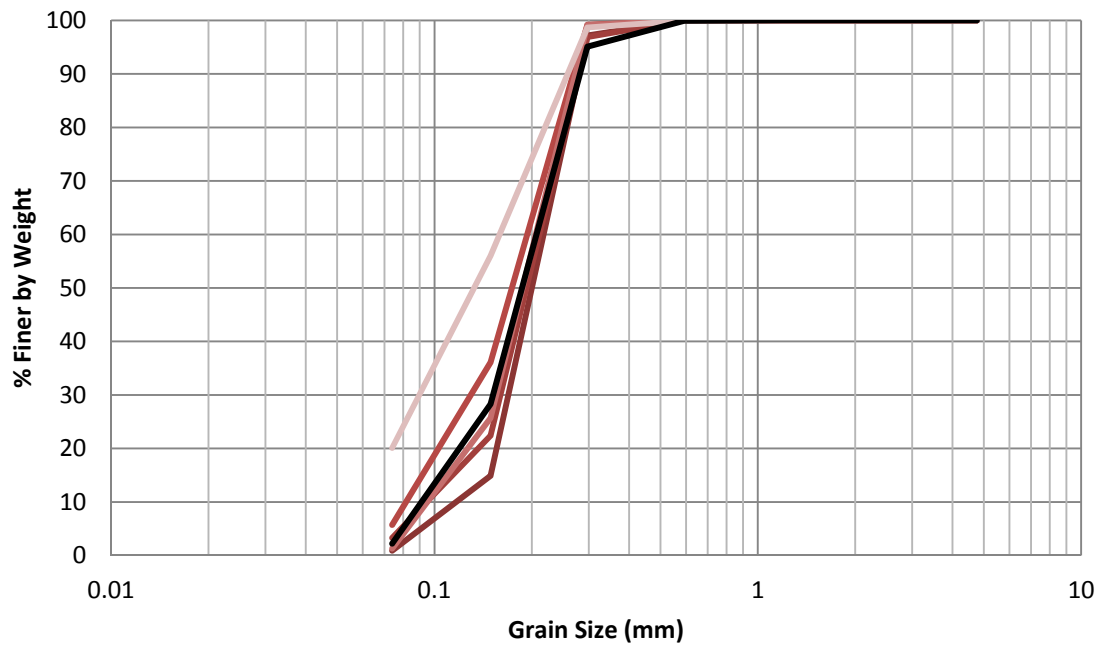
Figure H.25 EB-18 1988 Grain Size Distribution
