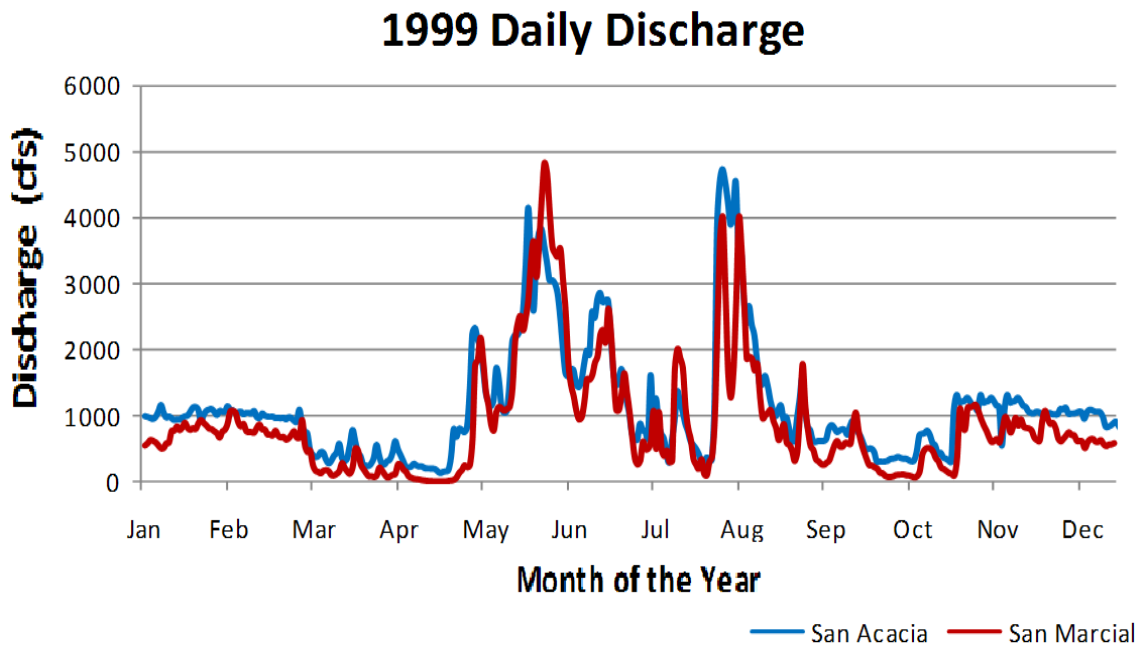
Figure 2.13: Daily Discharge of the Rio Grande in 1999
