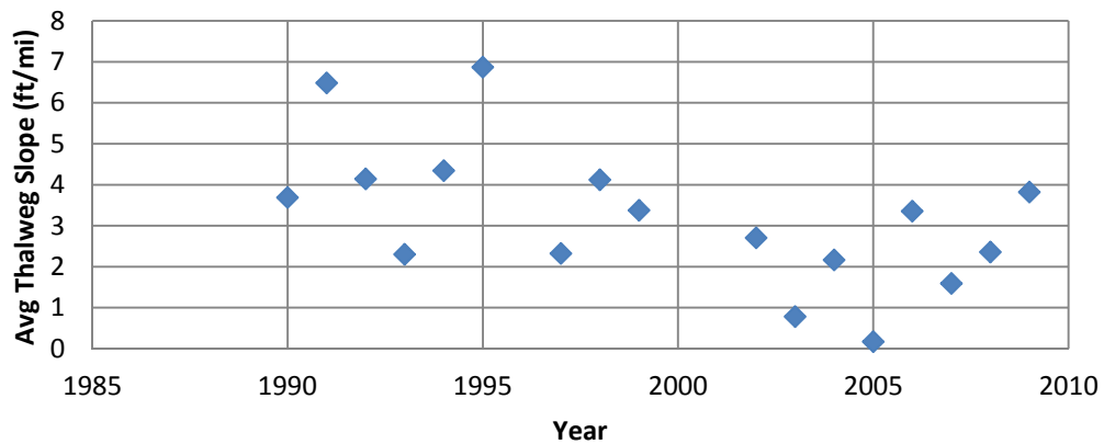
Figure 4.22 Subreach 1 Average Channel Thalweg Slope: Temporal Trend
