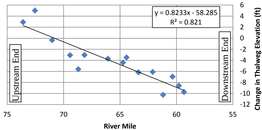
Figure 4.43 Magnitude of Aggradation and Degradation at River Miles (2004 to 2005)
