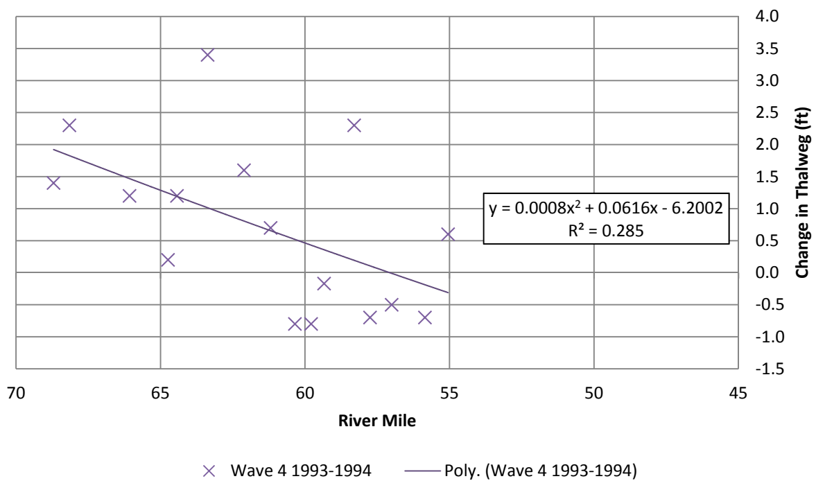
Figure G.4 1993-1994 Thalweg Change
