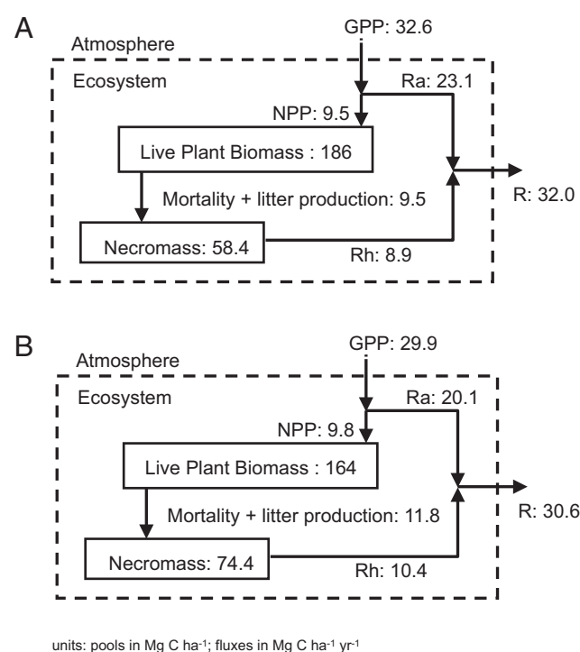
Fig. 4. Carbon pools (boxes, \text{MgC ha}^{-1} ) and fluxes (arrows, \text{MgC}\cdot\text{ha}^{-1}\cdot\text{y}^{-1} ): (A) before logging; and (B) for the 3-y period following logging (Table S3). Carbon pools include live plant biomass ( 186 \text{ MgC ha}^{-1} ) (34), necromass ( 58.4 \text{ MgC ha}^{-1} ) (53), and soil mineral carbon ( 71 \text{ MgC ha}^{-1} ) (54).
