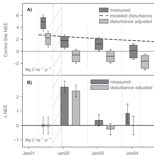
Fig. S2. (A) Averaged NEE ( \text{MgC}\cdot\text{ha}^{-1}\cdot\text{yr}^{-1} ) at the control site (km 67) in the Tapajos National Forest, Para, Brazil: measured NEE (dark box plots), modeled NEE because of disturbance (dashed curve) (1), and measured NEE adjusted for disturbance (light box plots). Horizontal line at center of each box plot is mean gap-filled NEE, shaded box plot limits are mean NEE for u_* = 0.17 \text{ m}\cdot\text{s}^{-1} and u_* = 0.27 \text{ m}\cdot\text{s}^{-1} filters. (B) Difference between NEE at the logged and unlogged sites. Vertical hatched region September 15 to December 15, 2001 indicates logging period. Error bars on boxes are the uncertainty because of gap filling and sampling.
