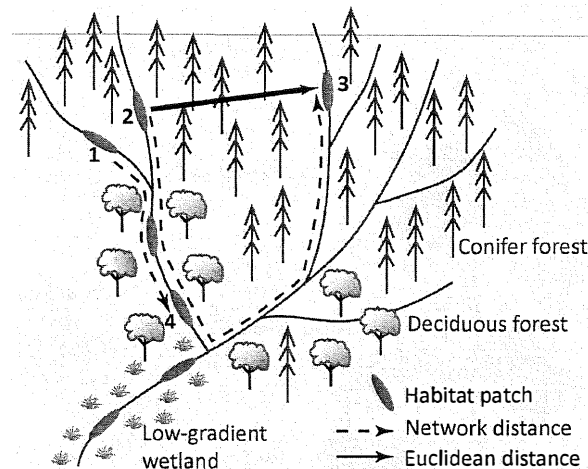
Figure 1. Contrasting interpretation of distance measures in a stream system: the shortest Euclidean distance is not the shortest network distance.
