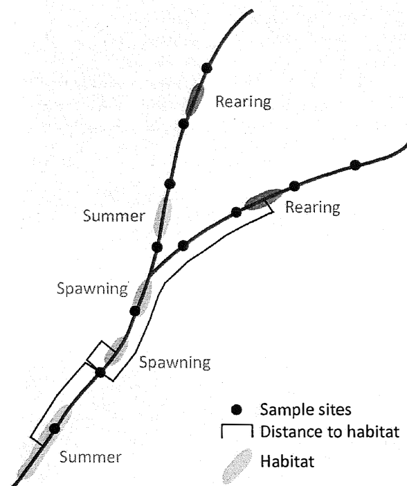
Figure 4. Network distances calculated from juvenile coho salmon snorkel sites to the closest available seasonal habitat.
