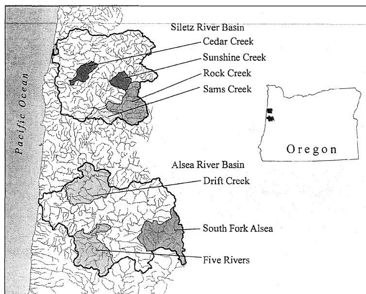
Figure 2. Highlighted sub-basins in the Alsea and Siletz River basins included in an analysis of multiple spatial scales over time that incorporated a stream network framework.
