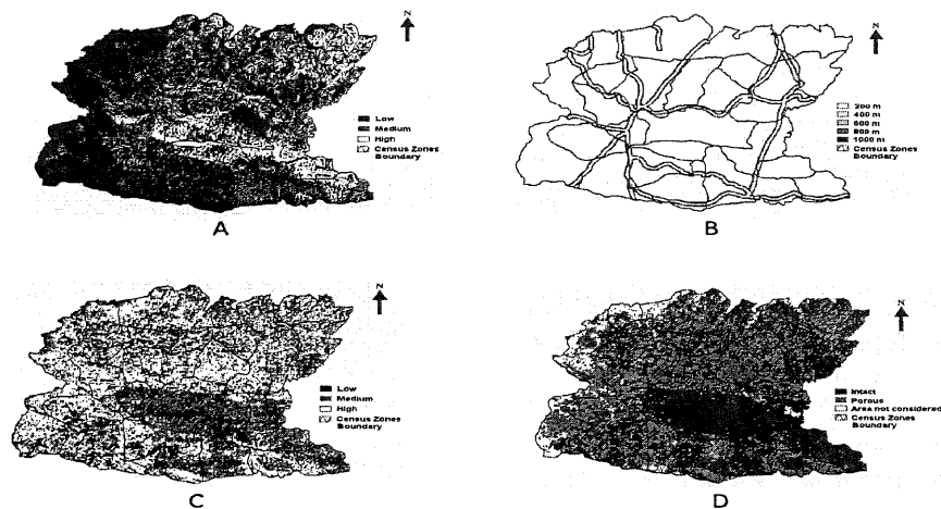
Figure 4. Topography, roads, and vegetation conditions in the entire Garo Hills: (a) terrain complexity, (b) roads and buffers, (c) vegetation patchiness, (d) vegetation porosity. Polygon outlines denote elephant census zones (Marak 1998; see Figure 5d).
