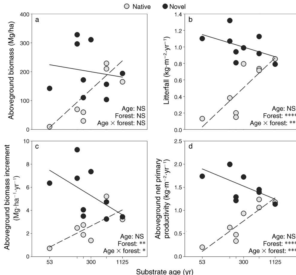
FIG. 3. Aboveground ecosystem properties and processes, including (a) aboveground biomass (AGB), (b) litterfall (leaves + stems <1 cm diameter), (c) AGB increment, (d) aboveground net primary productivity calculated as the sum of litterfall and AGB increment, in nine novel (solid line) forests dominated by introduced species compared to eight native forests (dashed line). Sites are found on a primary successional matrix of lava flows in lower Puna, Hawai'i Island. Significance levels reflect results of analysis of covariance, with substrate age (i.e., age) as the covariate (log-transformed to provide normality) and forest type as a fixed factor.
