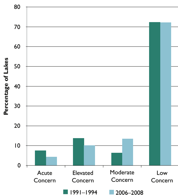
Figure 2-14. Northeastern TIME Lakes by ANC Category, 1991-1994, vs. 2006-2008. Acute Concern—less than 0 \mu\text{eq/L} , Elevated Concern—0 \mu\text{eq/L} to less than 50 \mu\text{eq/L} , Moderate Concern—50 \mu\text{eq/L} to less than 100 \mu\text{eq/L} , Low Concern—greater or equal to 100 \mu\text{eq/L} (prepared by U.S. EPA).
