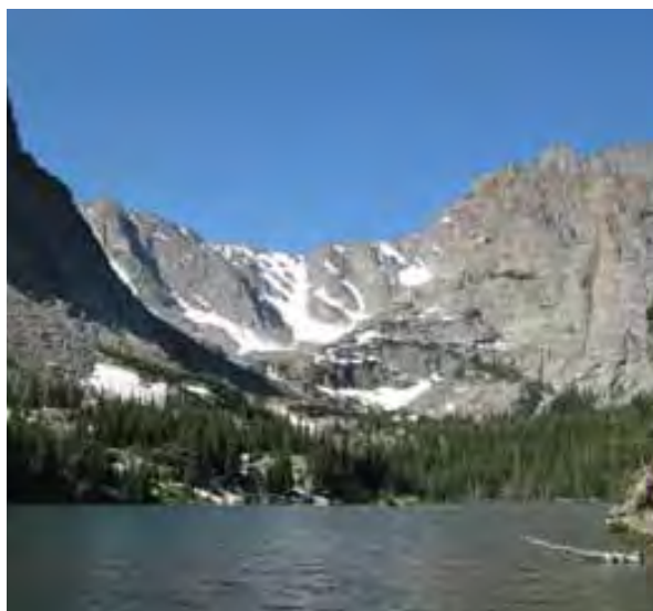
Loch Vale in Rocky Mountain National Park receives among the highest loads of atmospheric nitrogen deposition in the Front Range of the Colorado Rockies (photo courtesy USGS).
