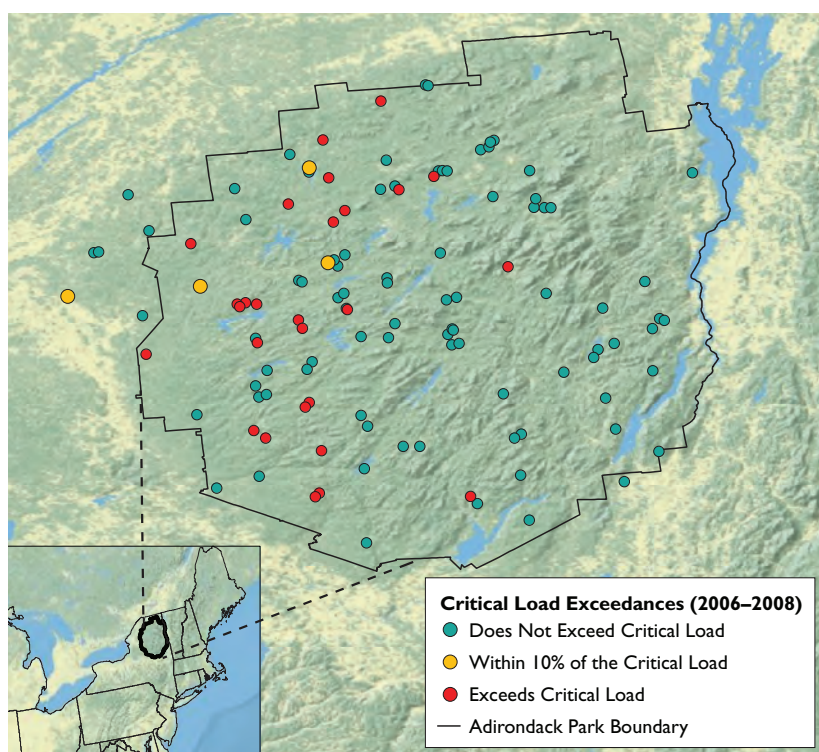
Figure 2-16. Critical load exceedances in Adirondack Mountain TIME lakes, 2006 to 2008 (No. lakes = 117) (prepared by U.S. EPA).
