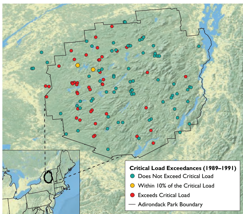
Figure 2-15. Critical load exceedances in Adirondack Mountain TIME lakes, 1989 to 1991 (No. lakes = 117) (prepared by U.S. EPA).
