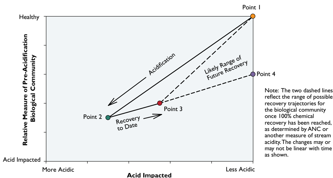
Figure 3-1. Conceptual figure showing hypothetical acidification and recovery patterns in a waterbody that has been acidified by atmospheric deposition (prepared by USGS).
