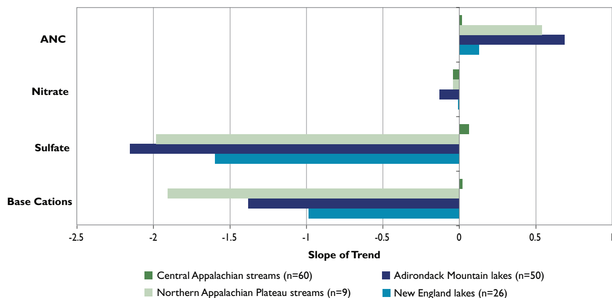
Figure 2-13. Trends in acidification of LTM lakes and streams, 1990–2008 (prepared by U.S. EPA).
