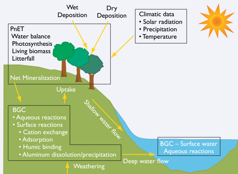
Conceptual diagram of the biogeochemical processes and chemical stores of the PnET-BGC model (figure courtesy of Charles Driscoll, Syracuse University).
