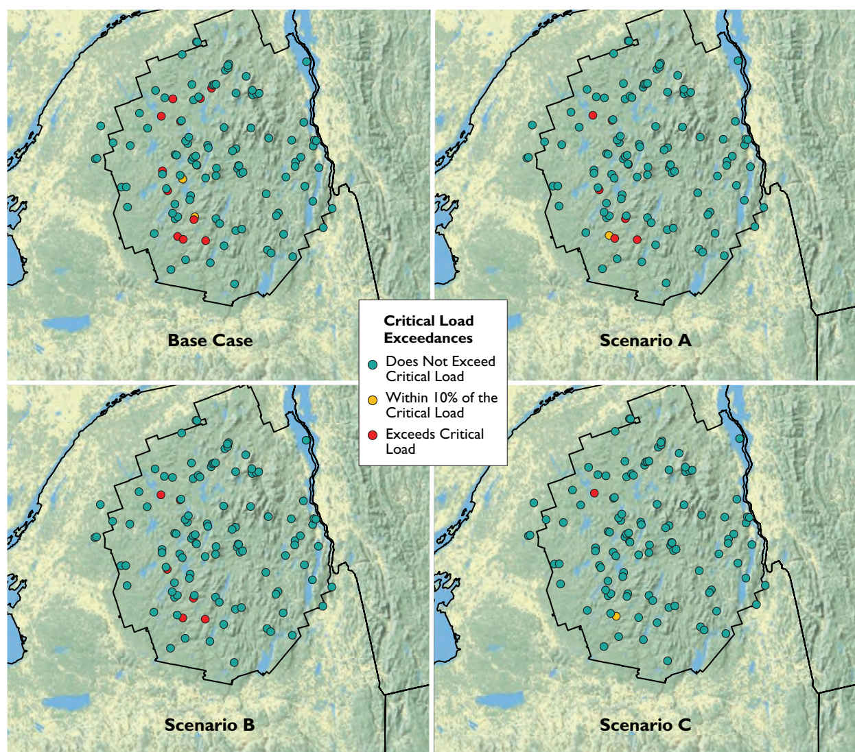
Figure 4-11. Critical load exceedances in the Adirondack Mountains (prepared by U.S. EPA).
