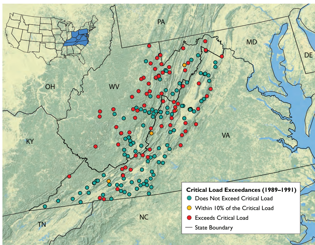
Figure 2-17. Critical load exceedances in central Appalachian streams, 1989 to 1991 (No. streams = 184) (prepared by U.S. EPA).
