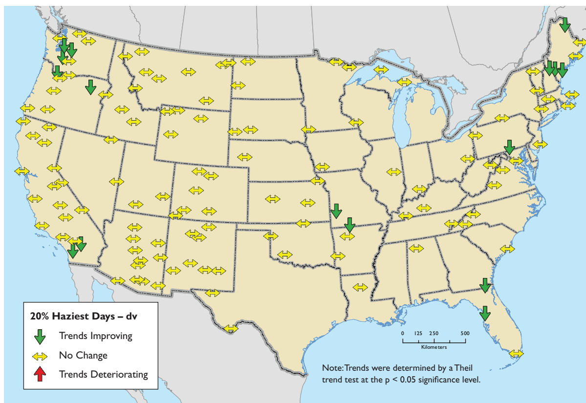
Figure 2-20. 1999 to 2008 trends for the change in visibility on the haziest days (worst 20% of visibility) as measured at 140 IMPROVE monitoring stations (prepared by NPS).
