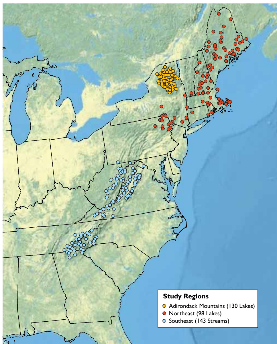
Figure 4-8. Regions and waterbodies modeled using MAGIC (prepared by U.S. EPA).
