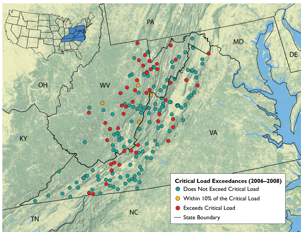
Figure 2-18. Critical load exceedances in central Appalachian streams, 2006 to 2008 (No. streams = 184) (prepared by U.S. EPA).
