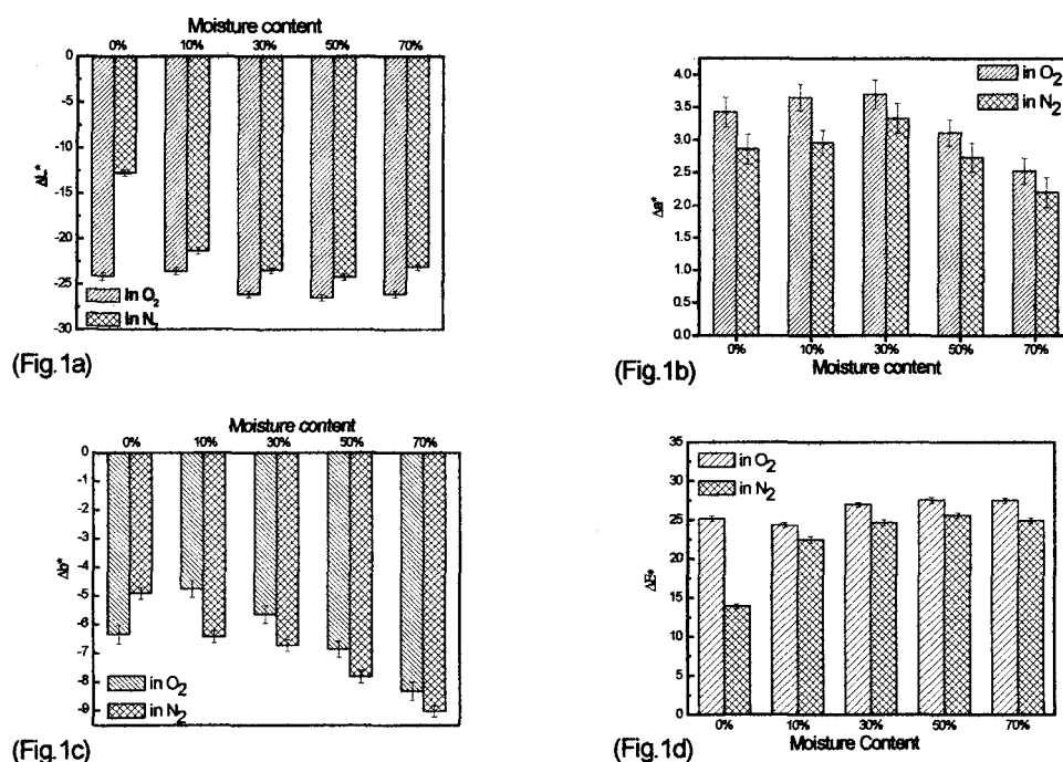
Fig. 1. Changes in color parameters for wood flour heat treated with different initial MCs in either oxygen or nitrogen atmosphere: (a) \Delta L^* , (b) \Delta a^* , (c) \Delta b^* , (d) \Delta E^*
