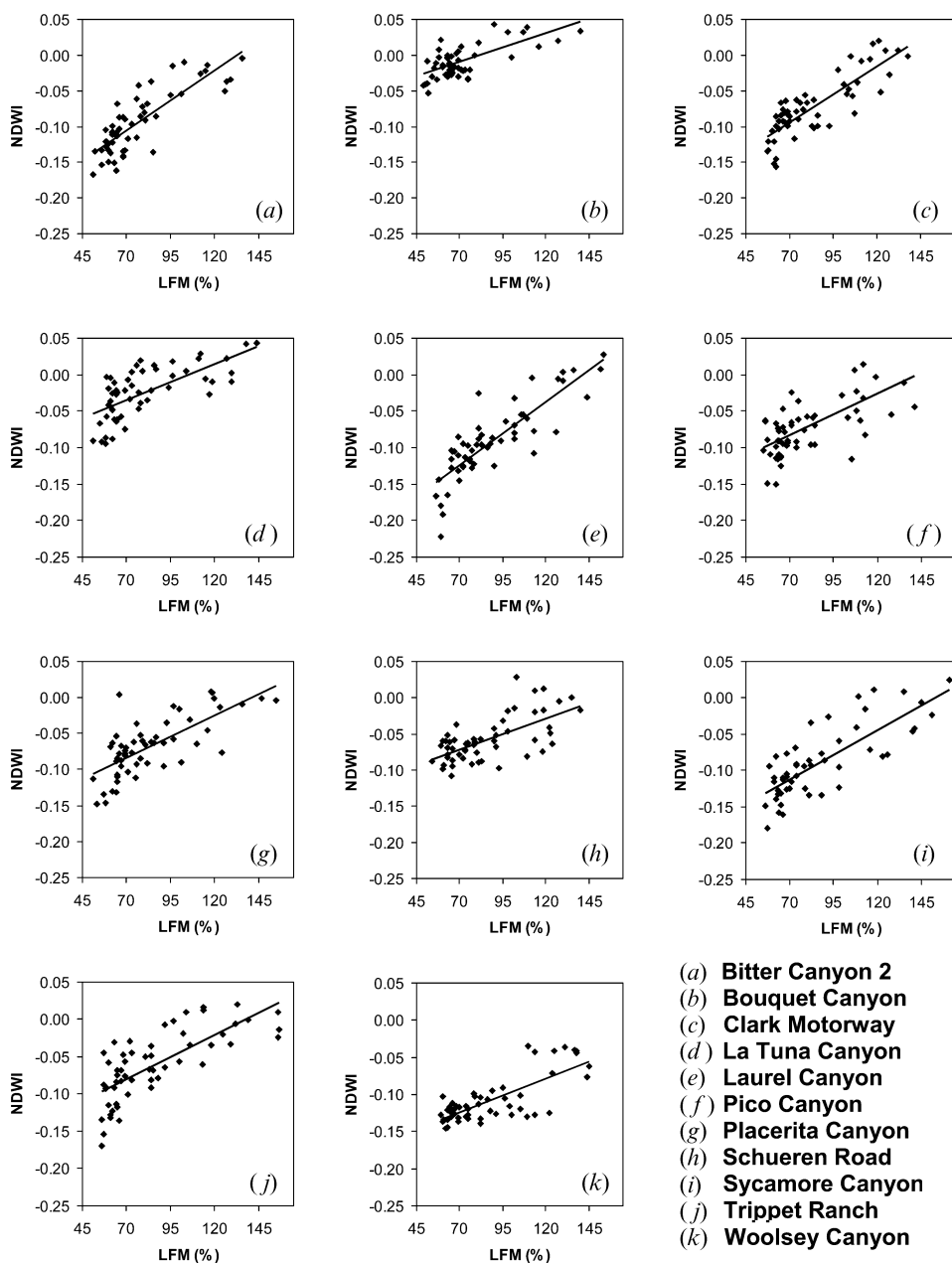
Figure 2. Plots of percentage live fuel moisture (LFM) versus NDWI for chamise ( Adenostoma fasciculatum ) at 11 sites sampled by LACFD. Each sampling date during the 2000–2002 period is represented by a point, while the lines indicate the best fit line.
