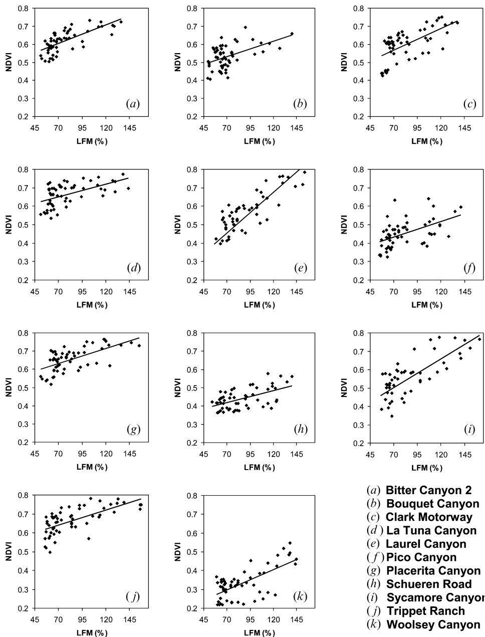
Figure 1. Plots of percentage live fuel moisture (LFM) versus NDVI for chamise ( Adenostoma fasciculatum ) at 11 sites sampled by LACFD. Each sampling date during the 2000–2002 period is represented by a point, while the lines indicate the best fit line.
