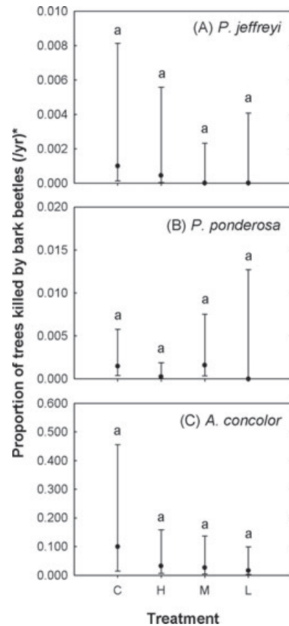
Figure 3 Proportion of (A) Pinus jeffreyi , (B) Pinus ponderosa and (C) Abies concolor trees killed by bark beetles (per year, all bark beetle species) over a 10-year period after thinning [low (18.4 m 2 /ha), medium (27.6 m 2 /ha), high (41.3 m 2 /ha), untreated control] in Pinus jeffreyi stands, Tahoe National Forest, California, U.S.A., 1999–2009. Points represent the mean with the 95% confidence interval. Bars followed by the same letter are not significantly different ( P > 0.05 ). *A theoretical upper confidence bound for the binomial distribution was calculated for treatments with zero mortality counts: Upper bound = \frac{1}{nyears} \left[ \frac{1-0.05}{nyears} \right] .
