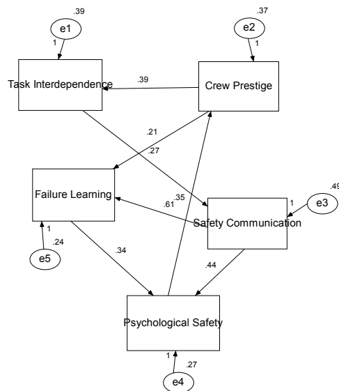
Figure 2. Structural Equation Model depicting relationships among variables measuring the crew interaction environment and communication activities. \chi^2(3) = 7.86, p = .05 ; CFI = .99 ; RMSEA = .09 ; SRMR = .03
