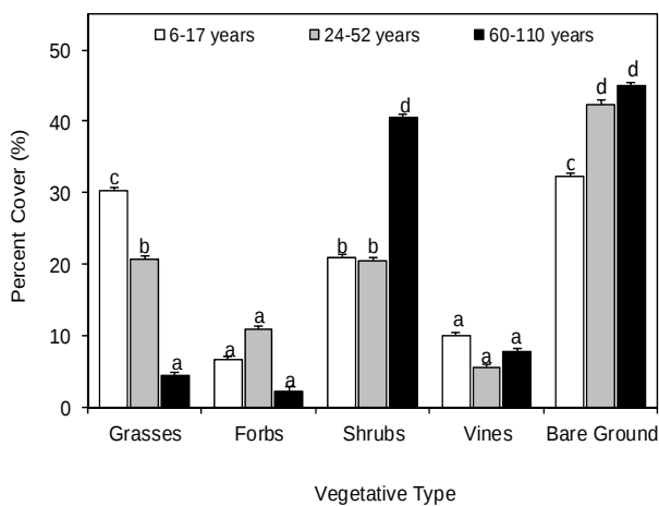
Figure 4. Composition of understory vegetation by patch age interval.
