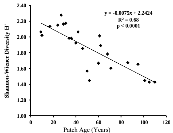
Figure 5. Shannon-Wiener Diversity index along a 110-year longleaf pine chronosequence as measured from 26 differently aged pine patches.
