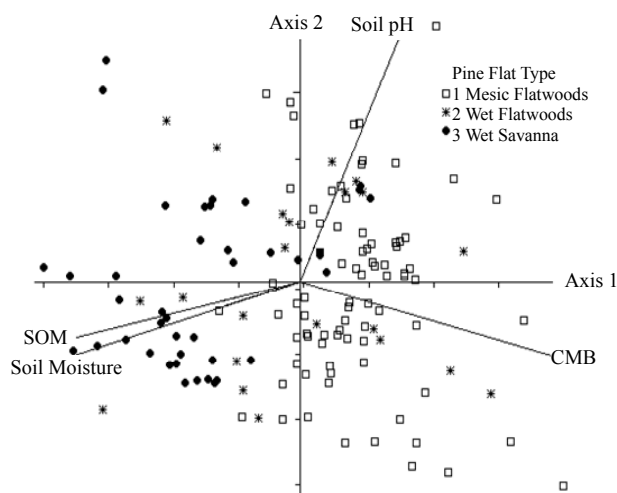
Figure 6. Pine flatwoods type determined by a four-dimensional ordination biplot derived from Canonical Correspondence Analysis (CCA) of 144 plots using understory plant species abundance and soil biogeochemical data (SOM, soil organic matter; CMB, microbial biomass carbon) from the three reference sites.
