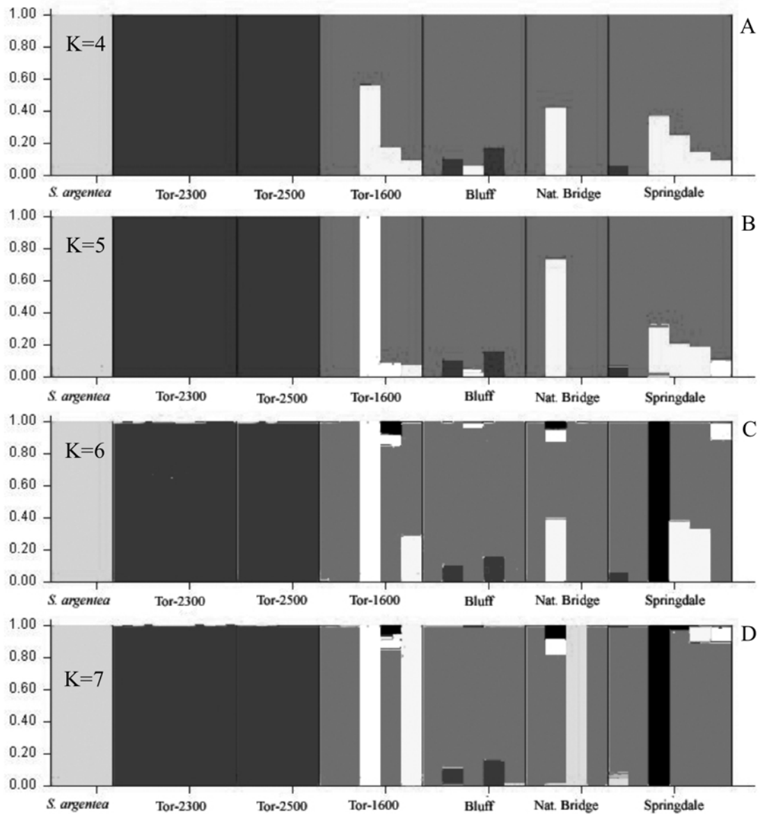
Fig. 4-7. Inferred population structure of Shepherdia rotundifolia AFLP genotypes from six populations in the field when; (A) testing a four population model (K = 4); (B) testing a five population model (K = 5); (C) testing a six population model (K = 6); and (D) testing a seven population model (K = 7); a thin vertical line represents each individual, black lines separate individuals of different populations
