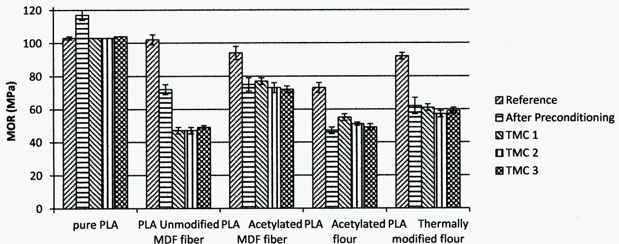
Fig. 3. Modulus of rupture for pure PLA and for the composite samples after water soaking and TMC exposure according to ENV 807
