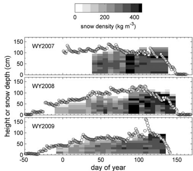
Figure 4. Snow depth at the SNOTEL site (open circles) and density profiles (from snow pits) during each winter (winter 1 on top, winter 3 on bottom). Density data are shown in 10 cm increments, and density is indicated by shading. Snow pit depth in the pits is indicated by the height of the density grid.
