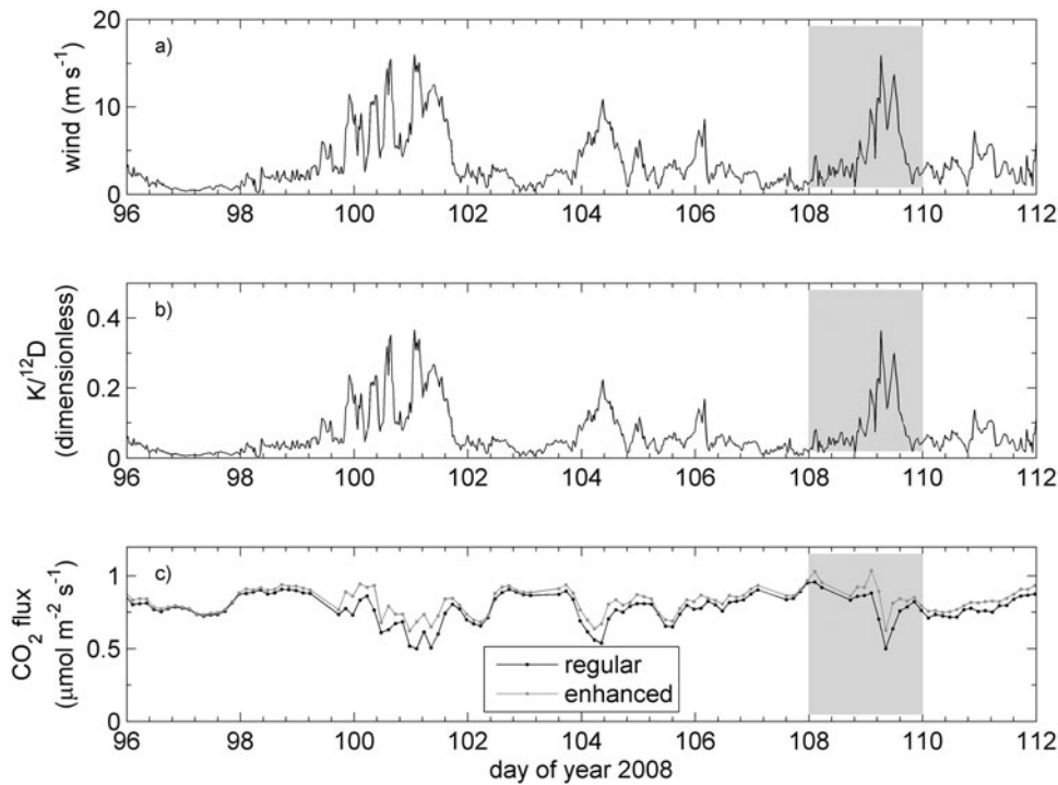
Figure 9. Sixteen-day time series of (a) above-canopy wind speed, (b) enhancement factor ( K/^{12}D ), calculated from the wind velocity regression for all winters (method A, shown in Figure 6), and (c) total \text{CO}_2 flux calculated with and without the enhancement to diffusion. The enhanced fluxes ( ^{12}F_{enh} + ^{12}F_s + ^{13}F_{enh} + ^{13}F_s ) are shown in gray, and the regular fluxes ( ^{12}F + ^{12}F_s + ^{13}F + ^{13}F_s ) are shown in black. The time period detailed in Figure 3 is highlighted in the gray box.
