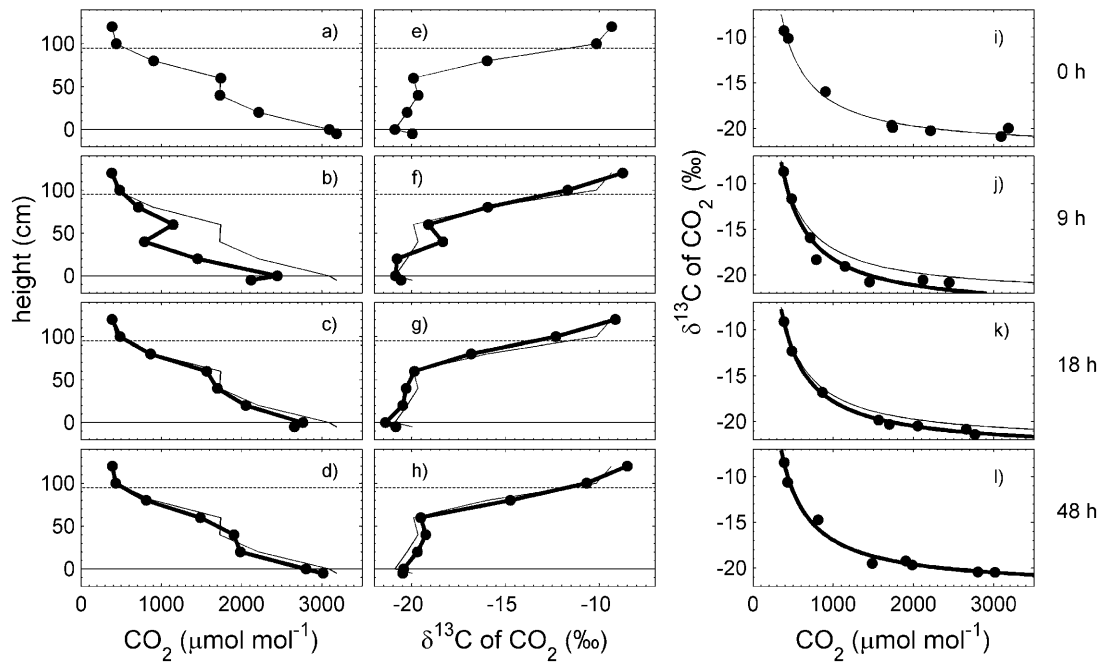
Figure 3. An example of the influence of wind on profiles of (a–d) \text{CO}_2 and (e–h) \delta^{13}\text{C} of \text{CO}_2 within the snowpack and soil. Data are shown from prior to the start of the wind event on 19 April 2007 (Figures 3a, 3e, and 3i) and from 9, 18, and 48 hours later (Figures 3b–3h and 3j–3l). (The wind time series is shown in Figure 9a.) (i–l) The relation between \delta^{13}\text{C} and \text{CO}_2 at each time period and mixing relationships for each. Thin solid lines in Figures 3a, 3e, and 3i are repeated in the panels below for comparison; in Figure 3l the thin line is obscured by the thick line. Horizontal lines in Figures 3a–3h indicate the snow–air interface (dashed) and the soil–snow interface (solid).
