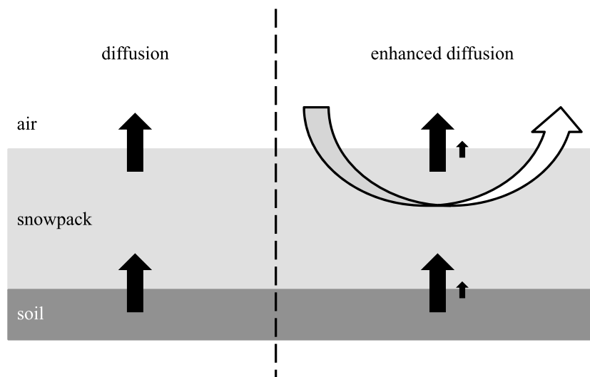
Figure 1. Conceptual diagram of the enhancement of diffusion caused by wind-induced snowpack ventilation, illustrating (left) a non-windy case in which the diffusive soil respiration flux (designated by the arrow) enters and leaves the snowpack and (right) how ventilation of the snowpack by pressure pumping can lead to an enhancement of flux rate (small arrow) beyond that due to molecular diffusion alone (large arrow) for a given gradient in \text{CO}_2 . Note that the actual \text{CO}_2 production rate by respiration is not changed, but the transport is enhanced.
