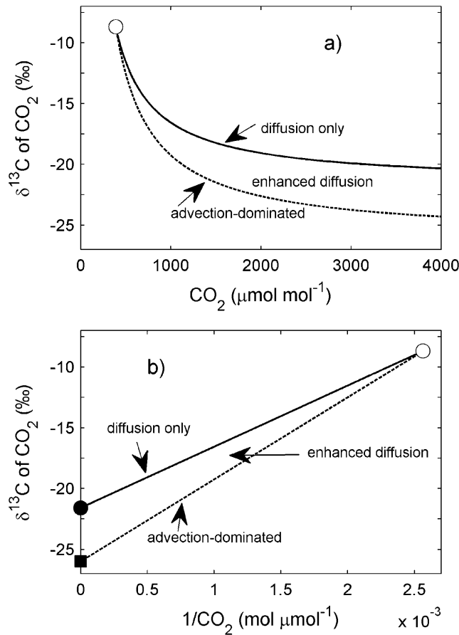
Figure 2. Theoretical mixing relationships of \text{CO}_2 and \delta^{13}\text{C} of \text{CO}_2 when air mixes with soil-respired \text{CO}_2 , with (a) the measured quantities and (b) the Keeling-plot version shown. The lines represent the same mixing relationships in both panels. Under nondiffusive conditions, the air outside the snowpack (open circle) will mix along the dashed line with \text{CO}_2 produced by respiration (with \delta^{13}\text{C} indicated by the square). Under fully diffusive conditions, a kinetic fractionation affects the \text{CO}_2 within the snowpack, and mixing follows the solid line. The y -intercepts of the lines in Figure 2b are separated by 4.4‰, and a Keeling plot constructed with samples collected under fully diffusive conditions will have an intercept (solid circle) that is more enriched than the actual respiratory source (square). The zone in between represents the variable isotopic effect associated with enhanced diffusion. For this figure an assumed \delta^{13}\text{C} of respiration of -26\text{‰} was used [Bowling et al. , 2009].
