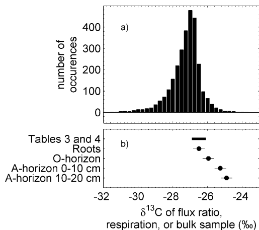
Figure 7. (a) Frequency distribution for the ratio of total fluxes [(^{13}\text{F} + ^{13}\text{F}_s)/(^{12}\text{F} + ^{12}\text{F}_s)] converted to delta notation (equation (8)). Data for all winters are shown. (b) The range of values for the assumed isotope ratio of soil respiration ( \delta_s ) that was associated with regression intercepts of 1.0044 (in Tables 3 and 4) and the measured \delta^{13}\text{C} of bulk roots and soils [Schaeffer et al., 2008] are shown for comparison.
