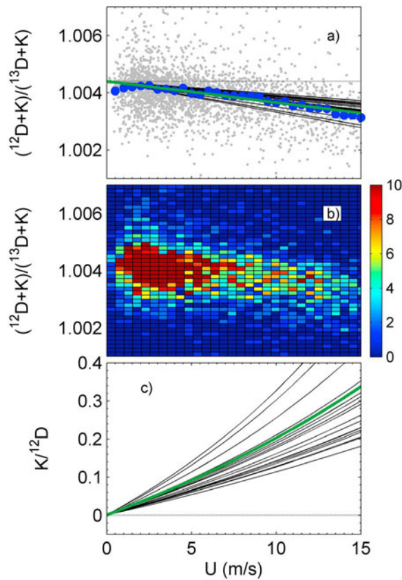
Figure 6. Dependence of the apparent isotopic fractionation associated with diffusion on above-canopy wind speed. When there is no wind ( U = 0 ), the enhanced diffusivity ( \text{K} ) is zero, and the diffusivity ratio (equation (10)) converges to equation (3), with an intercept of 1.0044 (shown in Figure 6a as a horizontal dashed line). (a) Relationship between the diffusivity ratio and wind speed for all winters, including 3 h data (gray circles). Means ( \pm 1 SE error bars, smaller than symbols in some cases) are shown for wind bins of width 0.5 \text{ m s}^{-1} (blue circles), and a linear regression (green solid line) through the 3 h data is shown (italicized in Table 3). Also shown (in black) are all the statistically significant regression lines from Tables 3 and 4. (b) Two-dimensional frequency distribution of the data in Figure 6a (color axis indicates number of occurrences). (c) The enhancement factor ( \text{K}/^{12}\text{D} ) as a function of wind speed, which is derived via equation (10) from the regressions shown in Figure 6a. Quantities on the ordinate axes are dimensionless in all cases.
