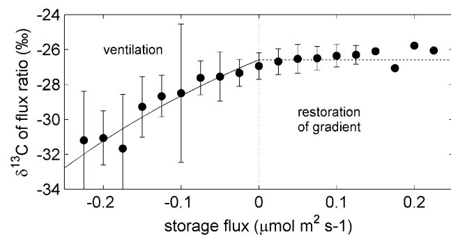
Figure 8. The influence of the storage flux on the \delta^{13}\text{C} of the flux ratio (as in Figure 7a). Means ( \pm 1 SD error bars) are shown for storage flux bins of width 0.025 \mu\text{mol m}^{-2} \text{s}^{-1} (missing error bars indicate fewer than 3 samples). The right half of the figure (positive storage flux) represents periods when the \text{CO}_2 stored in the snowpack increased as respiratory \text{CO}_2 was added during calm conditions. The left half represents a decrease in the \text{CO}_2 stored as the snowpack was ventilated by wind. The lines were calculated using equation (14) as described in the text.
