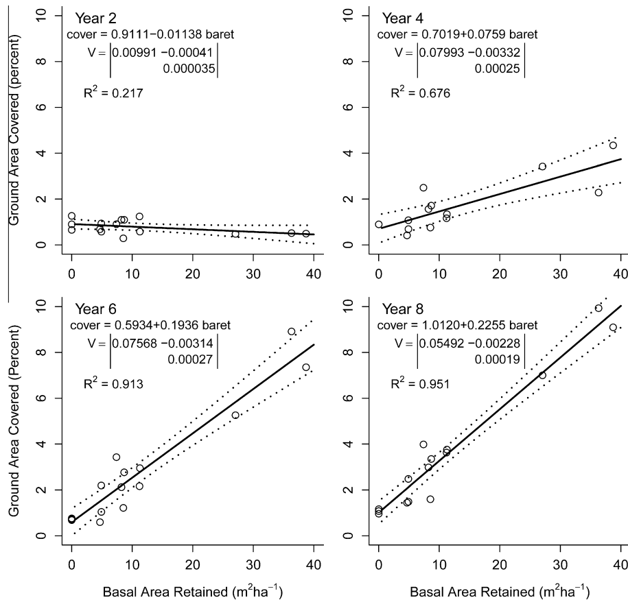
Fig. 6. Percent ground area covered by fuels >7.6 cm, observed (circles) and modeled (solid line), with 95% confidence intervals (dotted lines) and parameter estimate covariance matrix (V), over snag basal area retained ( \text{baret m}^2 \text{ha}^{-1} ).
