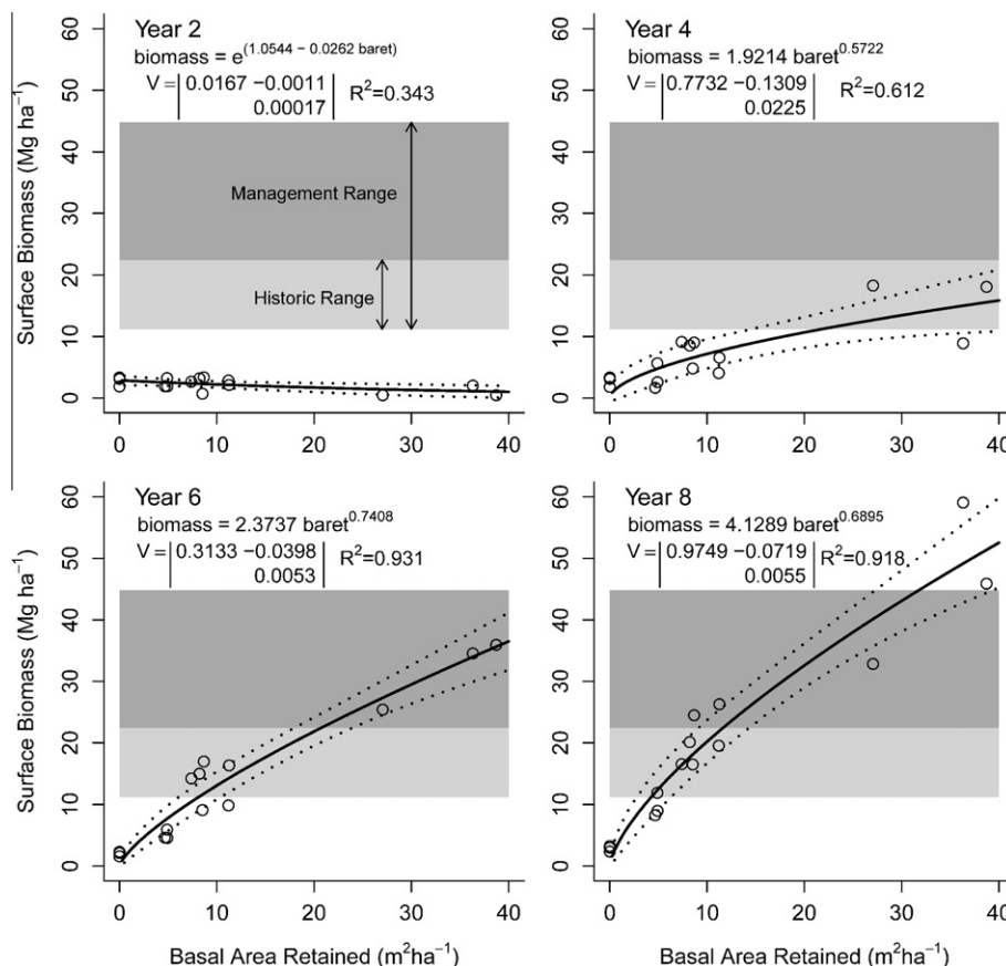
Fig. 4. Surface fuel accumulation, observed (circles) and modeled (solid line) with 95% confidence intervals (dotted lines) and parameter estimate covariance matrix ( V ), for material >7.6 \text{ cm} in diameter, over basal area retained ( \text{baret m}^2 \text{ ha}^{-1} ); historic and management ranges (Brown et al., 2003) are shaded.
