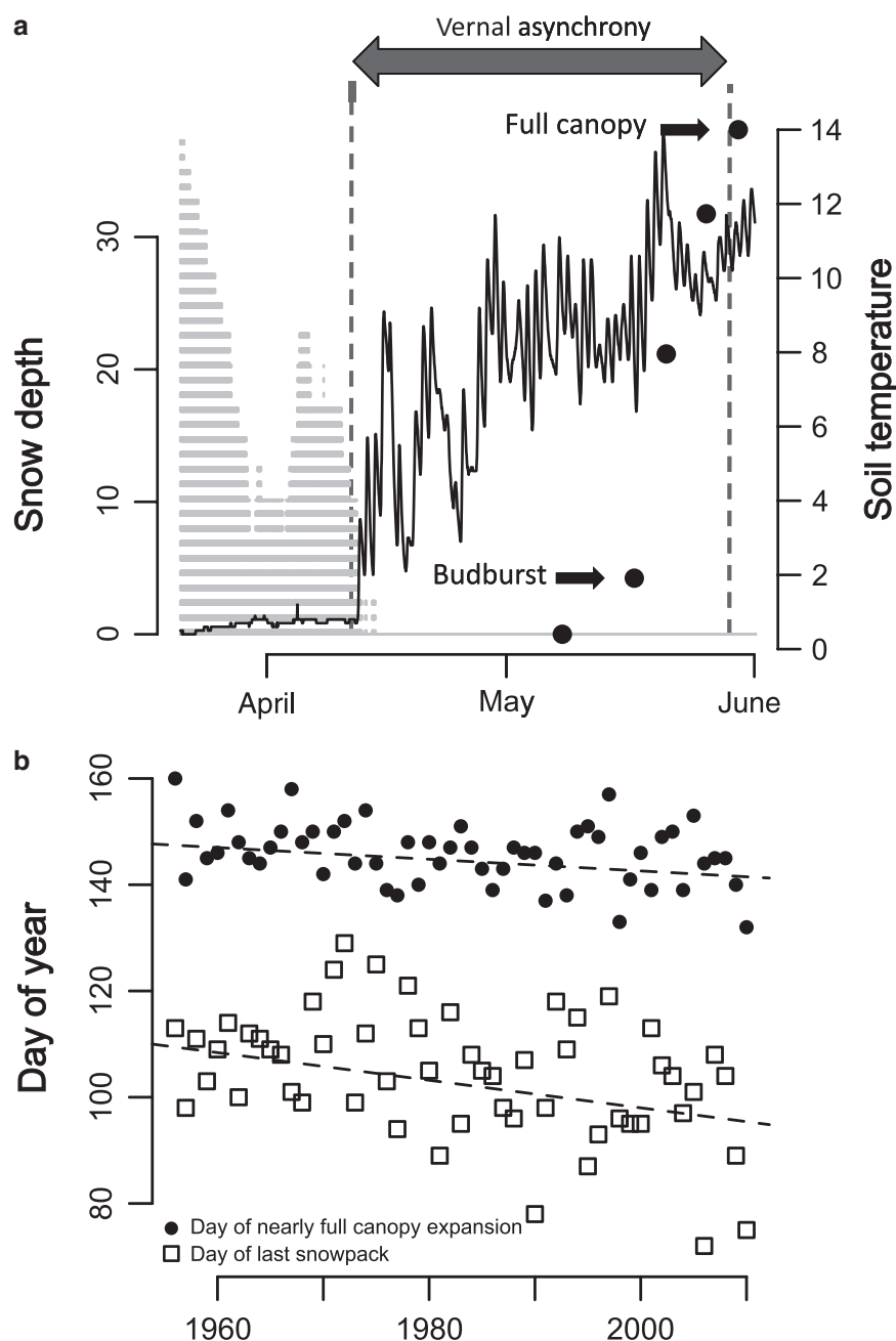
Figure 2. An example of (a) the relationship between the loss of snowpack (snow depth, in centimeters), soil temperature (in degrees Celsius), and spring leaf phenology and (b) changes in the modeled day of nearly complete canopy expansion and last snowpack at a middle elevation site in the Hubbard Brook Experimental Forest. In panel (a), data from 2003 show how the disappearance of snowpack (shown by the horizontal shading) coincides with an abrupt increase in soil temperature at 4 centimeters (cm; the solid line). The closed circles represent spring leaf phenology, and the arrow denotes the period of vernal asynchrony (see the text) that has increased over time. Spring canopy expansion (the closed circles) is becoming earlier, at a rate of 1.1 days per decade ( p = .02 ), whereas the day of last snowpack (the open squares) is becoming earlier at a rate of 2.6 days per decade ( p = .004 ); therefore, the length of the period between snowmelt and full canopy development has increased by over 8 days in 55 years.
