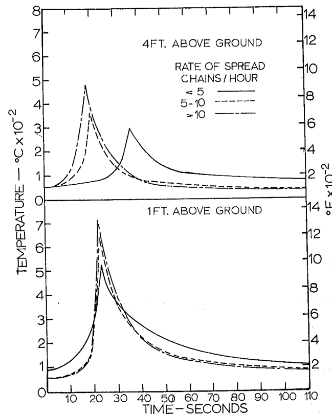
FIG. 4. Smoothed time-temperature records obtained by thermocouple from prescribed fires in palmetto-gallberry fuel in south Georgia. Note that fires with higher rates of spread indicate a higher temperature, probably due to higher gas velocities by the thermocouples.
