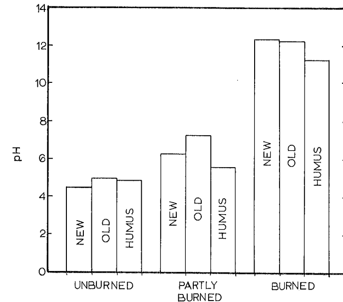
FIG. 2. Values of pH recorded from unburned, partly burned, and completely burned litter from a 28-year-old loblolly pine stand in Montgomery County, Virginia. The pH for all components of the fuel rose from less than 5 to greater than 11 when completely burned.
