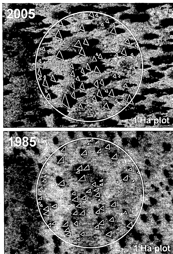
Figure 2. Photo interpretation of juniper cover. After rectifying the paired images from 1985 (or 1986) and 2005, an isosceles triangle was manually traced over each juniper tree contained in the 1-ha circular plot, with the base spanning crown diameter perpendicular to sun angle and a height spanning crown radius in the direction of the sun. The area of each triangle was calculated automatically using ArcMap software (ESRI, Redlands, CA) and converted to projected elliptical crown area as triangle area \times \pi .
