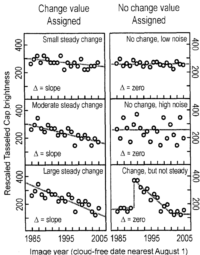
Figure 3. Examples of how LandTrendr was used to identify and quantify steady negative trends of 18 yr or more in brightness for each Landsat pixel. As shown on the right, pixels were assigned a default change value of zero when reflectance values over this period were flat, too noisy, or showed signs of punctuated change. Because we were attempting to detect juniper cover increases, any pixels exhibiting positive trajectories in brightness were also assigned a default change value of zero (not shown). As shown on the left, when brightness decreases over at least 18 yr are fit with a single negative linear segment, change was assigned according to the magnitude of the decrease.
