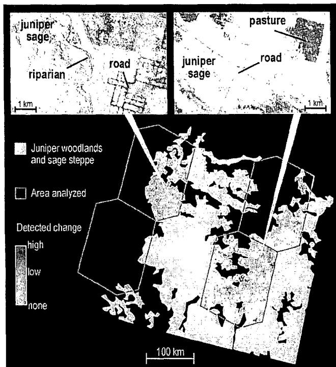
Figure 6. The detection of steady vegetation change for juniper woodlands of Oregon. Blue areas are those that exhibited steady, uninterrupted decreases in tasseled-cap brightness for at least 18 continuous years sometime between 1984 and 2007. White areas within analyzed polygons are those that exhibited no steady, uninterrupted decreases in tasseled-cap brightness. Overall, 27% of the area analyzed exhibited some steady decline in brightness over the measurement period. These locations were often identifiable as landform, vegetation, and anthropogenic features.
