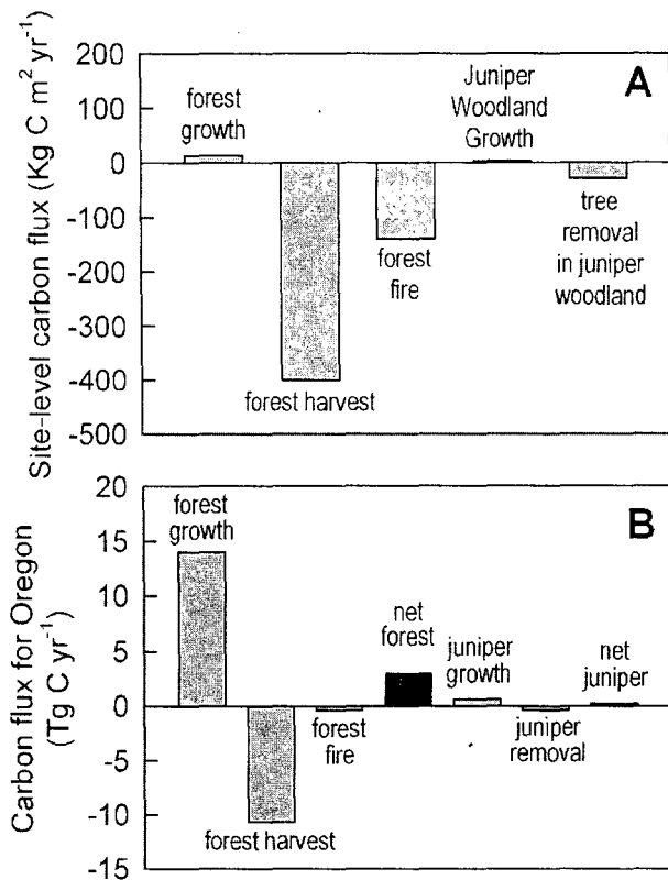
Figure 8. Changes in aboveground carbon stocks attributed to juniper encroachment compared with simulated ecosystem fluxes, A , per unit area and B , across all of Oregon. Net carbon accumulation in juniper woodlands, like forest biomass, is the small balance between large losses over small areas and small gains over larger areas. Note also that the gross and net carbon fluxes attributed to juniper encroachment in Oregon is very small compared to that of forests. Juniper fluxes are from this study, other fluxes are adapted from Turner et al. (2007).
