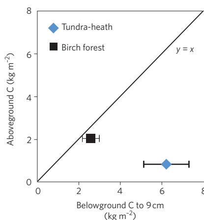
Figure 1 | Hartley et al. 3 show that as tundra systems give way to birch forest, more ecosystem carbon is harboured in aboveground pools, at a net loss of total ecosystem carbon. Belowground carbon pools dwarf aboveground pools, especially if one considers carbon deeper in the soil. Error bars were propagated from standard errors provided in the Supplementary Information 3 (belowground: bulk density and depth; aboveground: leaves, stems and roots). Y axis error bars are too small to plot.
