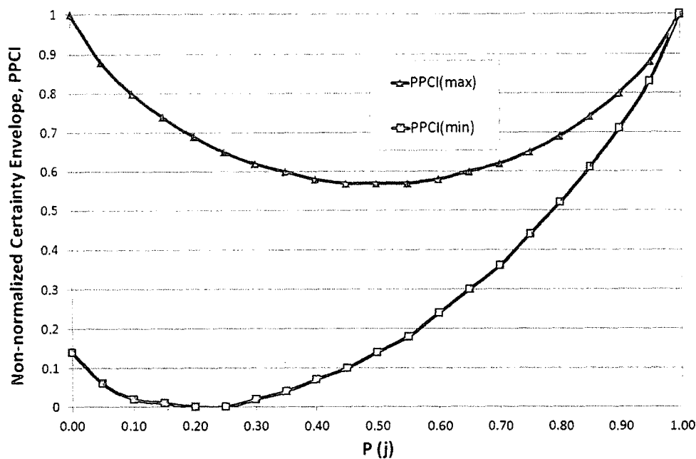
Fig. 1. Non-normalized certainty envelope of a probability distribution with N=5 states across the full range of probability values of a single state, P(N_5) .
