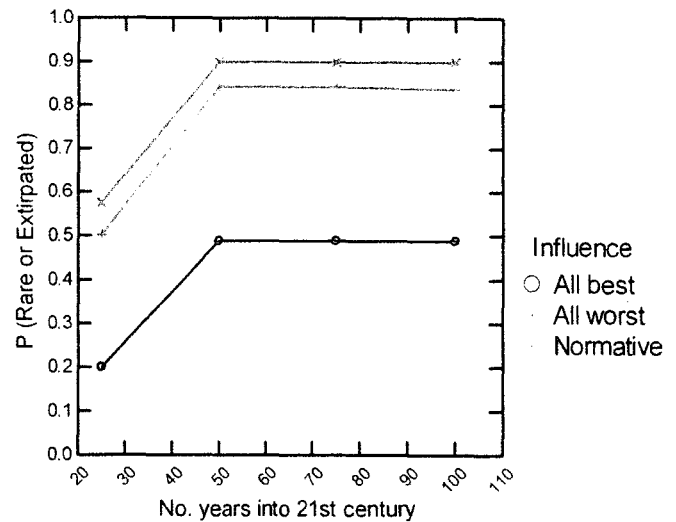
Fig. 3. Example of influence analysis of polar bear populations, under the IPCC B1 greenhouse gas scenario, plotting the probability of polar bear populations in the Seasonal Ice Ecoregion becoming rare or extirpated outcomes at 4 future time periods (Amstrup et al., 2010). “Normative” results refer to setting all stressors to their expected values for each time period, whereas the “all best” and “all worst” results refer to setting them to their best and worst case influences.
