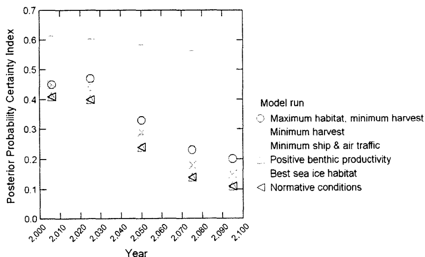
Fig. 6. Example of the posterior probability certainty index (PPCI; 1 = full certainty, 0 = full uncertainty) as a function of future time period, from posterior probability distributions of Pacific walrus populations, under normative and selected best-case influence analysis scenarios, under the IPCC A1B greenhouse gas scenario.
