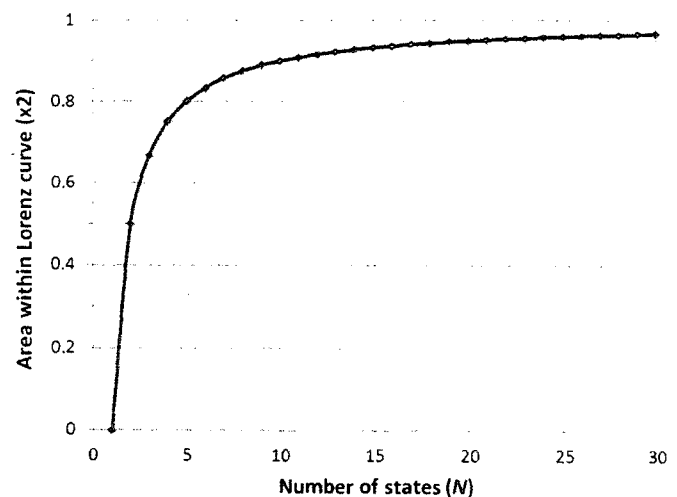
Fig. 2. Maximum value of the area within the Lorenz curve (=Gini coefficient, here doubled) increases asymptotically to 1.0 as a function of the number of states, as applied to posterior probabilities from Bayesian network models.
