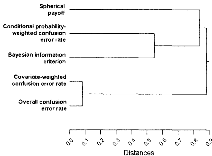
Fig. 8. Similarity (single linkage using Euclidean distance) of 5 metrics of Bayesian network model prediction performance based on the case example of modeling marten ( Martes spp. ) age as a function of genetic, somatic, and environmental variables (see text).
