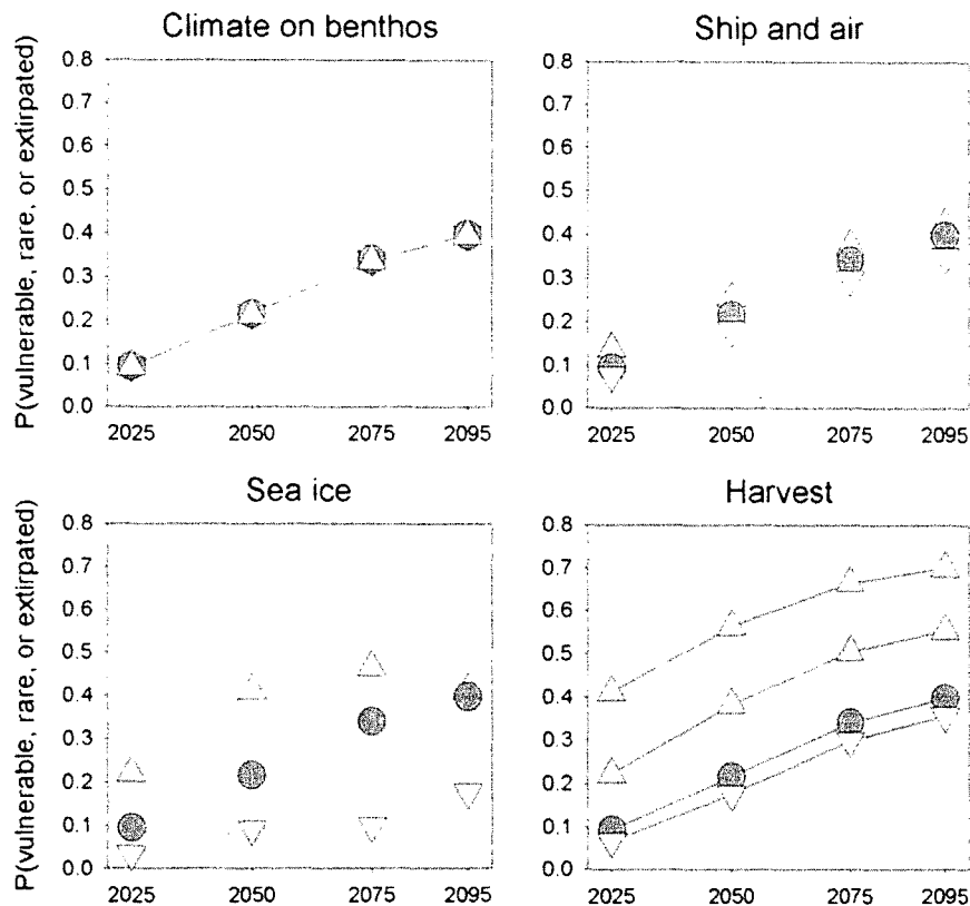
Fig. 5. Results of BN model runs of future Pacific walrus populations under normative (gray circles) and best-case and worst-case influence analyses (open triangles pointing downward and upward, respectively), plotting probability of future populations becoming vulnerable, rare, or extirpated as a function of future time period, under the IPCC A1B greenhouse gas scenario.
