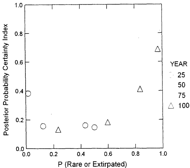
Fig. 4. Example of the posterior probability certainty index (PPCI; 1 = full certainty, 0 = full uncertainty) as a function of the posterior probability of polar bear populations becoming rare or extirpated in each of four global ecoregions, by future time period, under the IPCC B1 greenhouse gas scenario.
