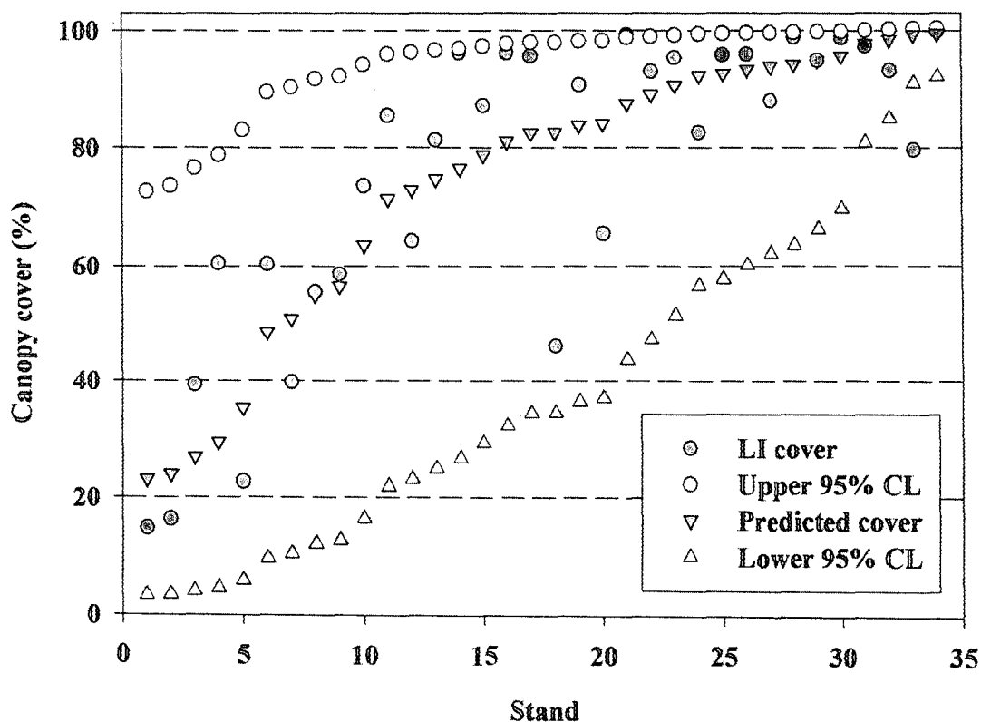
Figure 5. Predicted canopy cover for the wet hardwood forest group using model 8 (stocking) compared with measured line-intercept (LI) cover from the test data set. Individual stands are in ascending order by predicted cover. The 95% upper and lower confidence limits (CL) used the SE of the estimates.
