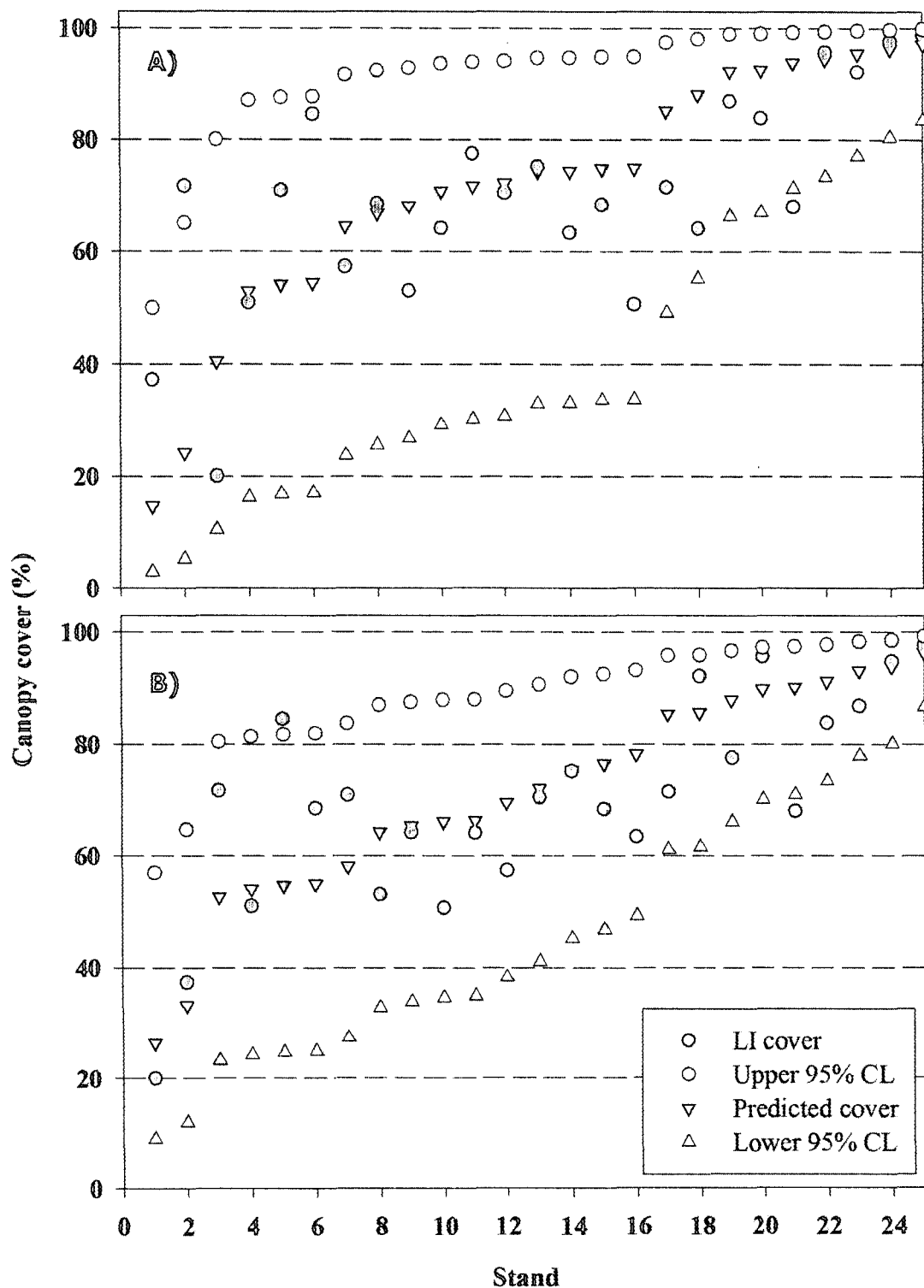
Figure 6. Predicted canopy cover for the dry hardwood conifer forest group using (A) model 44 (age, basal area, mai, and stand height) and (B) model 29 (stocking, mai, and stand height) compared with measured line-intercept (LI) cover from the test data set. Individual stands are in ascending order by predicted cover. The 95% upper and lower confidence limits (CL) used the SE of the estimates.
