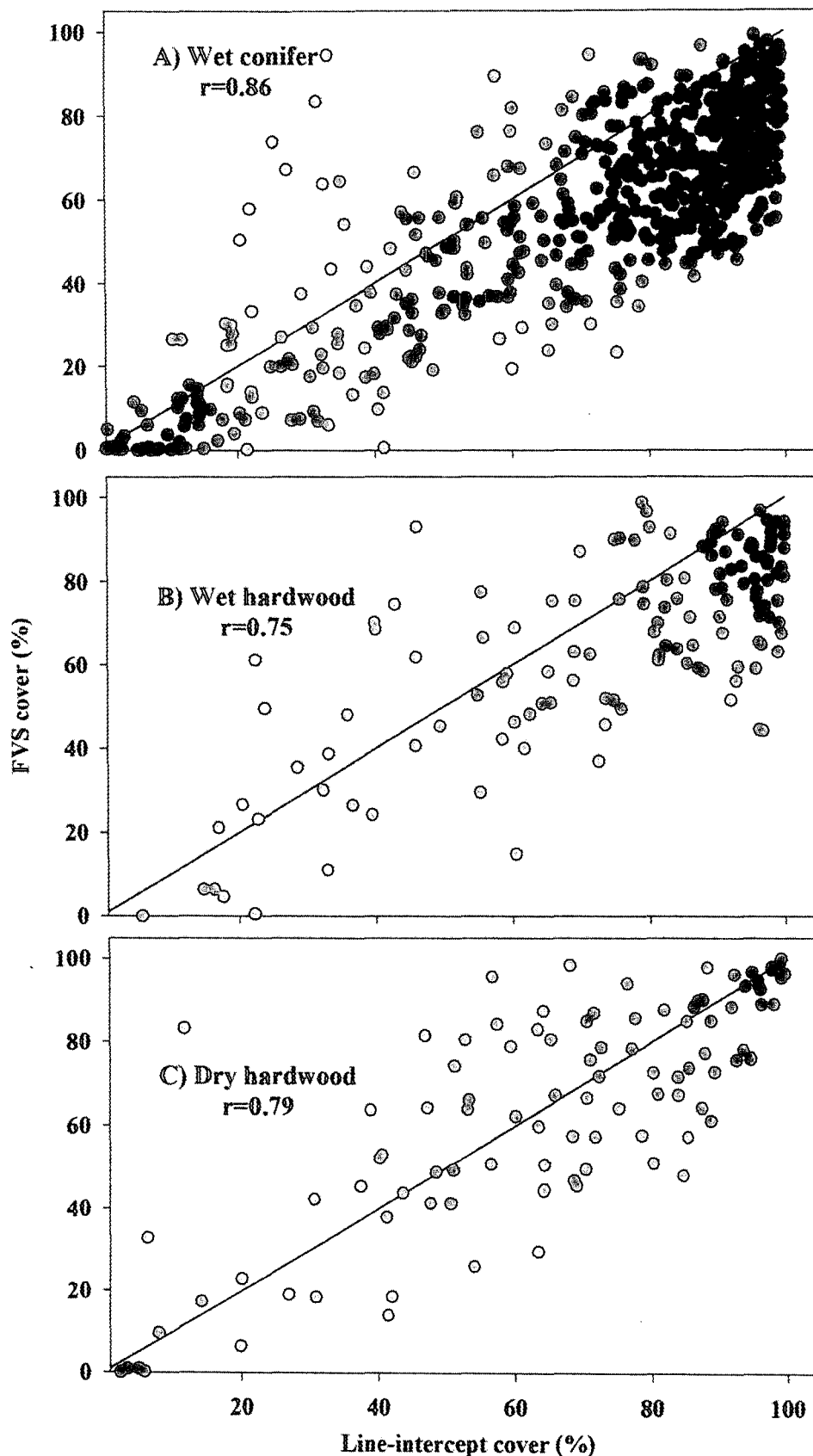
Figure 3. Comparison of cover predicted by FVS equations and ground-measured line-intercept cover for three general forest groups in western Oregon. The diagonal line represents a 1:1 relationship between the two cover estimates. The r value is the Pearson correlation coefficient.
