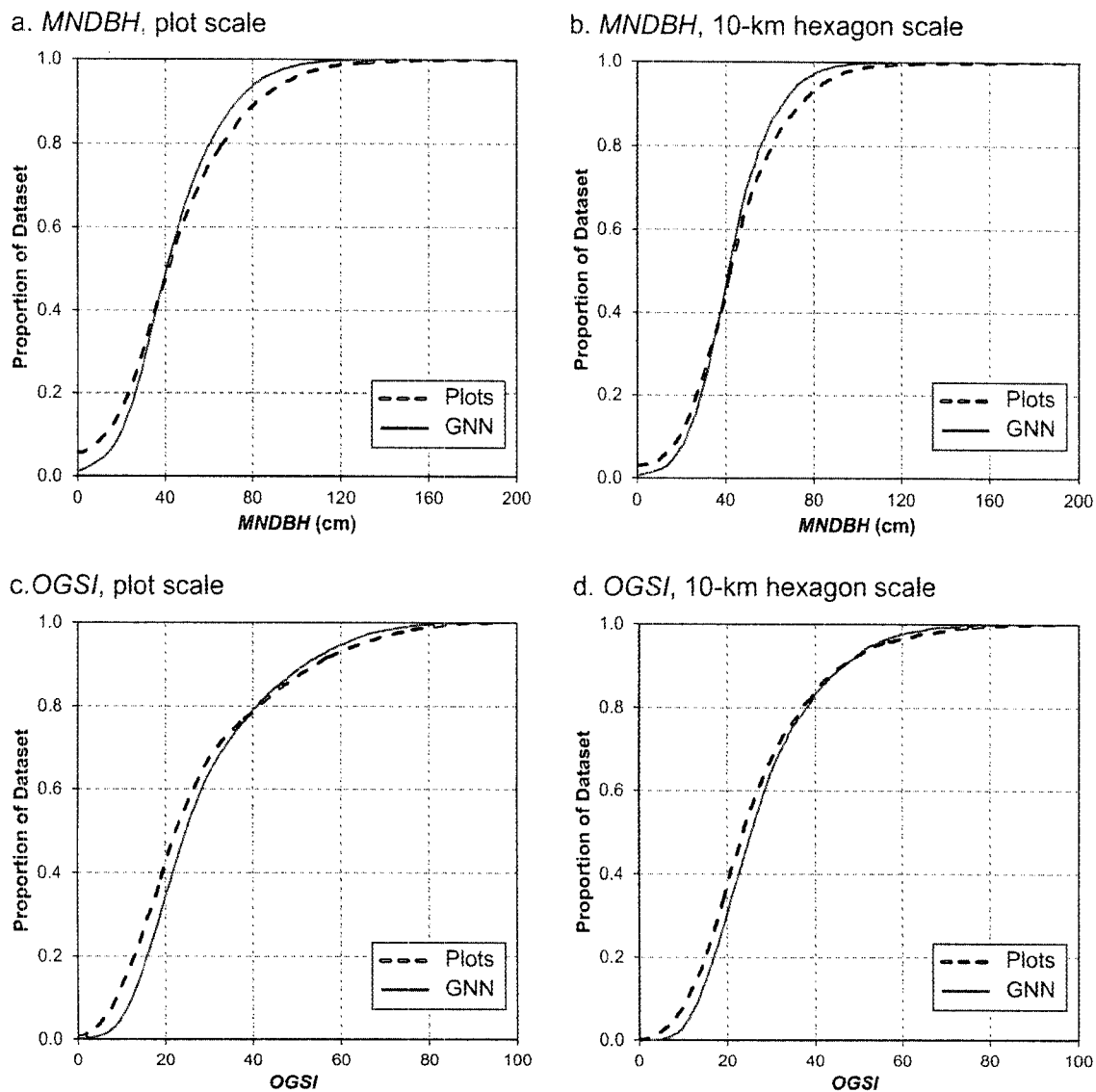
Fig. 8. Empirical cumulative distribution functions (ECDFs) for the FIA plot- and GNN-based estimates at the plot and 10-km-hexagon scales, for MNDBH and OGSi . The n = 5,505 FIA plots were measured from 2001 to 2008 and the GNN distributions are for Time 2 (2006/2007).
