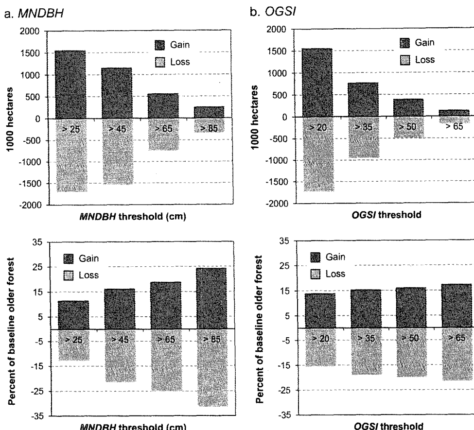
Fig. 3. Change in distribution of older forest from Time 1 to Time 2, shown as gross gain and gross loss, by threshold value for MNDBH where CANCOV > 40 (a) and OGSi (b). Change is expressed as area (top graphs) and as a percentage of older forest at Time 1 (bottom graphs).
