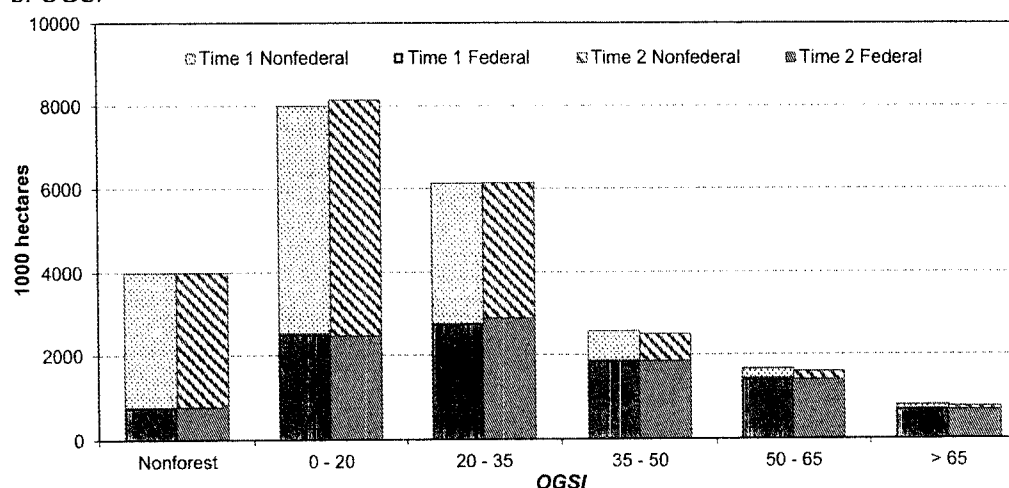
Fig. 2. Distribution of forest area by ownership and forest attribute ( MNDBH (a) and OGSI (b)), at Time 1 and Time 2. CANCOV is total tree canopy cover (%).
