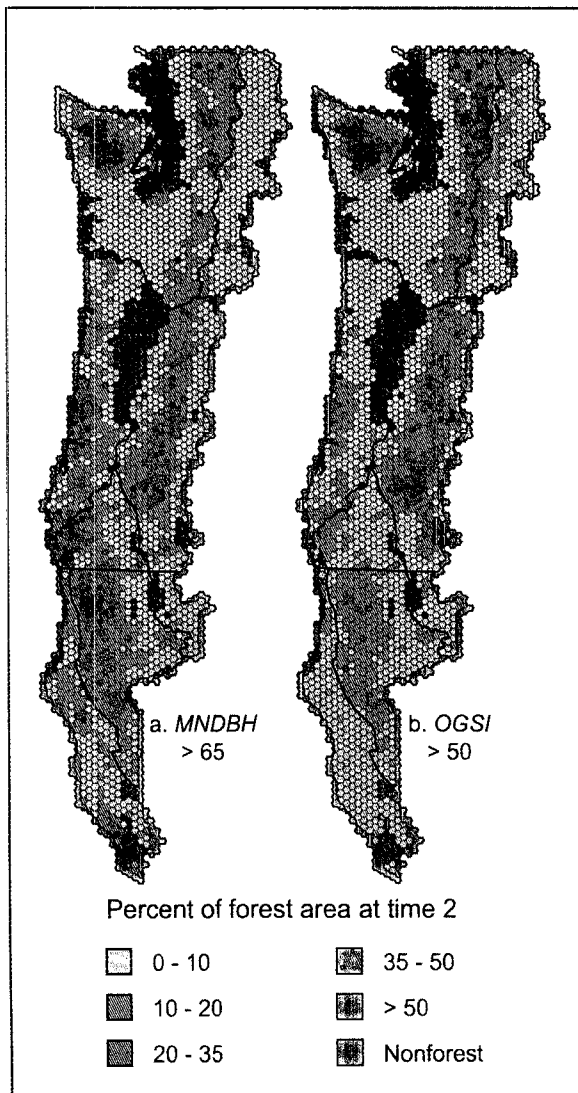
Fig. 4. Geographic distribution of older forest at Time 2 based on example threshold values for forest attributes: MNDBH \geq 65 (a) and OGSI \geq 50 (b). Values are percentage of GNN pixels meeting the threshold definition within 10-km hexagons.
