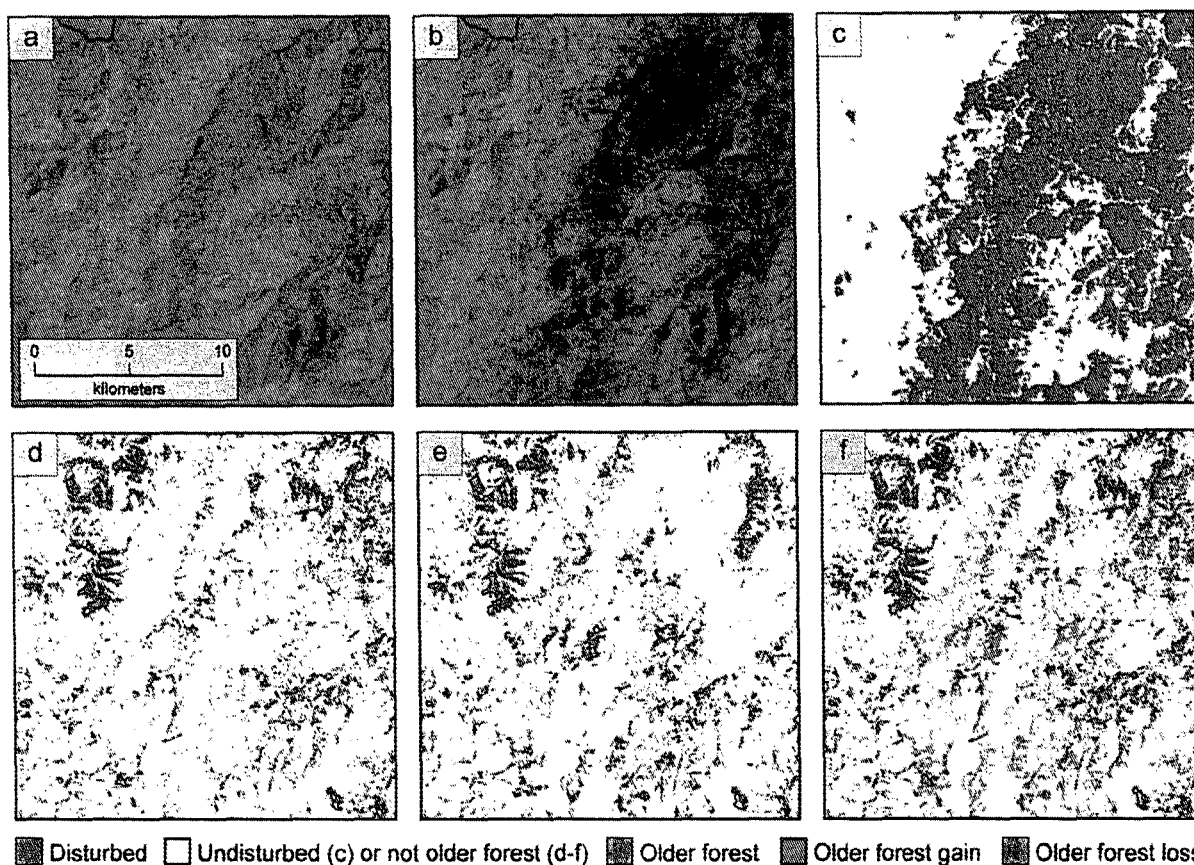
Fig. 5. A forest landscape in southwest Oregon encompassing a portion of the 2002 Biscuit Fire, showing tasseled cap axes 1–3 from Landsat imagery as a red-green-blue composite image for Time 1 (a) and Time 2 (b), areas mapped as disturbed from LandTrendr algorithms (c), older forest ( OGSI > 50 ) from GNN at Time 1 (d) and Time 2 (e), and change in older forest from spatial differencing the Time 1 and Time 2 maps (f). Note the fine-scale variability in older forest as mapped by GNN, and the comingled areas of older forest gain and loss within the disturbed area.
