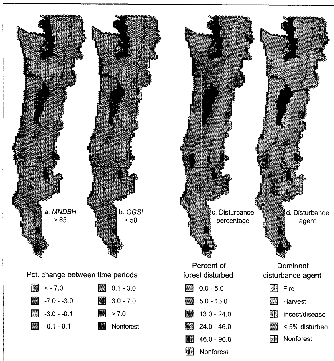
Fig. 6. Geographic distribution of forest change between Time 1 and Time 2: (a) Change in older forest ( MNDBH \geq 65 ) from Time 1 to Time 2 (from GNN). (b) Change in older forest ( OGSI \geq 50 ) (from GNN). (c) Percentage of forest disturbed (from LandTrendr; Kennedy et al., in press). (d) Dominant disturbance agent for hexagons with \geq 5\% disturbance (from LandTrendr).
