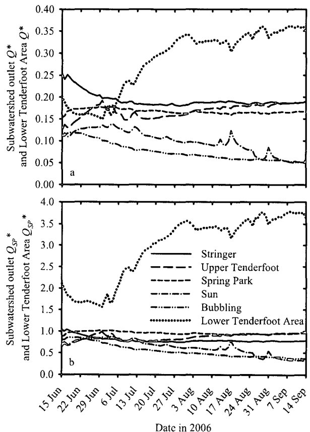
Figure 4. (a) Relative contributions to 2006 TCEF outlet base flow ( Q^* ) and (b) corresponding relative areal yields ( Q_{SP}^* ) from the subwatershed outlets and the Lower Tenderfoot contributing area.
