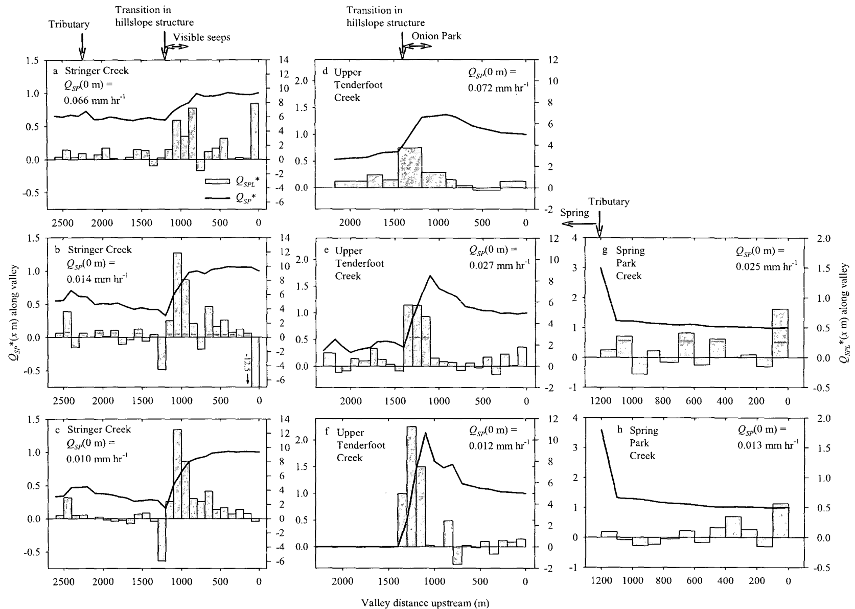
Figure 7. Longitudinal distributions of local areal yield relative to outlet areal yield ( Q_{SP}^*(x\text{ m}) , lines) and lateral areal yield relative to outlet areal yield ( Q_{SPL}^*(x\text{ m}) , bars) along the valleys of (a–c) Stringer Creek, (d–f) Upper Tenderfoot Creek, and (g and h) Spring Park Creek. Figures for each stream are stacked in order of decreasing flow at the outlet. Locations of notable hydrologic and structural features from Figure 2 are cross-referenced above the graphs.
