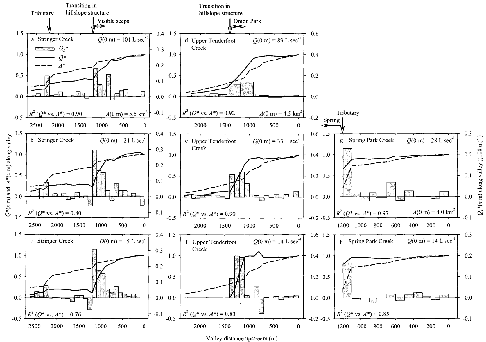
Figure 6. Longitudinal distributions of local discharge relative to outlet discharge ( Q^*(x\text{ m}) , solid lines), accumulated contributing area relative to outlet contributing area ( A^*(x\text{ m}) dashed lines), and lateral streamflow contributions relative to outlet discharge ( Q_L^*(x\text{ m}) , bars) along the valleys of (a–c) Stringer Creek, (d–f) Upper Tenderfoot Creek, and (g and h) Spring Park Creek. Figures for each stream are stacked in order of decreasing flow at the outlet. Locations of some notable hydrologic and structural features from Figure 2 are cross-referenced above the graphs.
