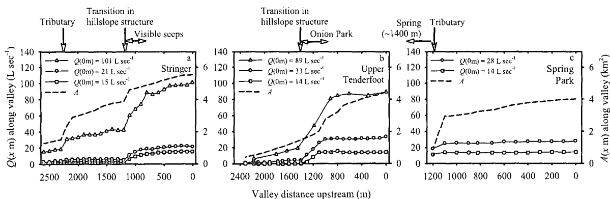
Figure 5. Longitudinal distributions of stream discharge ( Q(x\text{ m}) ) and topographic contributing area ( A(x\text{ m}) ) along the valleys of (a) Stringer Creek, (b) Upper Tenderfoot Creek, and (c) Spring Park Creek. Locations of some notable hydrologic and structural features from Figure 2 are cross-referenced above the graphs.
