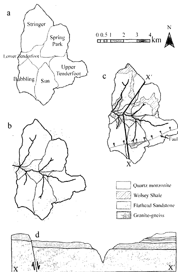
Figure 1. Site map and structural characteristics of the Tenderfoot Creek Experimental Forest watershed (TCEF, lat. 46^{\circ} 55' \text{ N} , long. 110^{\circ} 52' \text{ W} ) and its 5 gauged subwatersheds, including (a) names of subwatersheds, (b) topographic map with 20 m contours, (c) underlying bedrock geologic units [Reynolds and Brandt, 2007], and (d) an approximate bedrock profile along line X-X' (enlarged and the vertically exaggerated for clarity) (M. Reynolds, personal communication, 2009). The TCEF outlet gauge and 5 subwatershed gauges are located at the intersection of the stream with its corresponding watershed boundary. The Lower Tenderfoot contributing area is the region of TCEF that does not drain to 1 of the 5 subwatershed gauges.
