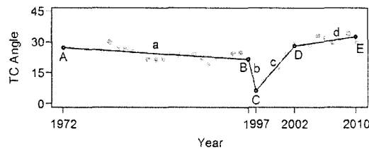
Fig. 4. Example of a normalized Landsat time series for a single pixel, showing yearly tasseled cap angle values (gray dots), the fitted time series (black lines), and the fitted segment start and end vertices (black dots). Downward trending segments represent disturbance (or maturation) and upward trending segments represent recovery. Flat segments (not shown) represent stable segments. A variety of disturbance and succession process (and related) parameters are derived from the fitted segment vertices. For example, the duration for insect disturbance segment a is determined by subtracting the year of vertex A from that of vertex B. The magnitude of change for fire disturbance segment b is calculated from the difference between the TCA values of B and C. The spectral value at vertex C represents the spectral value at the end vertex for the disturbance having the greatest observed magnitude. Time since the end of the greatest disturbance is calculated by subtracting the year of vertex C from that of vertex E for recovery segments c and d.
