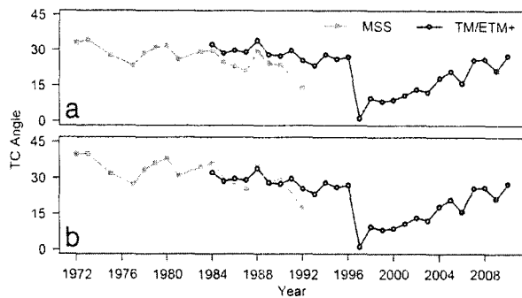
Fig. 2. Example trajectory of a single Landsat pixel showing TCA offset before (a) and after (b) pixel-level alignment of time series. The abrupt decrease of TCA in 1997 was caused by a stand replacing wildfire in August 1996. The disturbance is followed by a slow increase in TCA indicating forest recovery.
