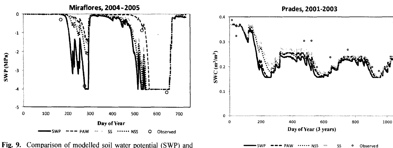
Fig. 10. Comparison of modelled and observed soil water content (SWC) from 2001 to 2003 for a holm oak stand at Prades using 4 methods that relate soil water to g_{sto} (see methods section for details).
