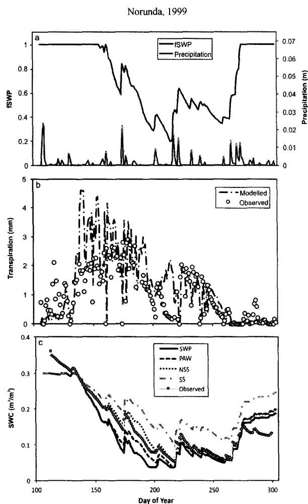
Fig. 3. (a) Modelled f_{\text{SWP}} and measured precipitation for a mixed Norway spruce and Scots pine stand at Norunda in 1999 using the PAW method; (b) Observed and modelled transpiration for the same year, stand and soil water calculation method; (c) Observed and modelled soil water content (SWC) using all four methods that relate soil water to g_{\text{sto}} (see methods section for details).
