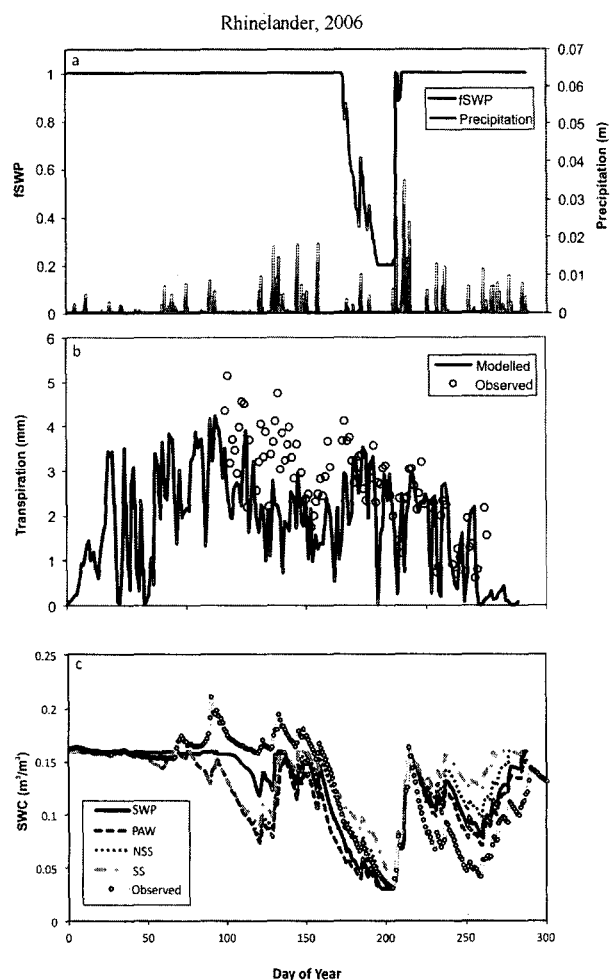
Fig. 4. (a) Modelled f_{\text{SWP}} and measured precipitation for a mixed aspen-birch stand at Rhineland in 2006 using the SWP model; (b) Observed and modelled transpiration for the same year, stand and soil water calculation method; (c) Observed and modelled soil water content (SWC) using all four methods that relate soil water to g_{\text{sto}} (see methods section for details).
