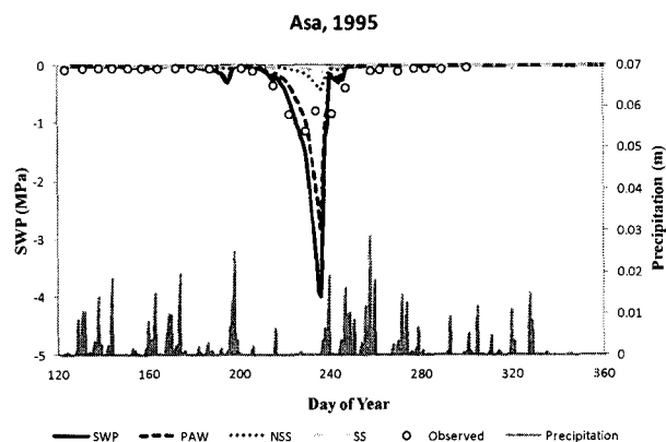
Fig. 6. Comparison of observed and modelled soil water potential (SWP) in 1995 for a Norway spruce stand at Asa using four methods that relate soil water to g_{sto} (see methods section for details).
