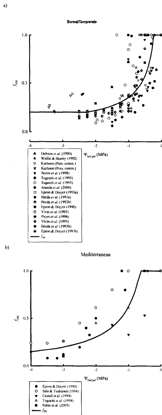
Fig. 2. f_{sw} relationships in comparison with observed data describing relative g_{sto} with pre-dawn leaf water potential ( \Psi_{leaf,pd} ) for (a) coniferous (Norway spruce and Scots pine) and deciduous (beech) trees in north and central Europe with \Psi_{max} = -0.6 MPa; \Psi_{min} = -1.5 MPa; PWP = -4.0 MPa and (b) Mediterranean trees (Holm oak) with \Psi_{max} = -0.9 MPa; \Psi_{min} = -3.6 MPa; PWP = -4.0 MPa.
