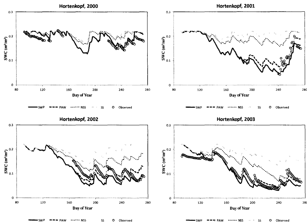
Fig. 8. Comparison of observed and modelled soil water content (SWC) in 2000, 2001, 2002 and 2003 for a mixed beech and temperate oak stand at Hortenkopf using four methods that relate soil water to g_{sto} (see methods section for details).
