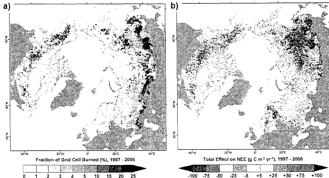
Figure 5. The spatial pattern of the (a) total fraction of grid cell area burned and (b) average annual effect ( \text{gC m}^{-2} \text{yr}^{-1} ) of all controlling factors on NEE across the boreal land regions over the 1997 to 2006 time period.
