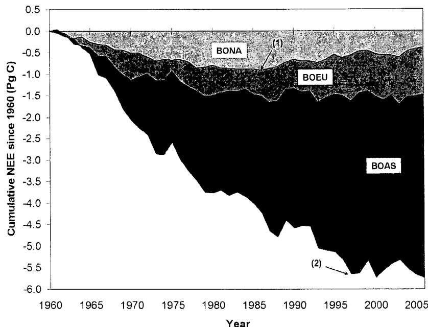
Figure 2. Estimated cumulative net uptake of atmospheric CO 2 (NEE) by boreal land regions since the latter half of the 20th century, according to the simulation experiment with all factors included (Sim7).
