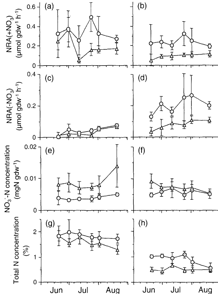
Fig. 5 Seasonal changes in NRA(+NO 3 ), NRA(-NO 3 ), NO 3 - -N concentration, and N concentration in leaves and roots of S. interior and P. balsamifera . Means ± SD (n=5) are shown for a leaf NRA(+NO 3 ), b root NRA(+NO 3 ), c leaf NRA(-NO 3 ), d
