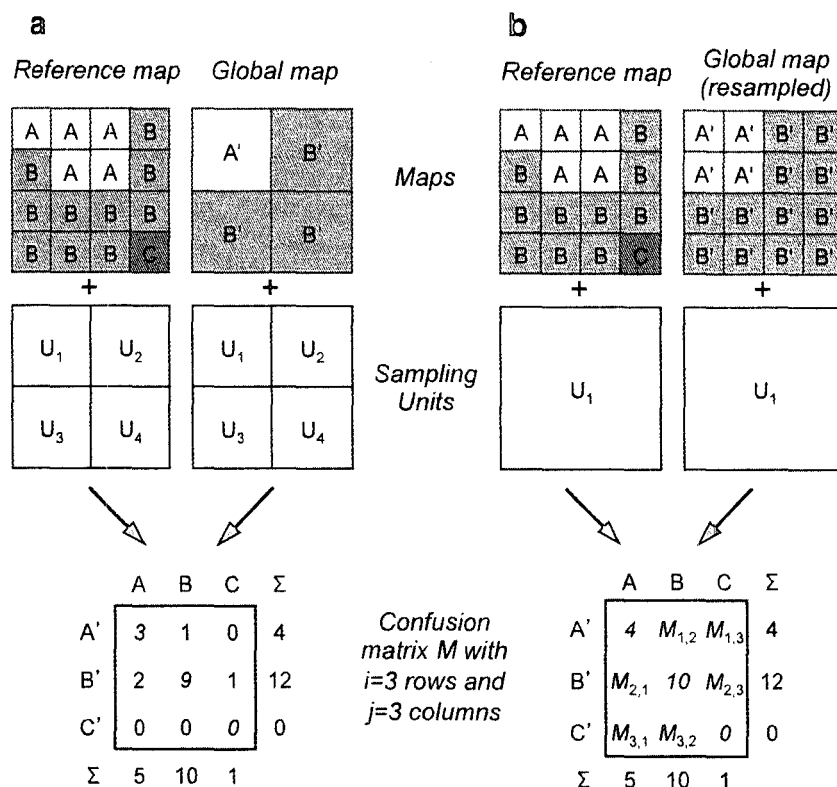
Fig. 2. Examples of constructing fractional error matrices for sampling units equal to a) the global map resolution and b) blocks of 2 \times 2 coarse resolution pixels. For pixel blocks, row and column totals must be computed from the map statistics.
