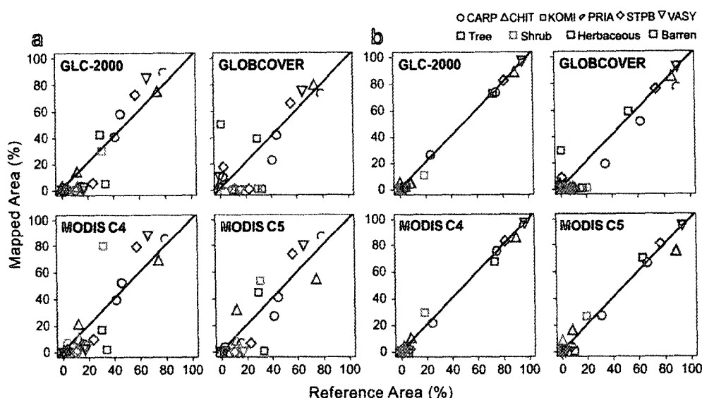
Fig. 7. Predicted (global map) versus reference land cover area, calculated from (a) all pixels and (b) pure pixels, in percent of total test site area for GLC-2000, GLOBCOVER, MODIS C4, and MODIS C5. Symbol shapes represent individual test sites. Symbol fill patterns and shades of gray represent individual LFT classes (tree: open light gray, shrub: filled light gray, herbaceous: open dark gray, barren: filled dark gray).
