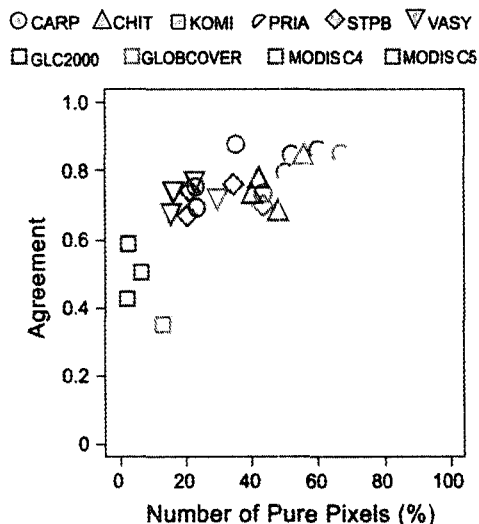
Fig. 9. Total agreement versus number of pure coarse resolution pixels at each site. Pure coarse pixels are defined to contain at least 95% of a single land cover class in the reference data. Symbol shapes represent individual test sites. Symbol fill patterns and shades of gray represent different global maps (GLC-2000: open light gray, GLOBCOVER: filled light gray, MODIS C4: open dark gray, MODIS C5: filled dark gray).
