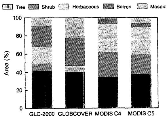
Fig. 3. Relative regional frequency of dominant life form types across Northern Eurasia based on global land cover maps.
