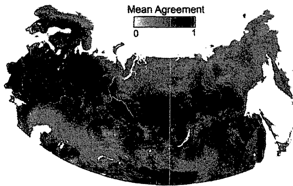
Fig. 5. Mean agreement of four land cover products (GLC-2000, GLOBCOVER, MODIS C4 and MODIS C5) after thematic aggregation to LFT legend (Table 1). Mean agreement is the average pairwise agreement between global maps and calculated as fractional agreement of land cover proportions within 3 \times 3 km blocks, e.g. a value of 0.8 means that on average 80% of the land cover in a pixel block is in agreement.
