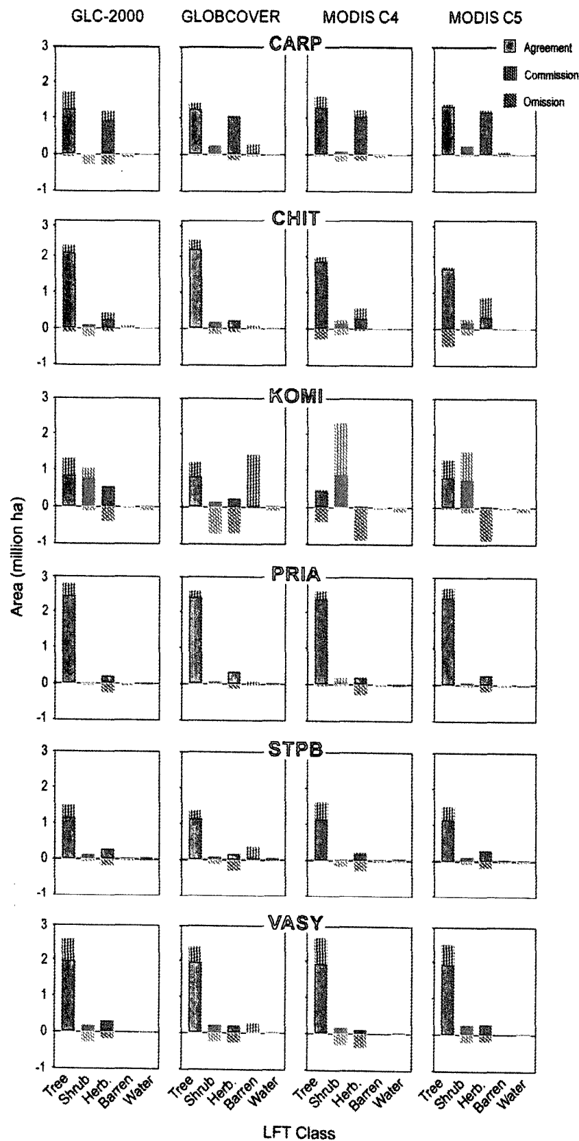
Fig. 8. Agreement, commission error, and omission error for LFT classes (tree: green, shrub: orange, herbaceous: magenta, barren: gray, water: blue) at six test sites (CARP, CHIT, KOMI, PRIA, STPB, and VASY) using 3 \times 3 km pixel blocks as sampling units. For illustration, omission error is represented by negative values, whereas agreement and commission error are represented by positive values.
