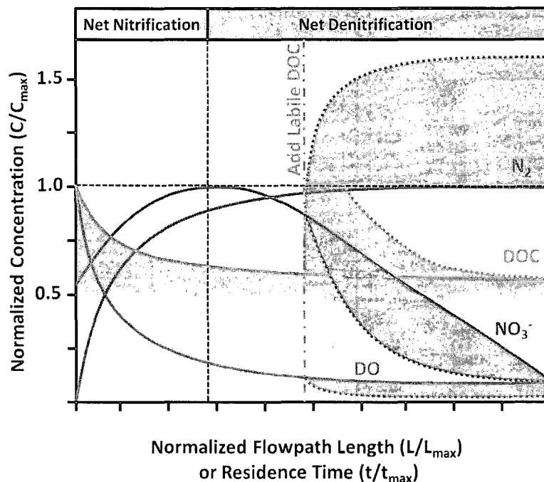
Figure 2. Steady state denitrification dynamics at the study site hyporheic zone (solid curves, modified from Zarnetske et al. [2011]) showing the hypothesized response of denitrification (dashed curves) to an addition of labile dissolved organic carbon (DOC). The shaded regions represent a net change in the abundance of a solute due to the addition of labile DOC. Note that the labile fraction of the total DOC is presented as the upper shaded region under the DOC curve with the remainder of the mass representing less bioavailable forms of DOC. Overall, we hypothesize that the addition of labile DOC to the hyporheic zone will significantly increase dinitrogen ( N_2 ) production, decrease total nitrate ( NO_3^- ) concentration and mass transported through the system, and facilitate additional dissolved oxygen (DO) consumption.
