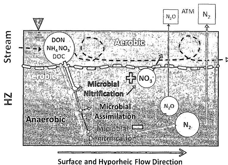
Figure 1. Illustration showing a simplified longitudinal cross-sectional view of a stream hyporheic (HZ) environment with commonly observed microbially mediated pathways for nitrate ( \text{NO}_3^- ) transformations. These pathways were observed in the present study's hyporheic system [Zarnetske et al., 2011]. Surface waters supply \text{NO}_3^- and dissolved organic nitrogen (DON) and carbon (DOC) to the hyporheic zone. In aerobic regions of the hyporheic zone, DON can be mineralized to \text{NH}_4^+ , which can be transformed via nitrification to create additional \text{NO}_3^- . The DOC and \text{NO}_3^- also can be retained in the hyporheic zone via microbial assimilation processes. DOC and \text{NO}_3^- entering anaerobic portions of the hyporheic zone can be utilized for denitrification, which produces dinitrogen oxide ( \text{N}_2\text{O} ) and dinitrogen ( \text{N}_2 ). The \text{N}_2\text{O} and \text{N}_2 can degas out of the stream system and return to the atmosphere (ATM).
