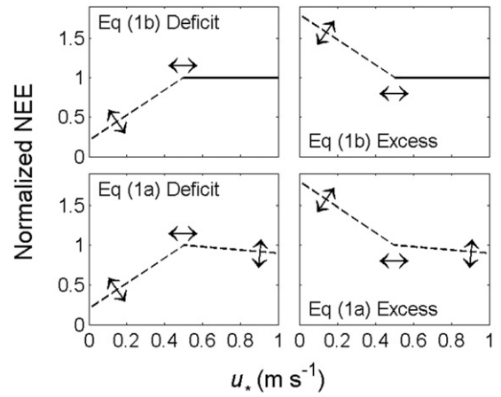
Fig. 1. Examples of the operational (Eq. (1b), upper panels) and diagnostic (Eq. (1a), lower panels) change-point models, in deficit mode (left panels) and excess mode (right panels). NEE has been normalized to one at the change point. The arrows indicate variation in model parameters.
