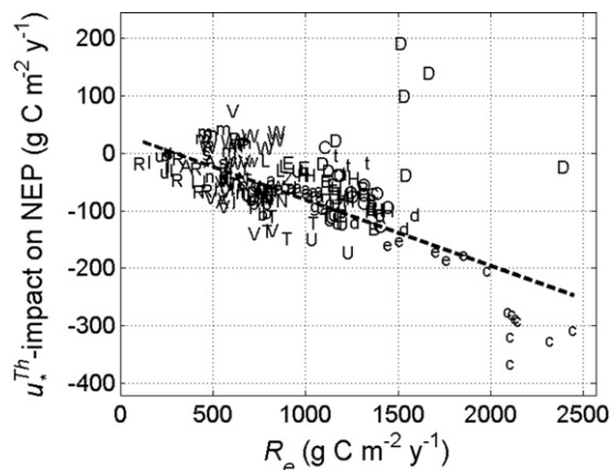
Fig. 5. Change in annual NEP ( \Delta \text{NEP} ) caused by the application of u^{\text{Th}} filter, in relation to annual R_e , by site-year. \Delta \text{NEP} is computed as the difference between annual NEP at the pooled median u^{\text{Th}} (modified method) and annual NEP calculated with no u^{\text{Th}} filter. Gaps in NEE were filled using the MDS method. Annual R_e was estimated using FCM gap-filling/partitioning. The linear regression relationship, applied to sites in deficit mode, is \Delta \text{NEP} = -0.11 \cdot R_e + 34 \text{ g C m}^{-2} \text{ y}^{-1} ( r^2 = 0.59 ).
