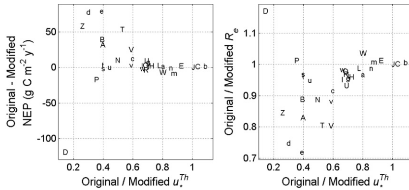
Fig. 6. Impact of modifications to the u_*^{Th} -evaluation method on mean annual NEP and R_e , by site, in relation to the ratio of the original and modified estimates of the u_*^{Th} . The left panel shows the difference between NEP estimated using the original u_*^{Th} and NEP estimated using the modified u_*^{Th} . The right panel shows the ratio of R_e estimated using the original u_*^{Th} to R_e estimated using the modified u_*^{Th} .
