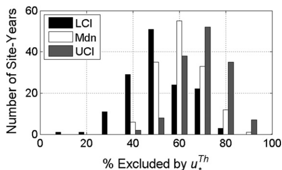
Fig. 11. Histogram of fractional data exclusion at the lower u^{*Th} 95% confidence interval (LCI), median u^{*Th} (Mdn), and upper u^{*Th} 95% confidence interval (UCI), as estimated by bootstrapping, for all site years.
