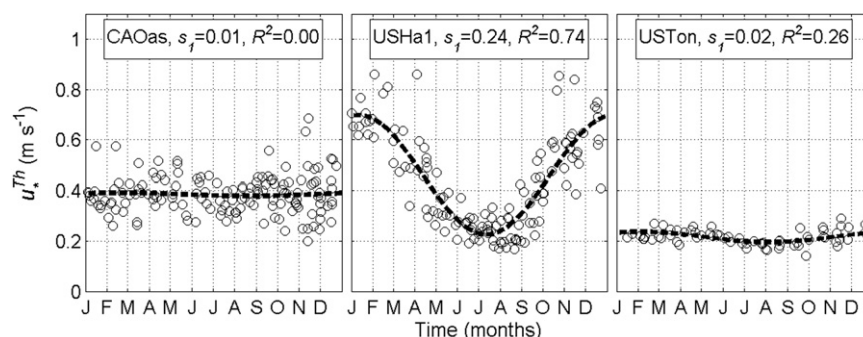
Fig. 8. Seasonal variation in the u_*^{Th} at three representative sites, estimated using temporal moving windows and with all years pooled. The dotted line is a fitted annual sine curve (Eq. (5)) with amplitude s_1 and coefficient of determination R^2 .
