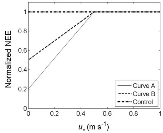
Fig. 2. Idealized ( u_* versus NEE) relationships used to evaluate u_*^{Th} detection methods. The control is a flat line with no u_*^{Th} .
