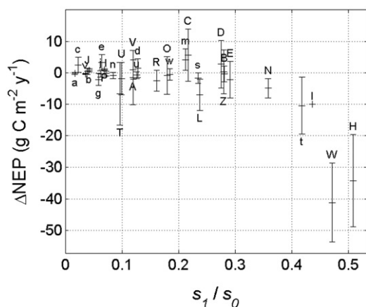
Fig. 9. Impact of seasonal variation in the u_*^{Th} on annual NEP (computed as the difference between annual NEP using a seasonally-varying u_*^{Th} filter and annual NEP at the median annual u_*^{Th} ), as a function of the s_1/s_0 ratio from Eq. (5). Gaps in NEP were filled using the MDS method. The error bars show one s.d. from the mean.
