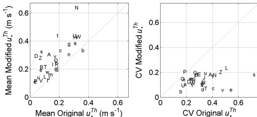
Fig. 4. Comparison of u^{*Th} estimates from the original (Papale et al., 2006) and modified methods, by site. Left panel: annual means; right panel: mean annual coefficient of variation.
