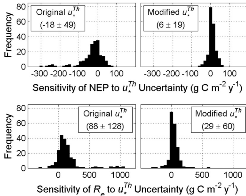
Fig. 7. Upper panels: Histograms for all site-years showing the sensitivity of annual NEP to uncertainty in the u_*^{Th} , computed as the difference between annual NEP at the 97.5 and 2.5 u_*^{Th} percentiles, for the original (left panel) and modified (right panel) u_*^{Th} methods. Gaps were filled using the MDS method. The bracketed numbers in the text boxes are the median \pm inter-quartile range, in ( \text{g C m}^{-2} \text{ y}^{-1} ). Lower panels: Same as upper panels but for annual R_e estimated using FCM gap-filling and partitioning.
