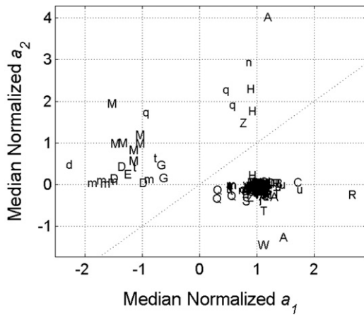
Fig. 3. Normalized parameters a_1 and a_2 from the diagnostic change-point model (Eq. (1a)), computed as annual medians from the most frequent mode (deficit or excess), and plotted annually by site code (Table 1). The values of a_1 and a_2 are normalized to an NEE value of one at u^* = u^{*Th} , by multiplying each by a factor of [u^{*Th}/(a_0 + a_1 \cdot u^{*Th})] .
