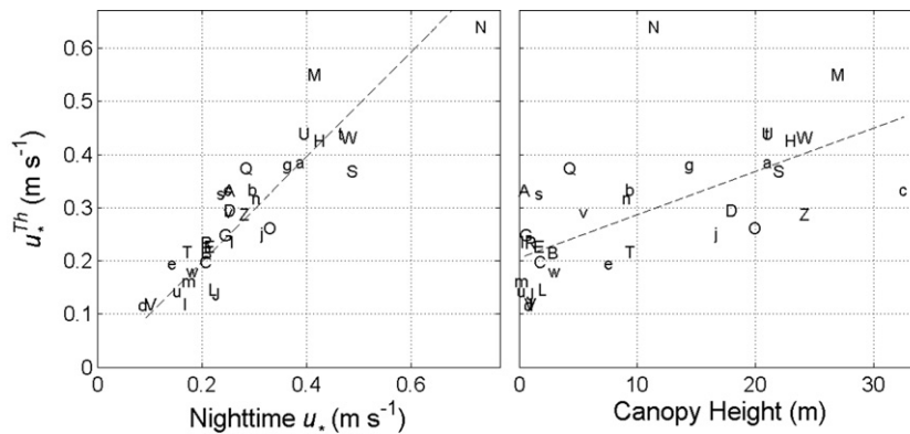
Fig. 10. Dependence of mean annual u_*^{Th} on mean annual nighttime u_* (left panel) and canopy height (right panel) across all sites. The linear regression fits are: u_*^{Th} = 0.988 u_* , r^2 = 0.79 (forced through origin, y intercept not significantly different from zero), and u_*^{Th} = 0.205 \text{ m s}^{-1} + 0.0081 h_c ( h_c in m) ( r^2 = 0.42 ).
