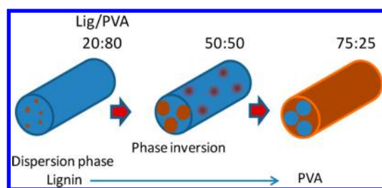
Figure 8. Schematic representation of proposed surface composition of composite electrospun lignin/PVA fibers. The exact distributions, size, and number of domains are unknown.
