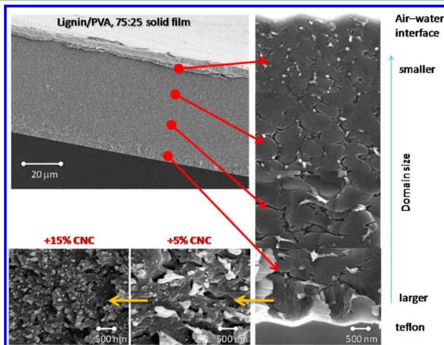
Figure 7. SEM images of cross sections of lignin/PVA (75:25) films. The two interfaces indicated correspond to the air/film interface and film/Teflon support. The size of the domains is reduced as they are closer to the air/film interface. The addition of CNC to the aqueous dispersion used as precursor of the films is observed to reduce the characteristic size of the phase-separated domains (see images in bottom panels with cross sections of films loaded with 5 and 15% CNCs).
