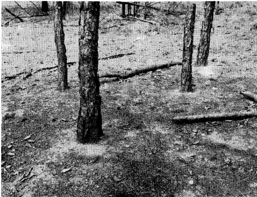
Figure 8.--Fire removes the protective litter from the ground at the base of trees. Stemflow water then frequently becomes surface runoff as shown above, where the soil in a ring around the trees has been washed free of charcoal and is packed and bare.
