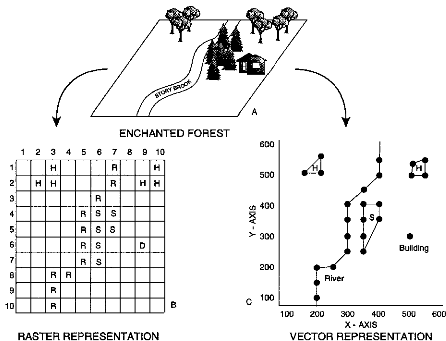
Figure 3—Comparison of vector and raster GIS models (modified from Aronoff 1989). A portion of the Enchanted Forest (A) is shown in raster representation (B) and in vector representation (C). The softwood (S) and hardwood (H) stands are area features. The Story Brook River (R) is a line feature, and the building representing district headquarters (D) is a point feature.
