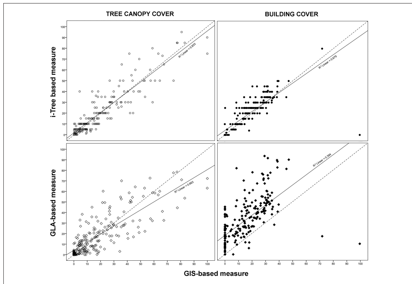
Figure 3. Comparison of field-taken tree canopy and building cover measures with the GIS-based measure. Dashed lines represent a perfect 1:1 correspondence of the two measures; solid line is the actual fit of the data.
