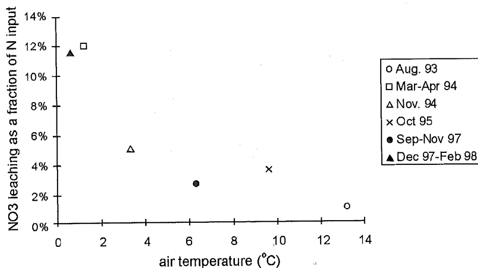
Figure 4-20. Observed relationship between \text{NO}_3^- leaching loss in runoff and mean air temperature at an experimental watershed site at Gårdsjön, Sweden. Each point represents an average of data collected over a period of 14 to 90 days. (Source: Moldan and Wright 1998.)
