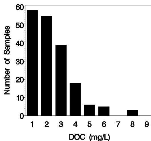
Figure 4-4. Patterns in DOC concentration in streams within a particular region. The data are not normally distributed; rather, they are skewed towards lower concentrations ( \leq 3 mg/L).
