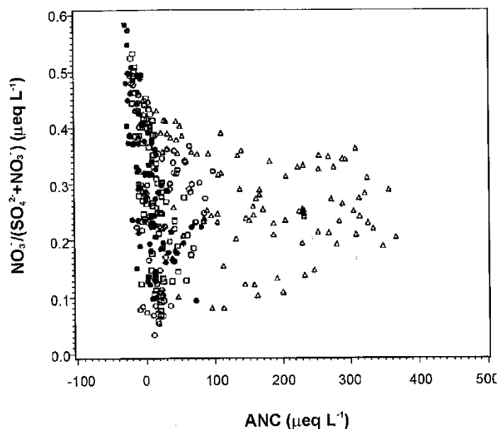
Figure 4-10. Ratio of \text{NO}_3^-:(\text{SO}_4^{2-} + \text{NO}_3^-) concentration versus ANC in stream water samples collected during hydrological episodes in four streams included in the Adirondack region of EPA's Episodic Response Program. The different symbols on the graph represent different streams. (Source: Sullivan et al. 1997.)
