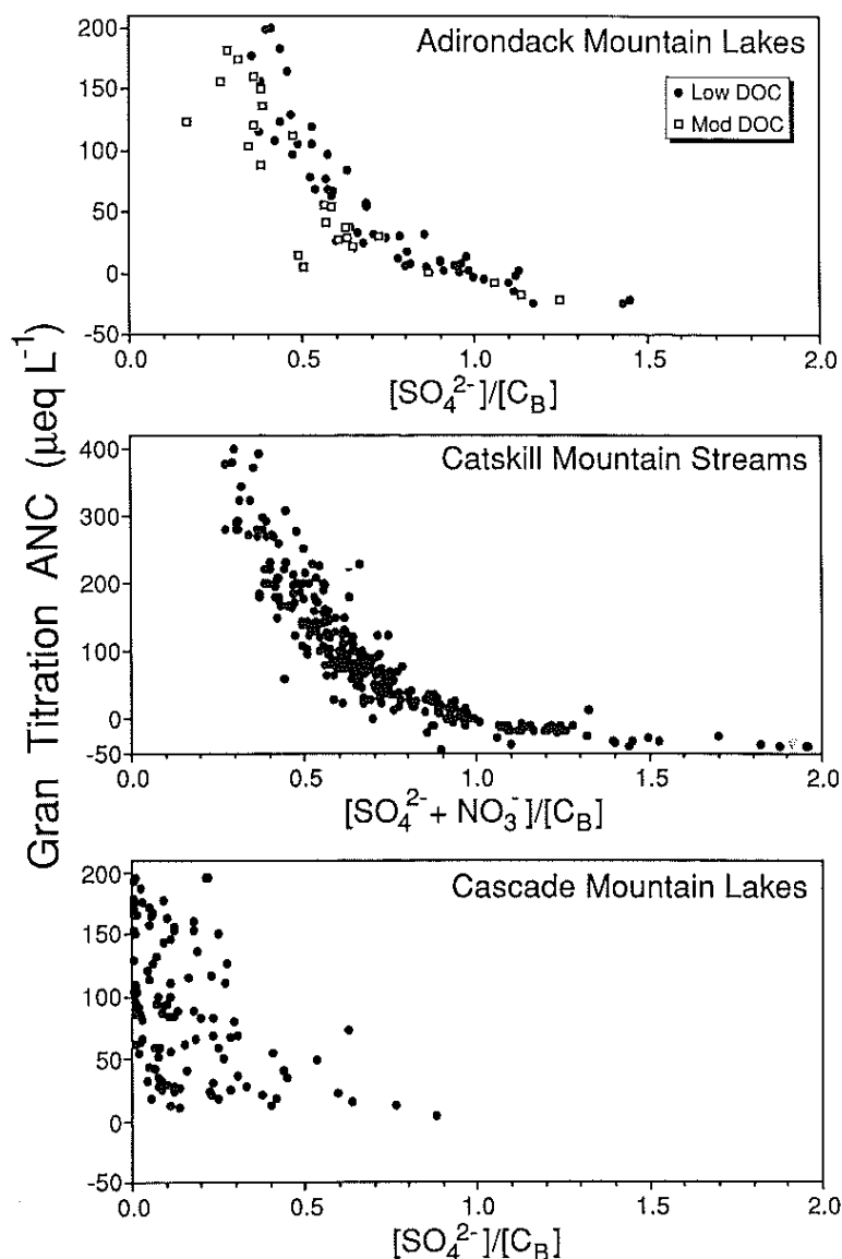
Figure 4-17. Plot of ANC versus ion ratio of \text{SO}_4^{2-} concentration divided by the sum of base cation concentrations (SBC) for low ANC ( \leq 200 µeq/L) surface waters in (a) Adirondacks, (b) Catskill Mountains, and (c) Cascade Mountains. The base cation sum includes \text{Ca}^{2+} + \text{Mg}^{2+} + \text{Na}^+ + \text{K}^+ . This plot reveals that surface water ANC is strongly related to the ratio \text{SO}_4^{2-}/\text{SBC} in the Adirondack region, and the ratio (\text{SO}_4^{2-} + \text{NO}_3^-)/\text{SBC} in the Catskill region, but weakly related to the ratio \text{SO}_4^{2-}/\text{SBC} in the Cascade Mountains region. Such an analysis sheds light on factors controlling surface water ANC. (Source: Sullivan 1990.)
